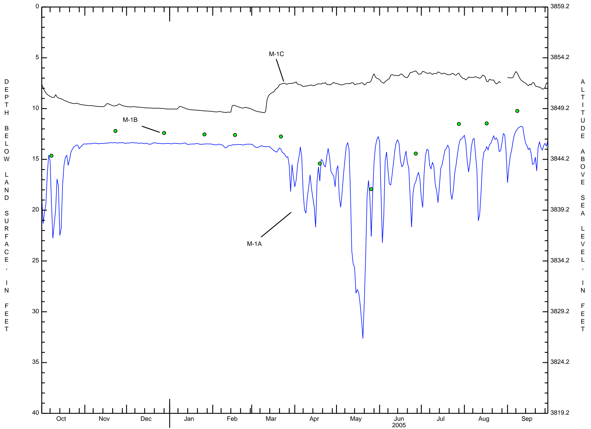
Mean daily water levels and miscellaneous water levels in well group M-1, 2005 water year.
