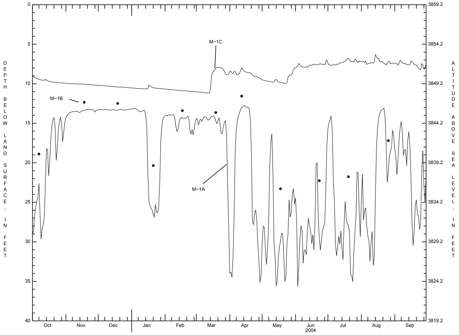
Mean daily water levels and miscellaneous water levels in well group M-1, 2004 water year.
