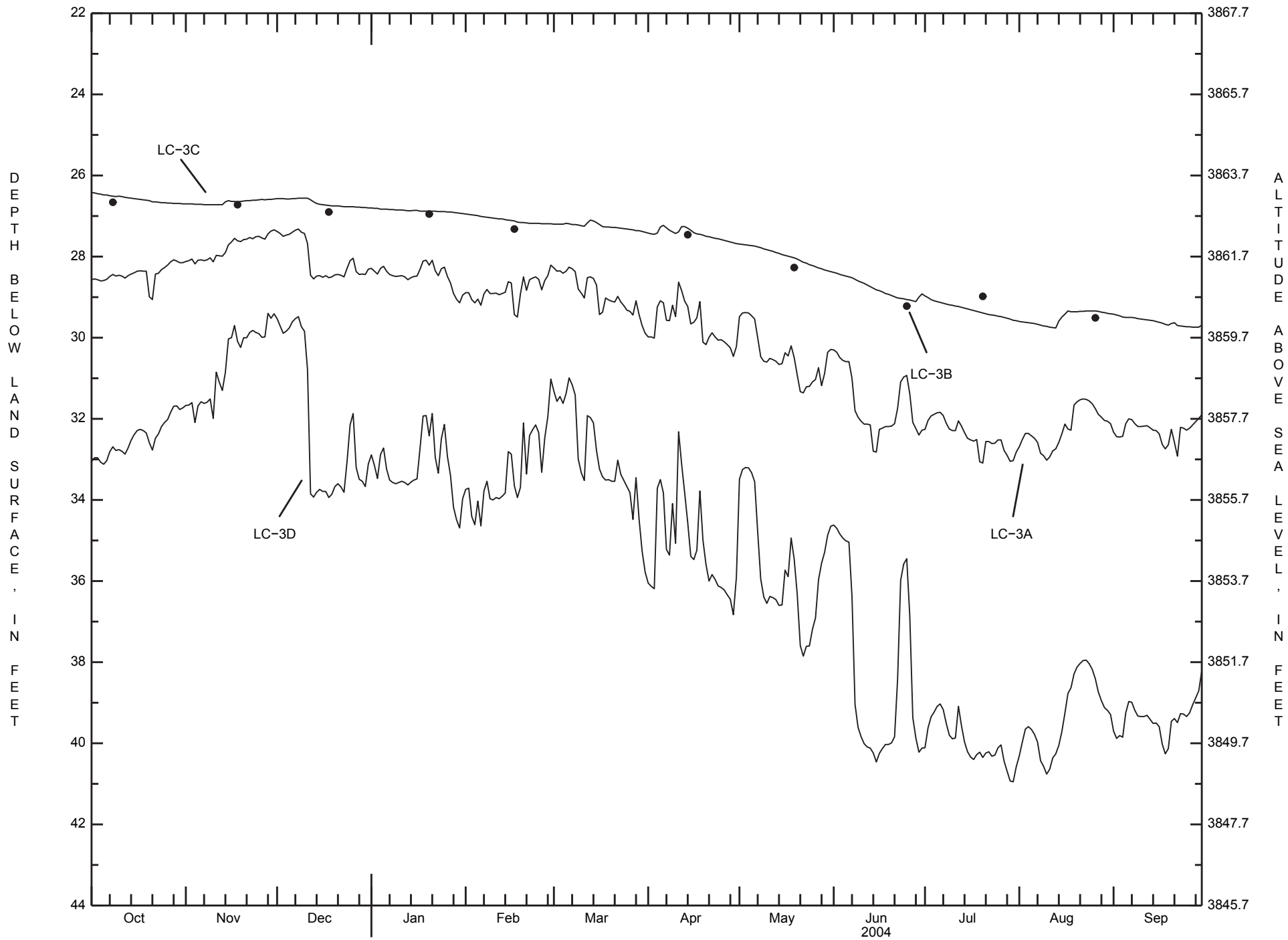
Mean daily water levels and miscellaneous water levels in well group LC-3, 2004 water year.
