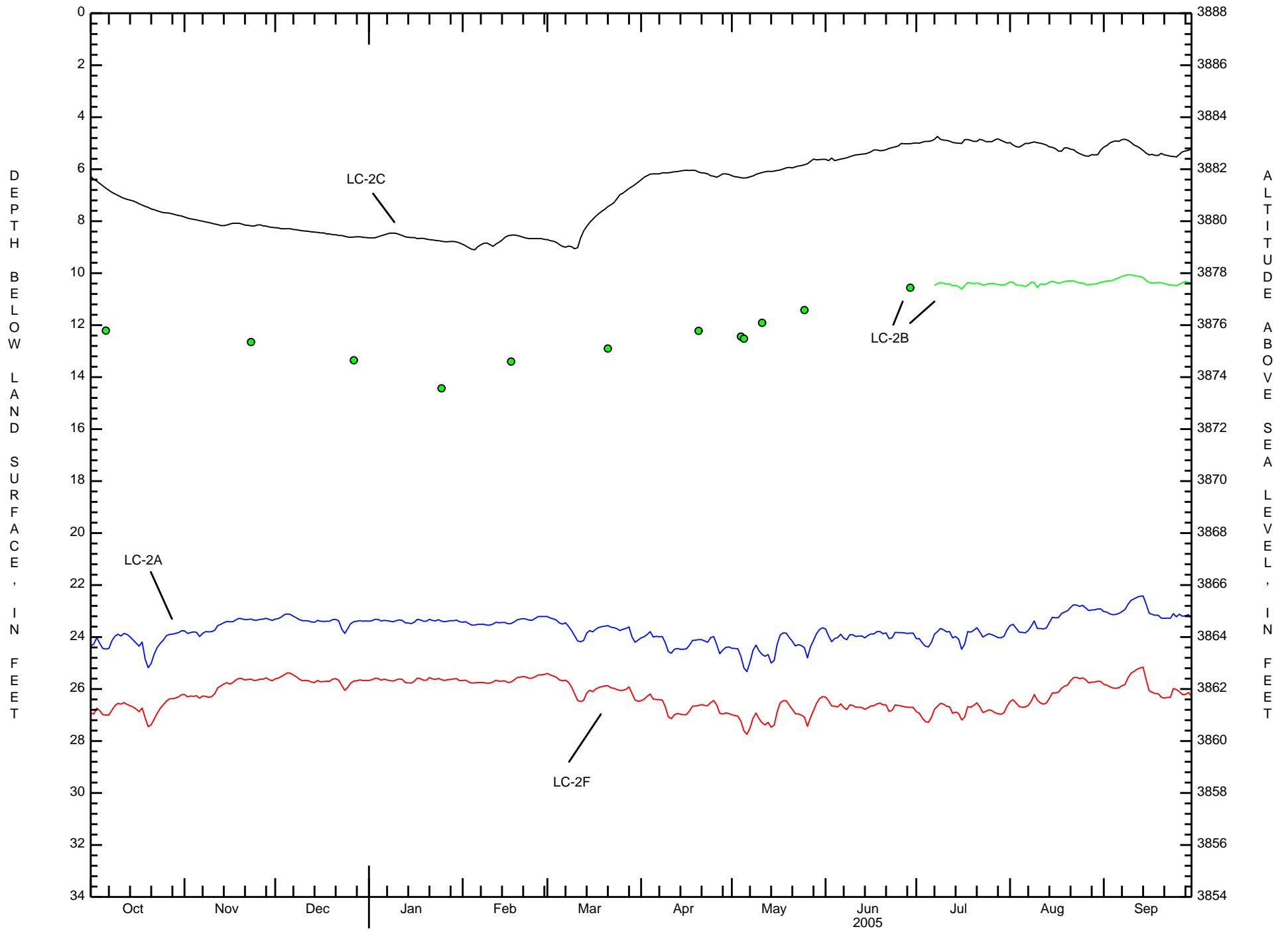
Mean daily water levels and miscellaneous water levels in well group LC-2, 2005 water year.
