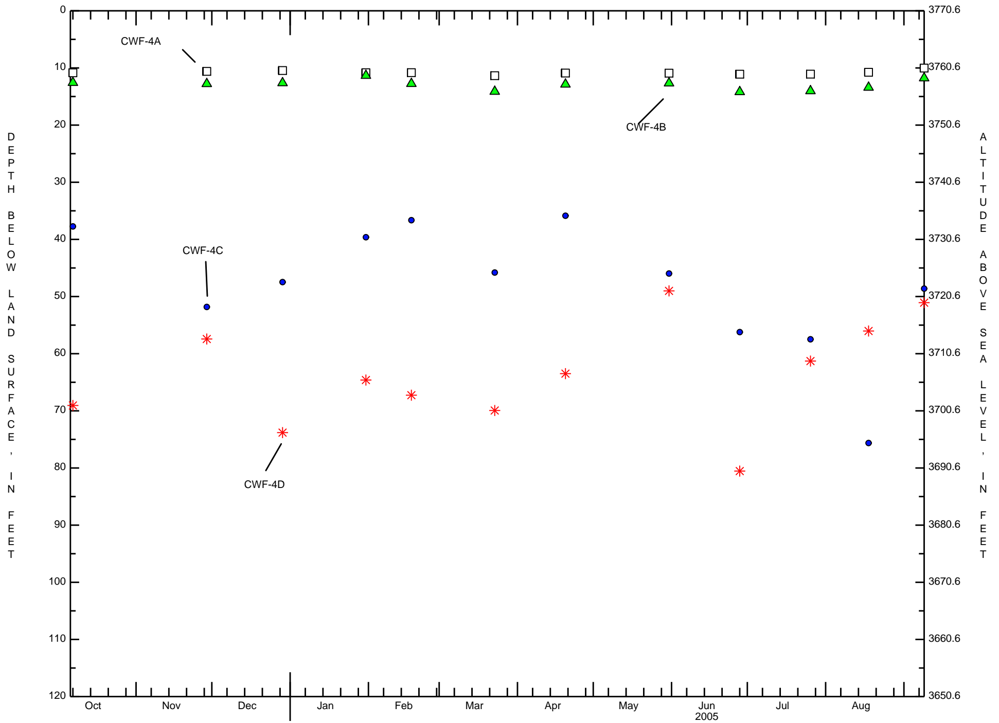
Miscellaneous water levels in well group CWF-4, 2005 water year.
