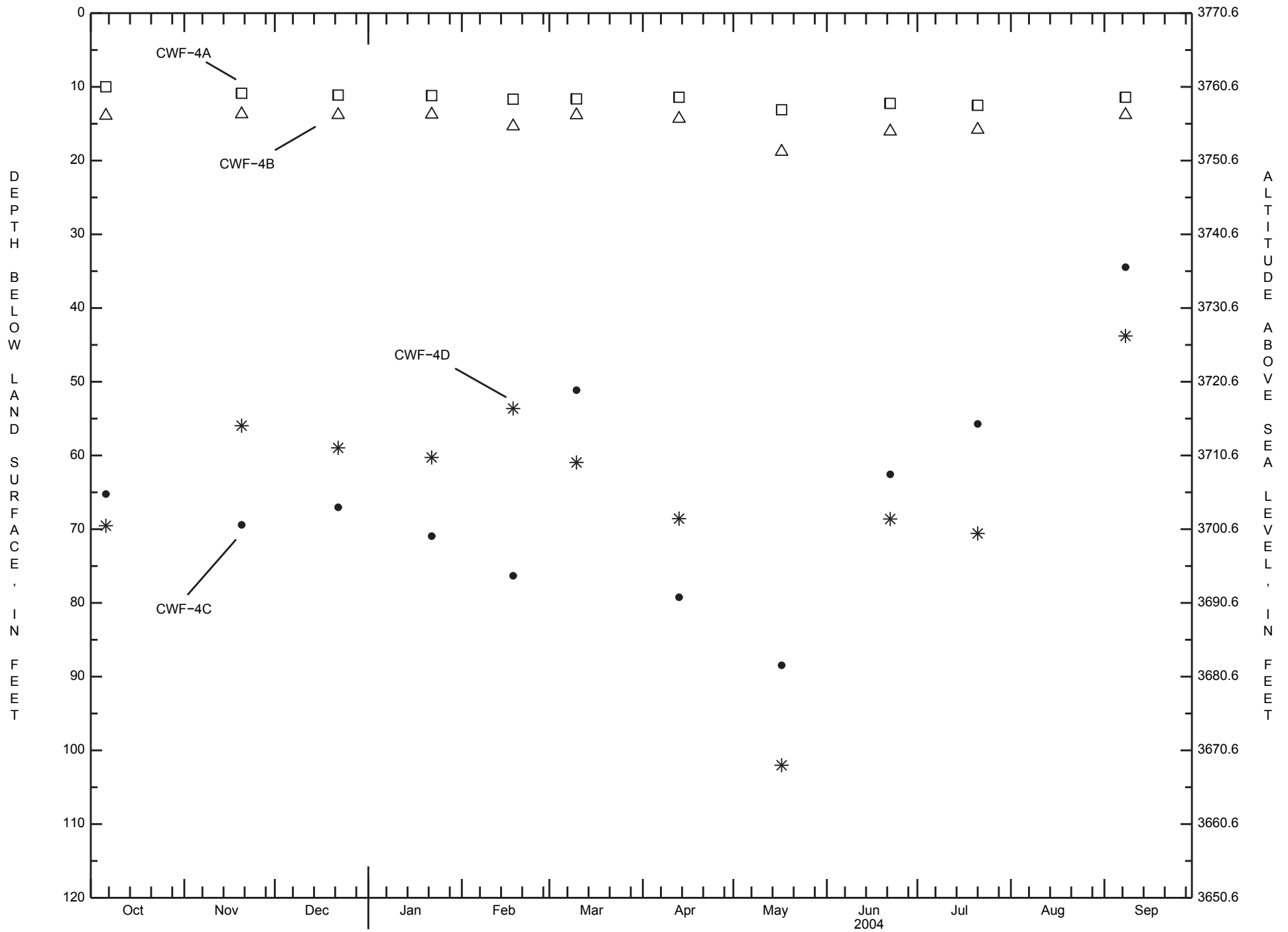
Miscellaneous water levels in well group CWF-4, 2004 water year.
