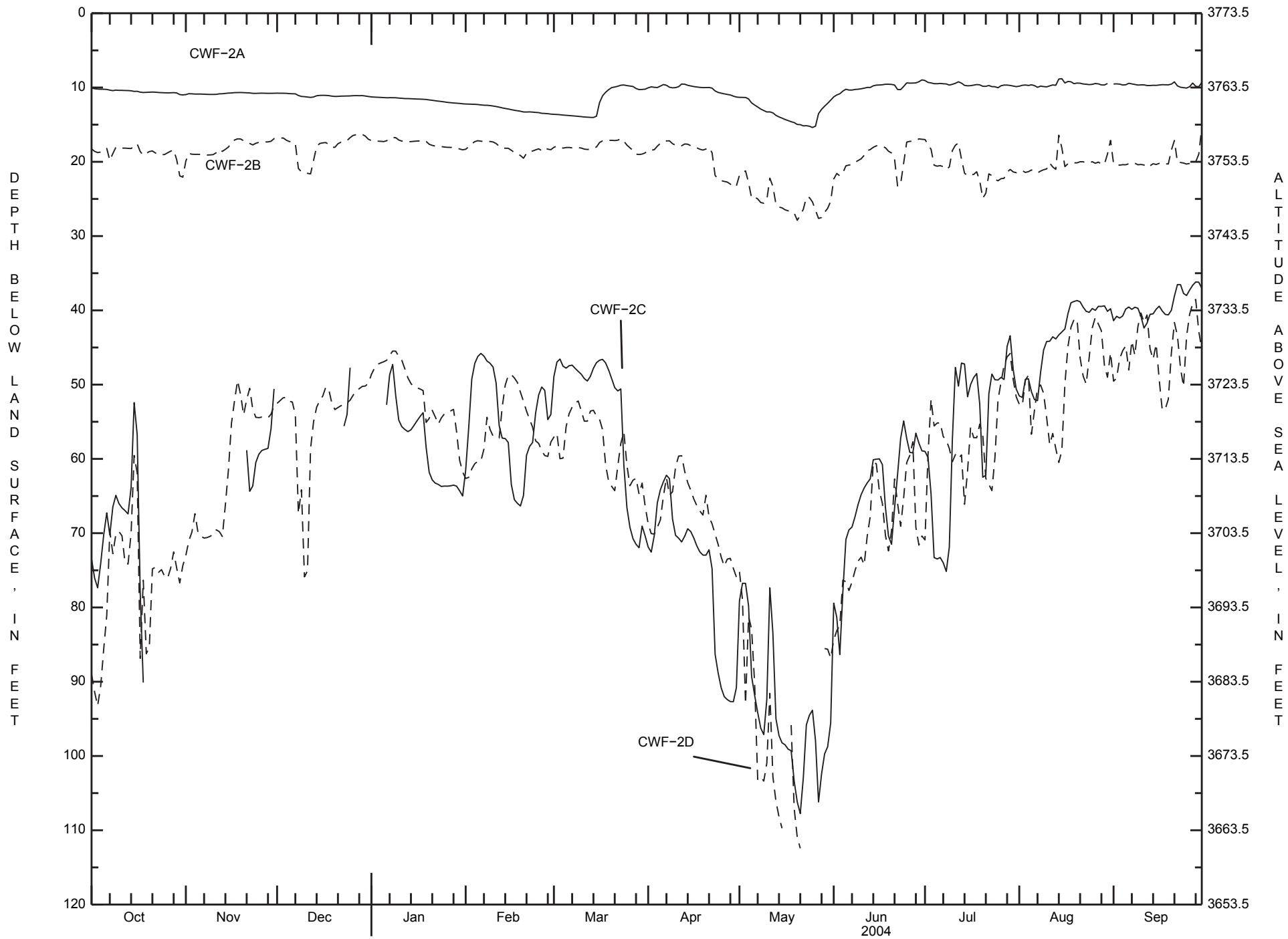
Mean daily water levels in well group CWF-2, 2004 water year.
