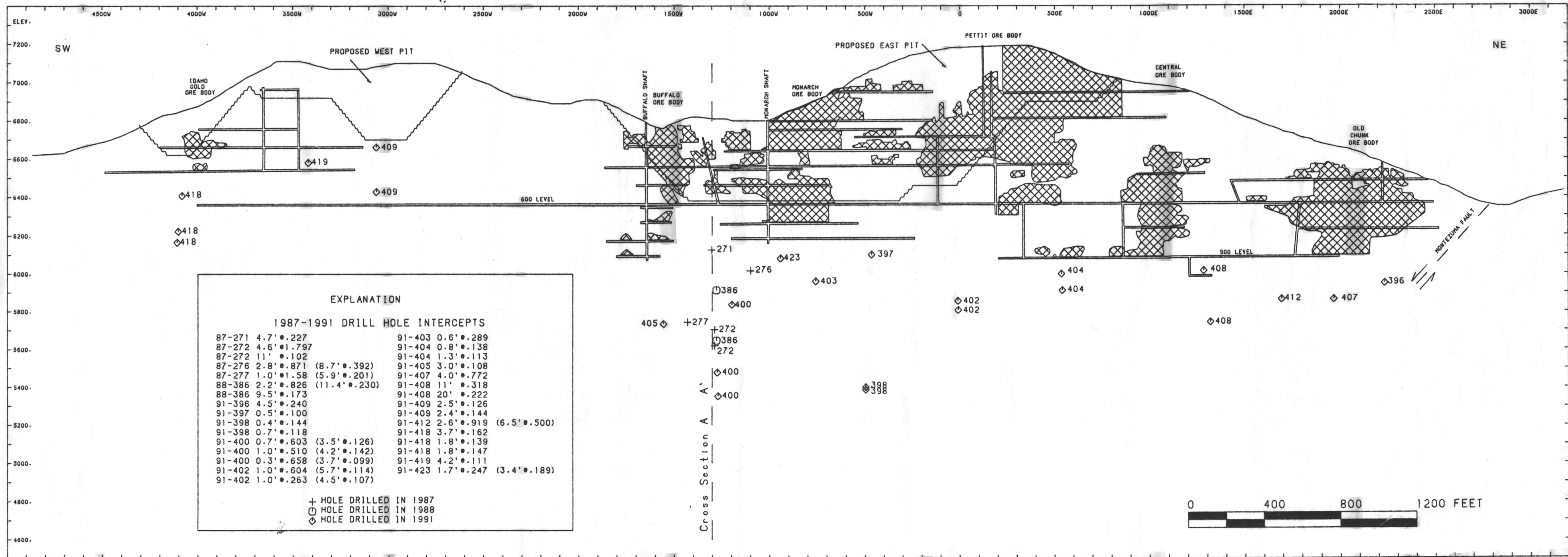
Plate 3. Longitudinal section B-B', along Base Line (pl. 2), looking northwest at Atlanta lode. Checked pattern marks former stopes, the parallel lines former mine levels, raises, and shafts (modified from Anderson (1939) and unpublished maps of Talache Mines, Inc.). Drill hole intercepts below old workings show (by symbol) year hole was drilled and abbreviated hole number. Intercept table shows year hole was drilled, complete hole number, true width of sampled material, and gold values in oz per ton. Tabular data in parentheses represent composite samples. Only holes with intercepts containing assay values of 0.10 oz Au per ton or more are shown.
