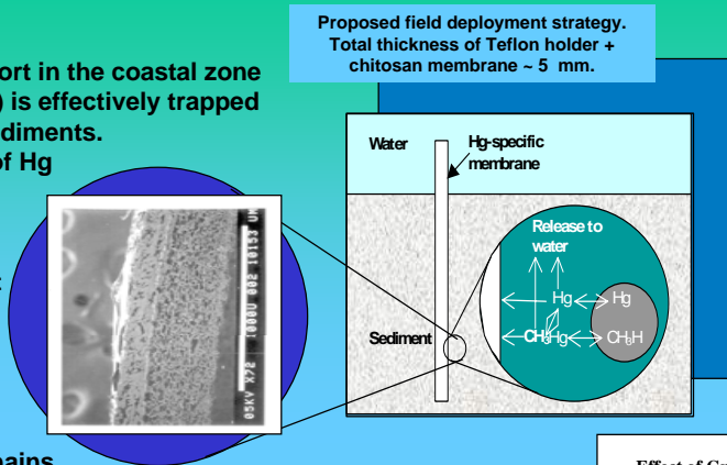
Cross-sectional view of scaffold reinforced chitosan membrane. Scale bar = 1 mm.
