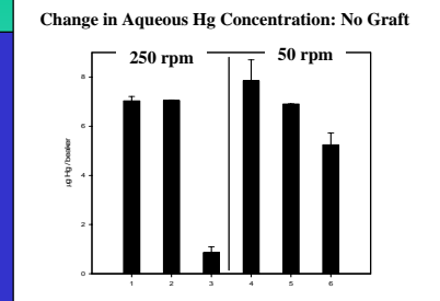
Treatments 1 & 4 = time 0; Treatments 2 & 5 = time 6 hrs for controls containing Teflon holders w/o membranes; Treatments 3 & 6 = time 6 hrs for Teflon holders w/ chitosan membranes.
