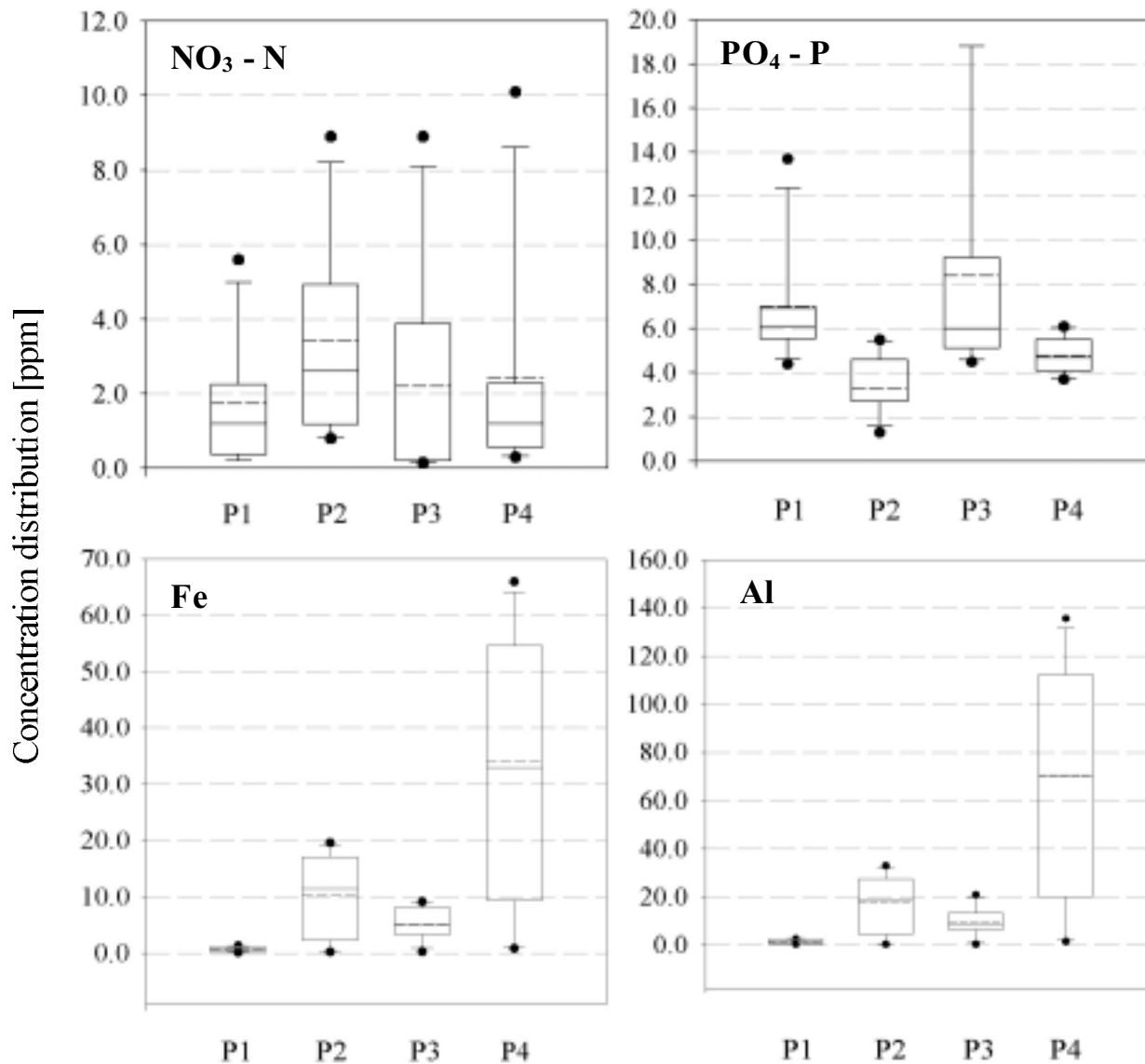
Fig. 1. Distribution of concentrations of NO 3 -N, PO 4 -P, Fe and Al in ppm (mg liter -1 ) from seven runoff events, following start of paratillage. Each box shows the 25 th percentile, median, and 75 th percentile. Whiskers show the 10 th and 90 th percentiles. Outliers beyond these limits are shown as dots. Means are shown as dotted lines inside boxes.
