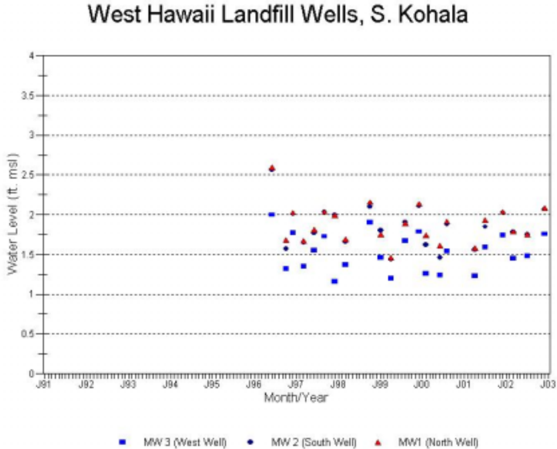
Figure 20. Water levels at the West Hawaii Landfill monitor wells.
