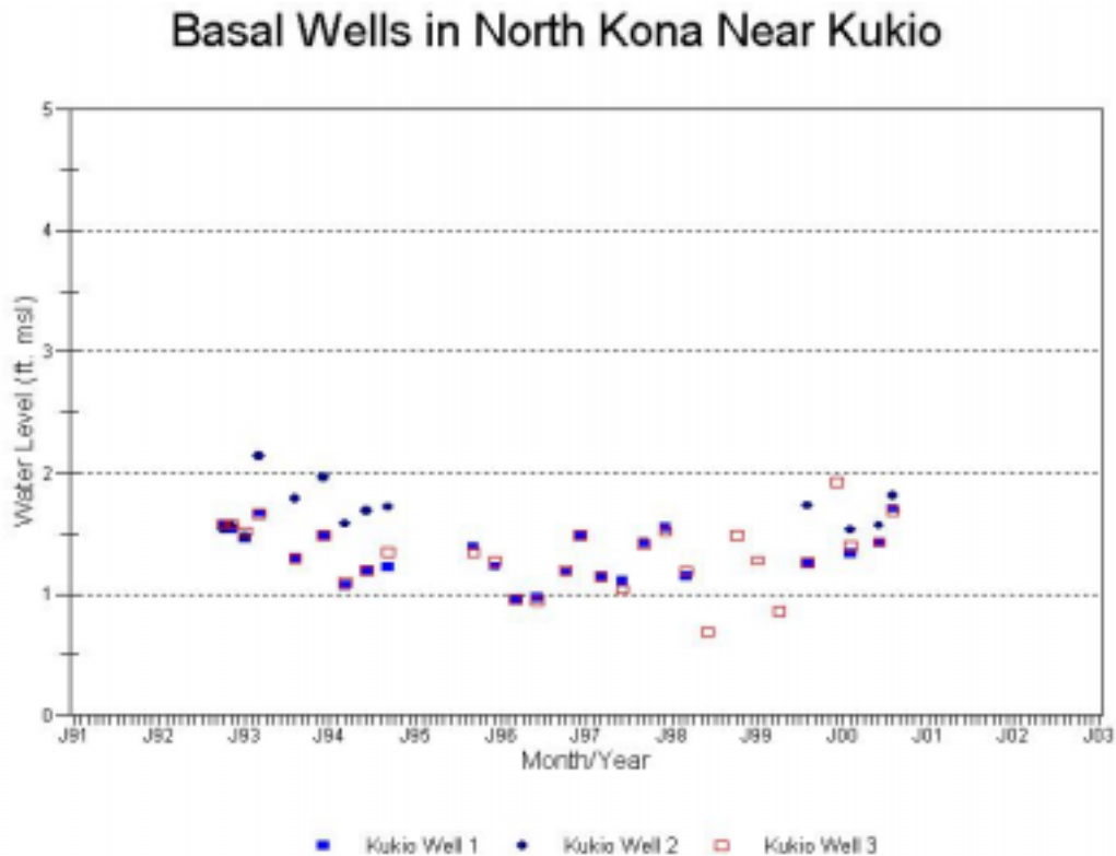
Figure 14. Water levels in the Kukio Irr. Wells.
