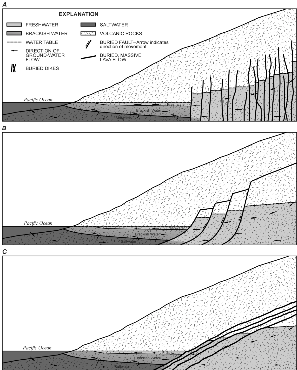
Figure 3. Three possible geologic structures that could impound high-level water.
