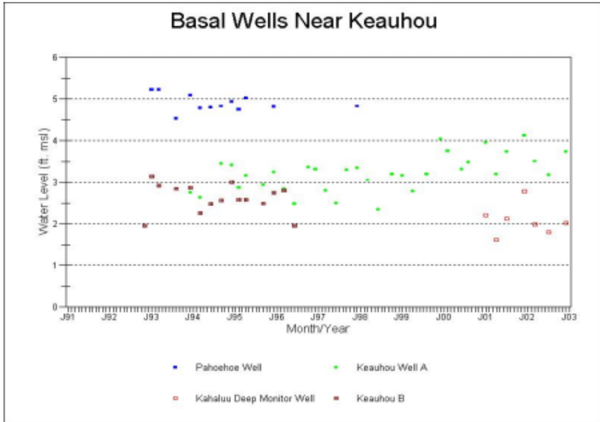
Figure 5. Basal wells in the Keauhou region.
