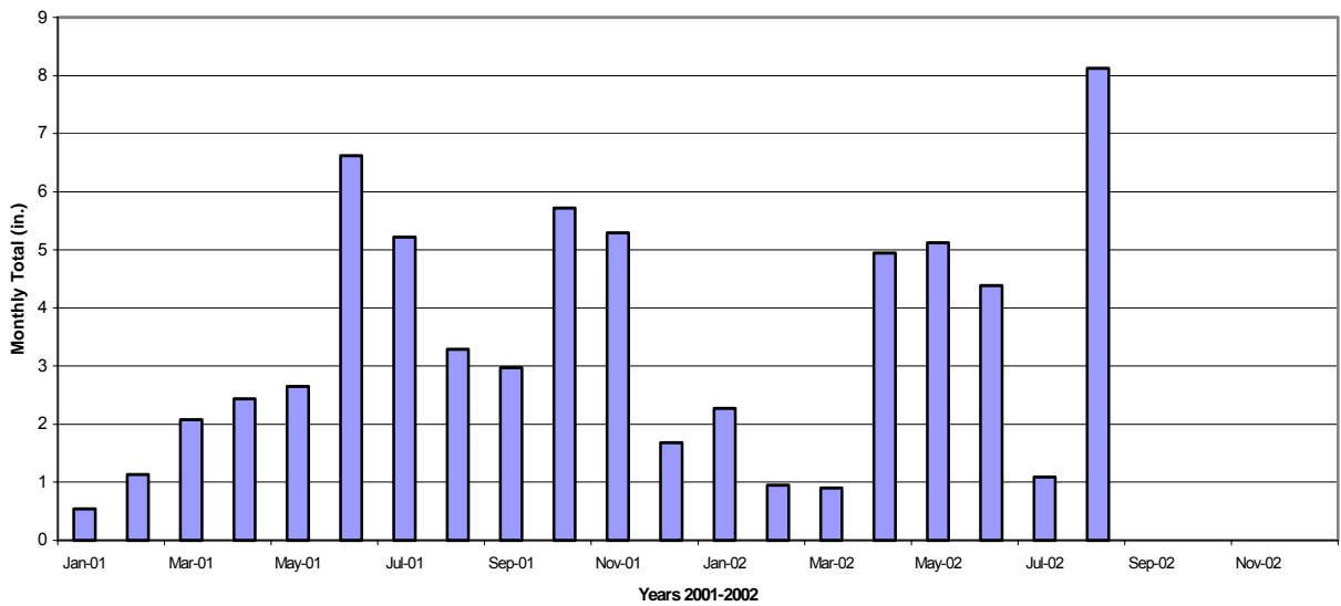
Figure 7. Monthly total rainfall for 2001-2002 at Lanikai Rain Gage 515330.
