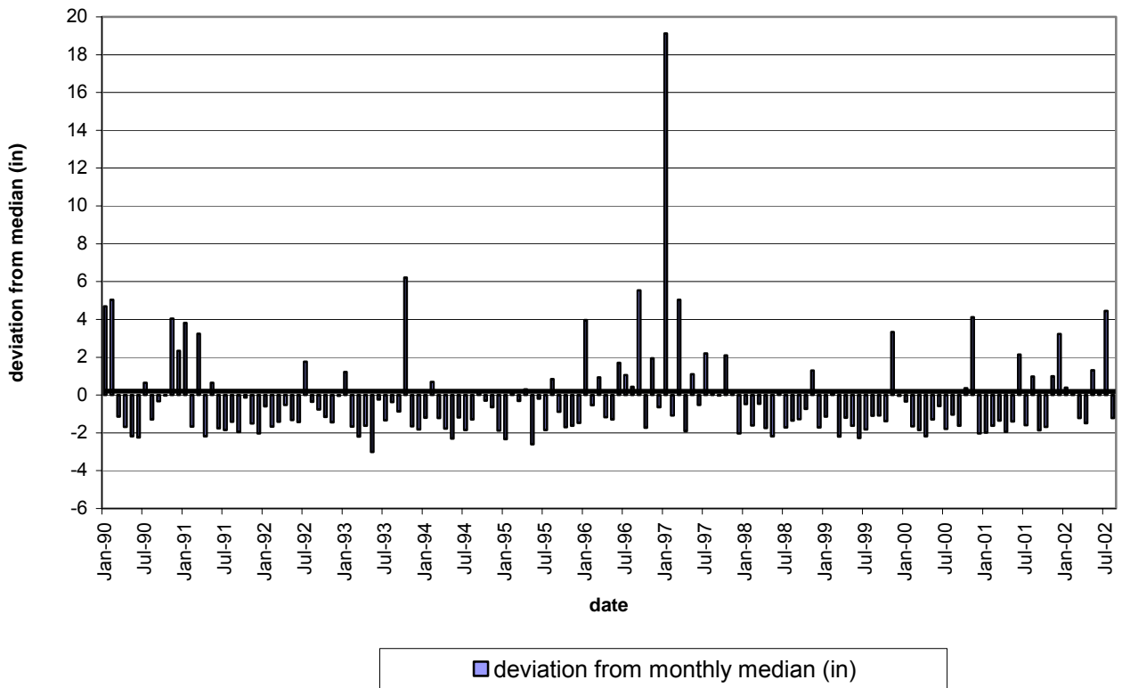
Figure 15. Departure of monthly median rainfall at the Huehue Station Gage 92.1.
