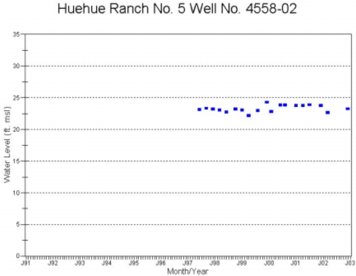
Figure 29. Water levels in Huehue Ranch 5.
