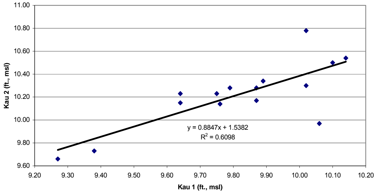
Figure 12. Correlation of water levels in the Kau wells.
