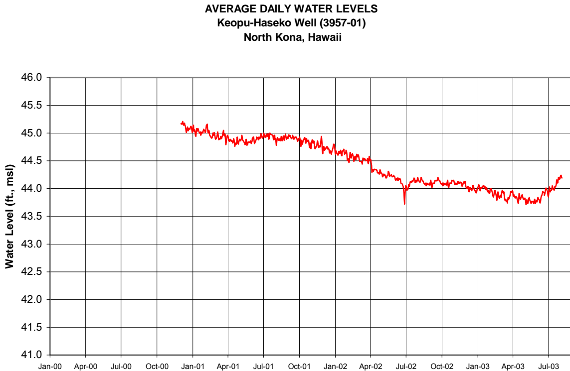
Figure 28. Average daily water levels in Keopu-Haseko well (from Daniel Lum, Water Resource Associates).
