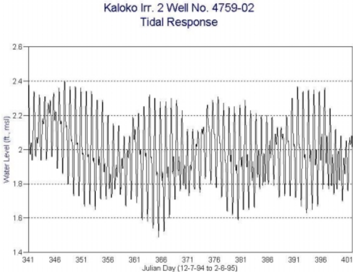
Figure 9. Tidal response in Kaloko Irr. 2 well no. 4759-02.
