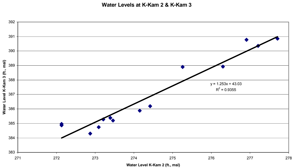
Figure 25. Water Level correlation between Keauhou-Kam 3 and Keauhou-Kam 2.
