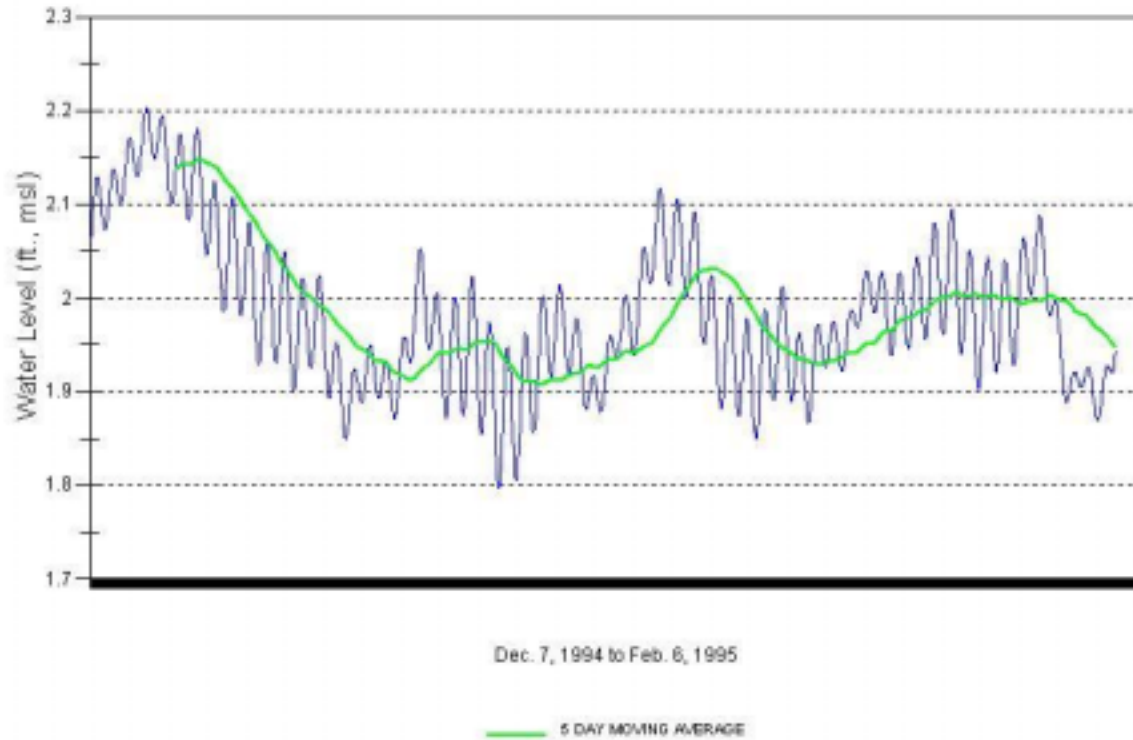
Figure 10. Tidal response removed and water levels smoothed.
