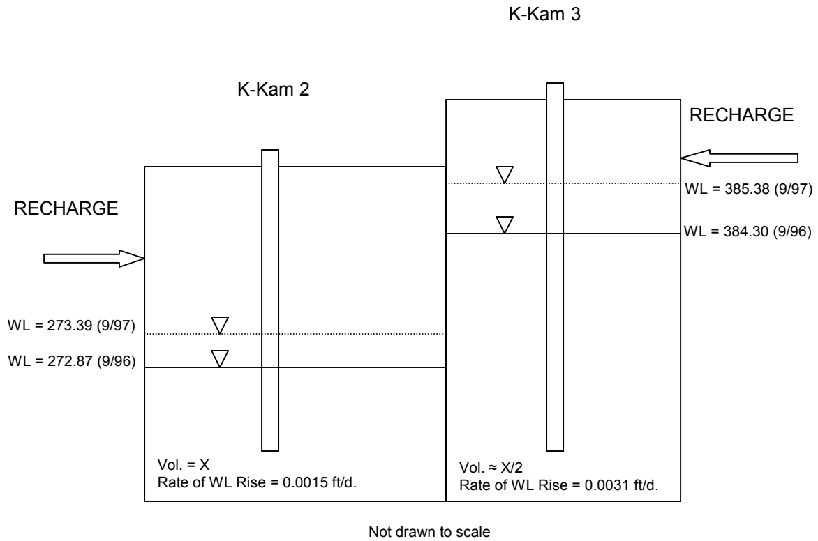
Figure 24. Conceptual model illustrating ground-water recharge into the high-level aquifers.
