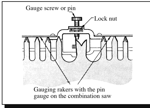
Figure 22—Gauging rakers.
