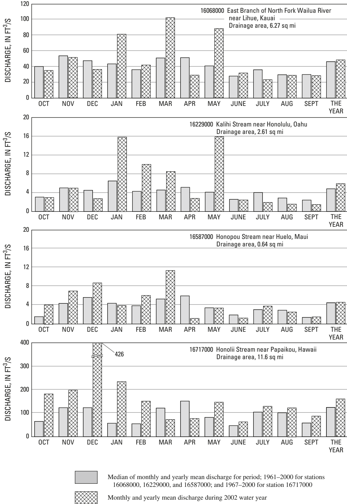
Figure 1. Discharge during 2002 water year compared with median discharge for four representative gaging stations.
