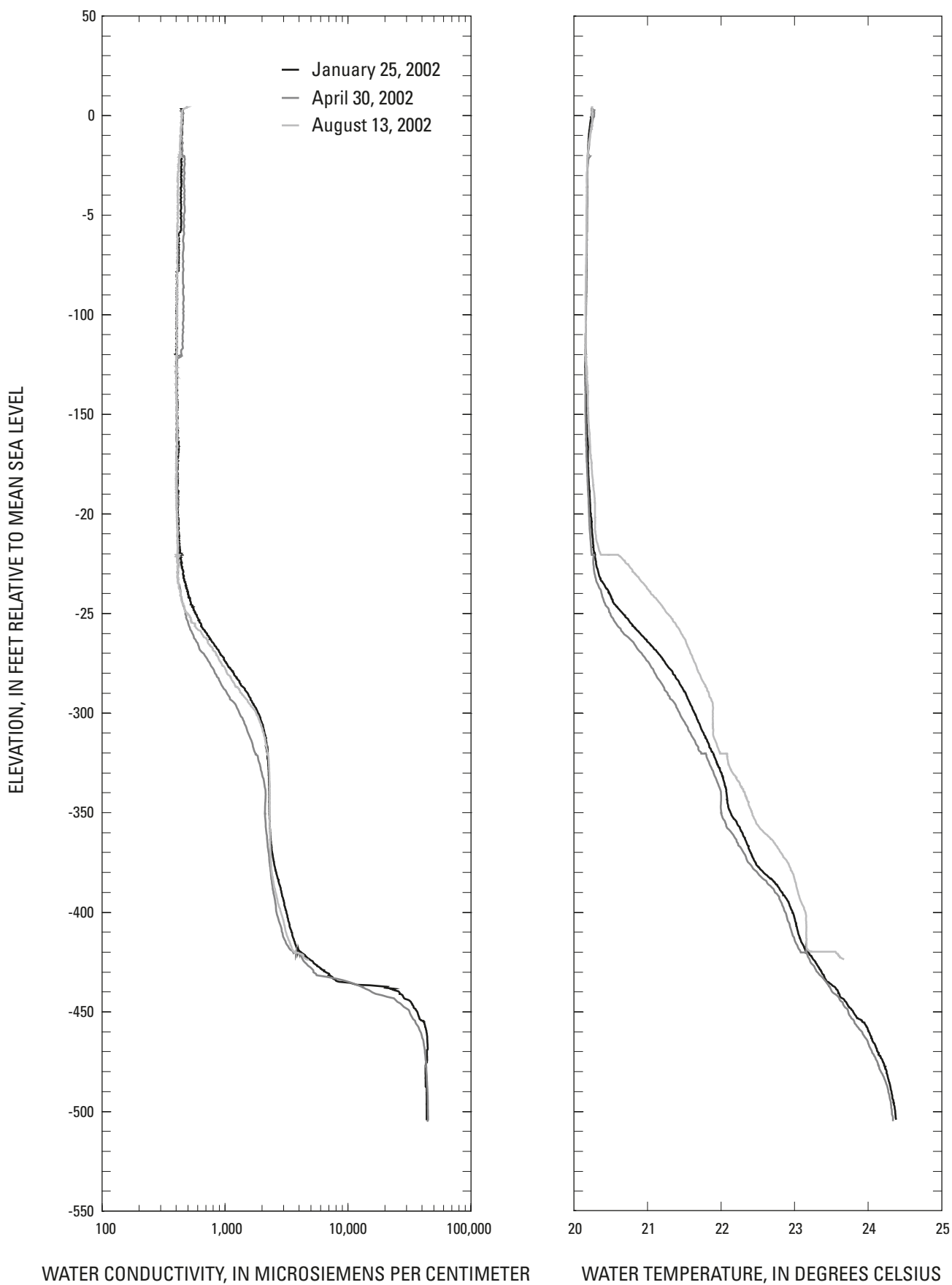
Water-conductivity and -temperature profiles measured in the Kualapuu deep monitor well (4-0800-01) on January 25, April 30, August 13 2002, Molokai, Hawaii. Data available from USGS Hawaii District log archive.
