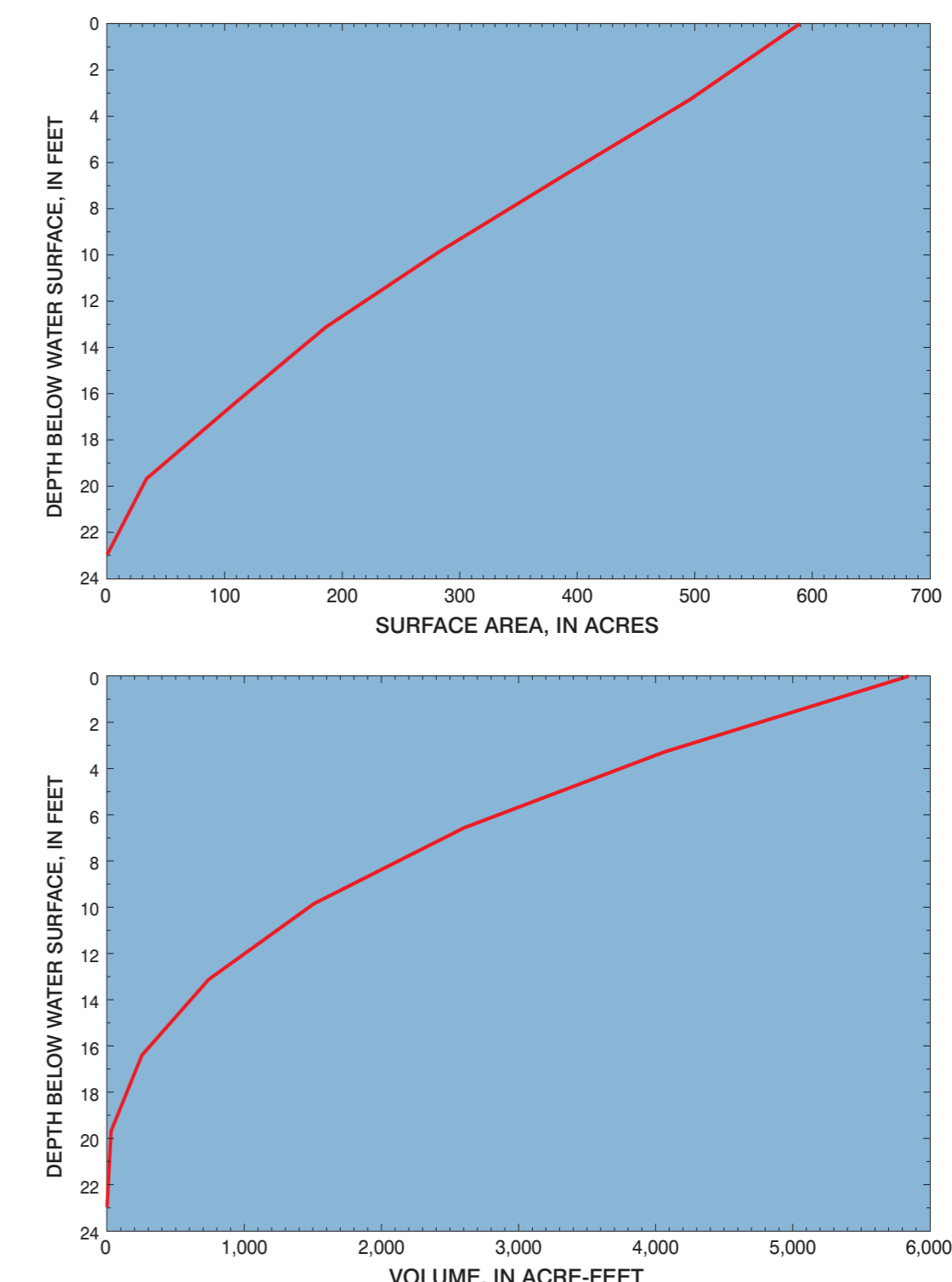
Figure 2. Depth-surface area and depth-volume relations for Black Bayou Reservoir. Water-surface elevation was 183.6 feet above sea level during the bathymetric survey of October 7-8, 1997.
