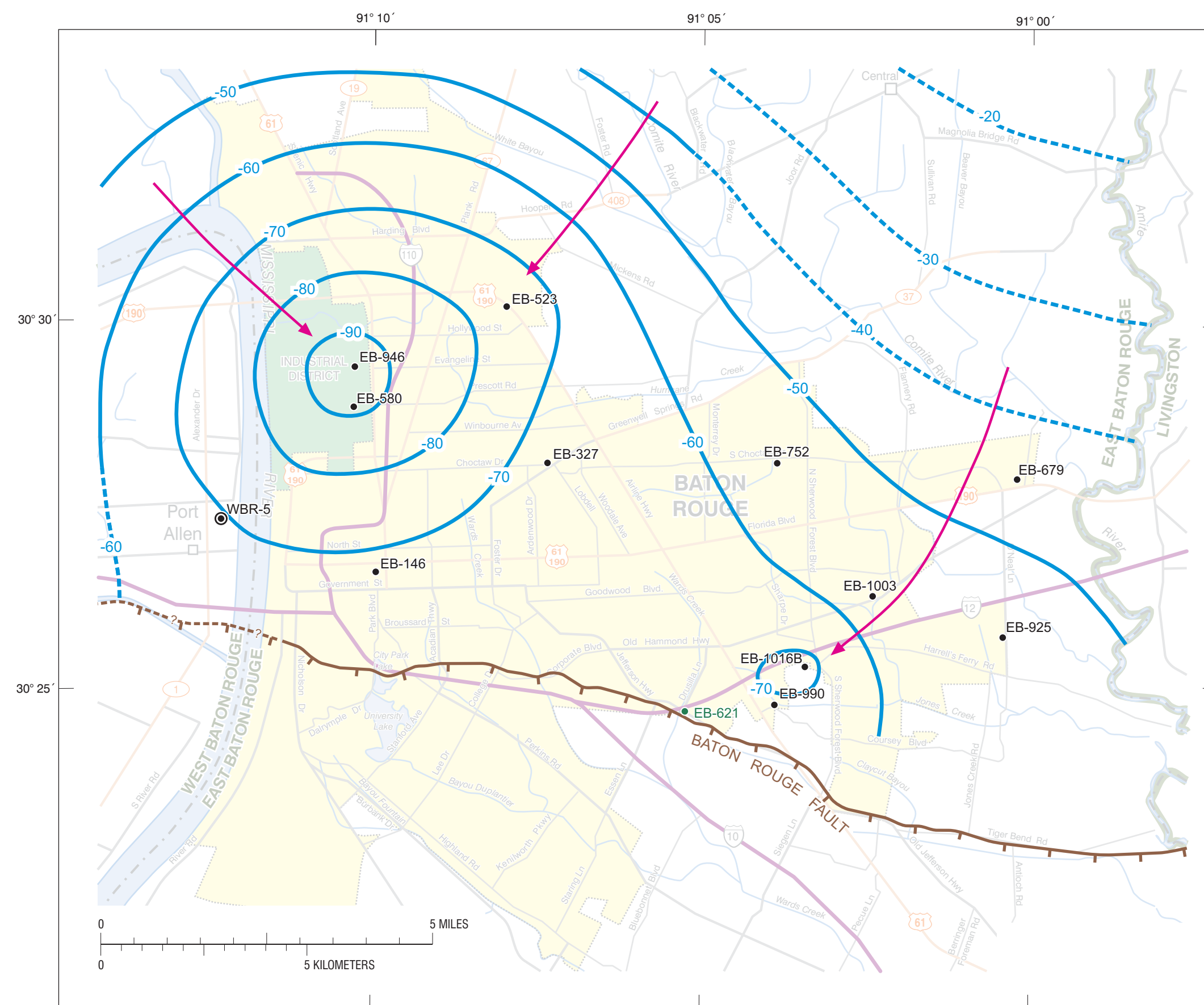
Base map modified from Louisiana Oil Spill Coordinator, Office of the Governor, Louisiana GIS CD: A Digital Map of the State, Version 2.0 Figure 5. Potentiometric surface of the "1,200-foot" sand in parts of East and West Baton Rouge Parishes, southeastern Louisiana, spring 2001.
