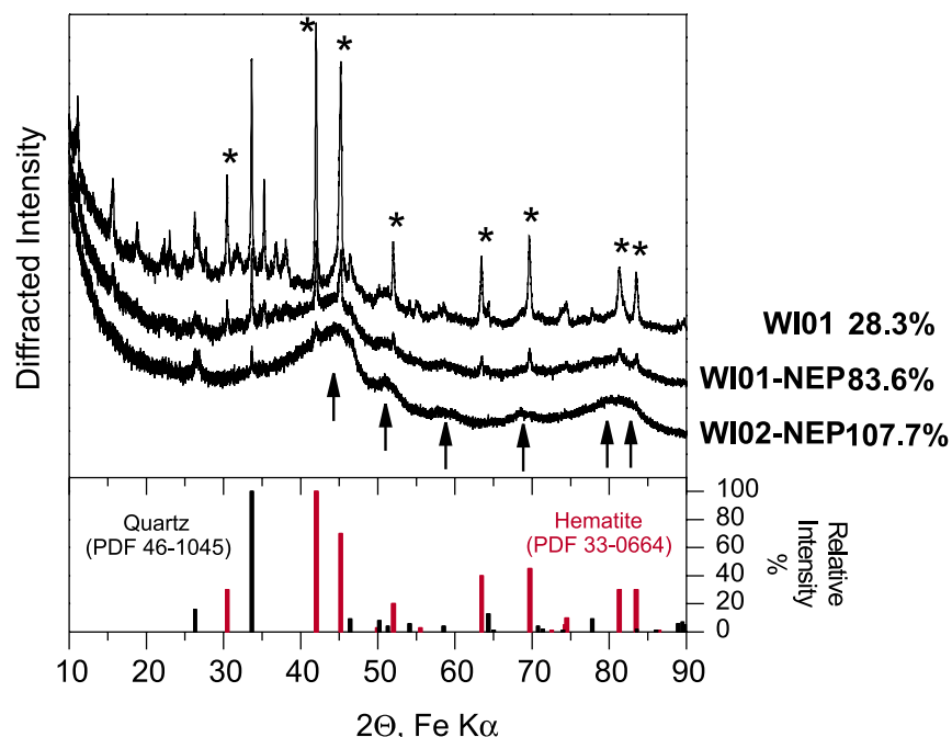
Figure 22 X-ray diffraction data showing the relative proportion of hematite and ferrihydrite in the <math><2\ \mu\text{m}</math> size fraction isolated from surficial sediment samples WI01, WI01-NEP, and WI02-NEP collected near the north-north-western margin of the HBHA Pond. The starred peaks in the pattern for sample WI01 correspond with the dominant peaks in reference hematite (PDF 33-0664). Mean percent iron extracted by ascorbate in duplicate samples is shown to the right of the sample labels. The diffraction pattern for sample WI02-NEP is dominated by a poorly crystalline 6-line ferrihydrite (see peaks marked with arrows).
