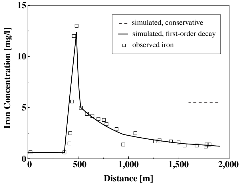
Figure 29. Spatial profile of dissolved iron concentration in St. Kevin Gulch.
