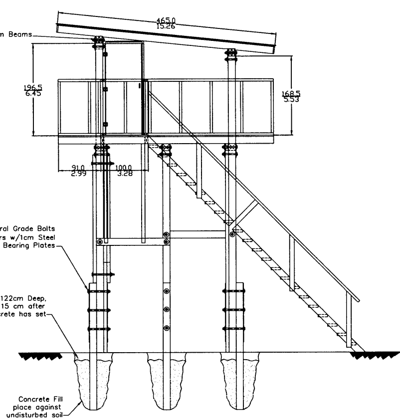
Side View (components omitted for clarity)
