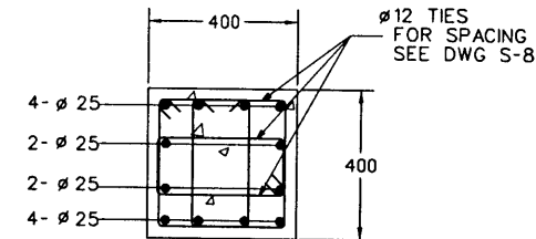
SECTION SCALE 1:10
