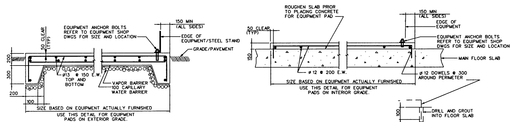
TYPICAL EQUIPMENT PADS NOT TO SCALE
