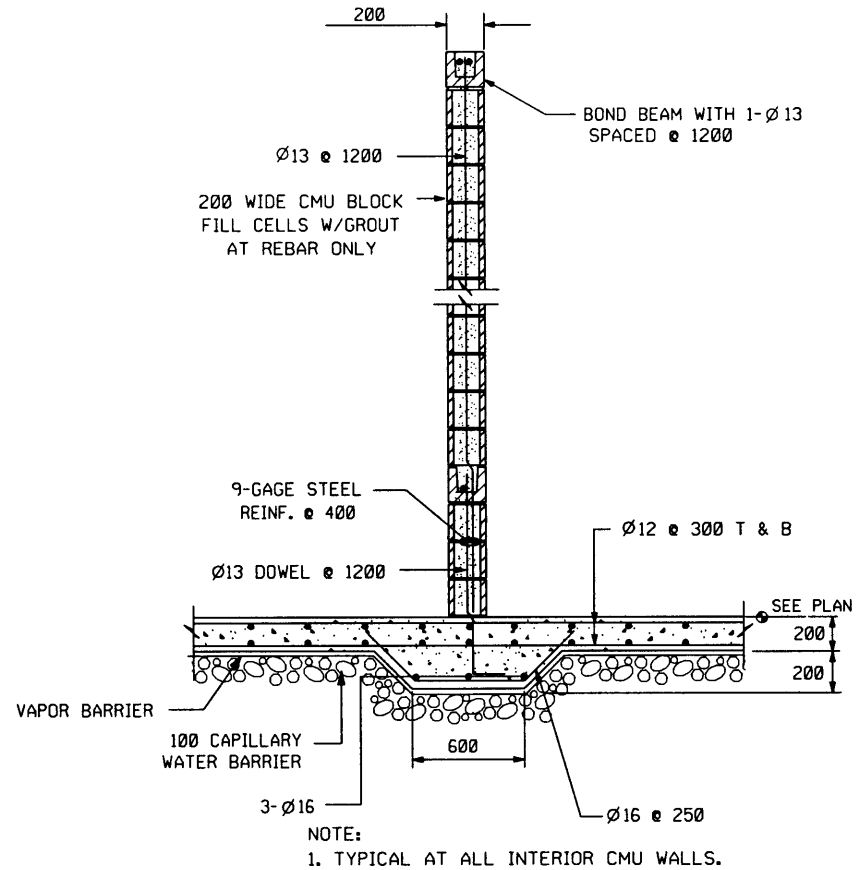
WALL SECTION SCALE NTS
