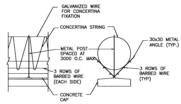
ELEVATION SECTION CONCERTINA STRING & BARBED WIRE DETAILS NOT TO SCALE
