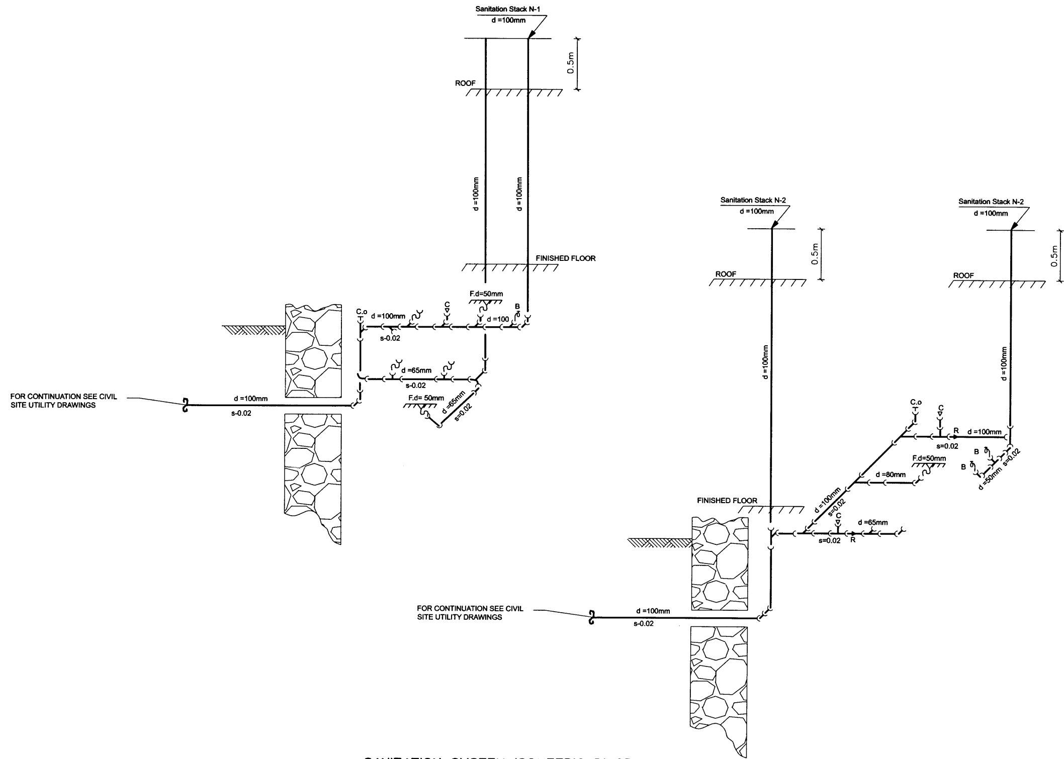
SANITATION SYSTEM ISOMETRIC DIAGRAM NOT TO SCALE
