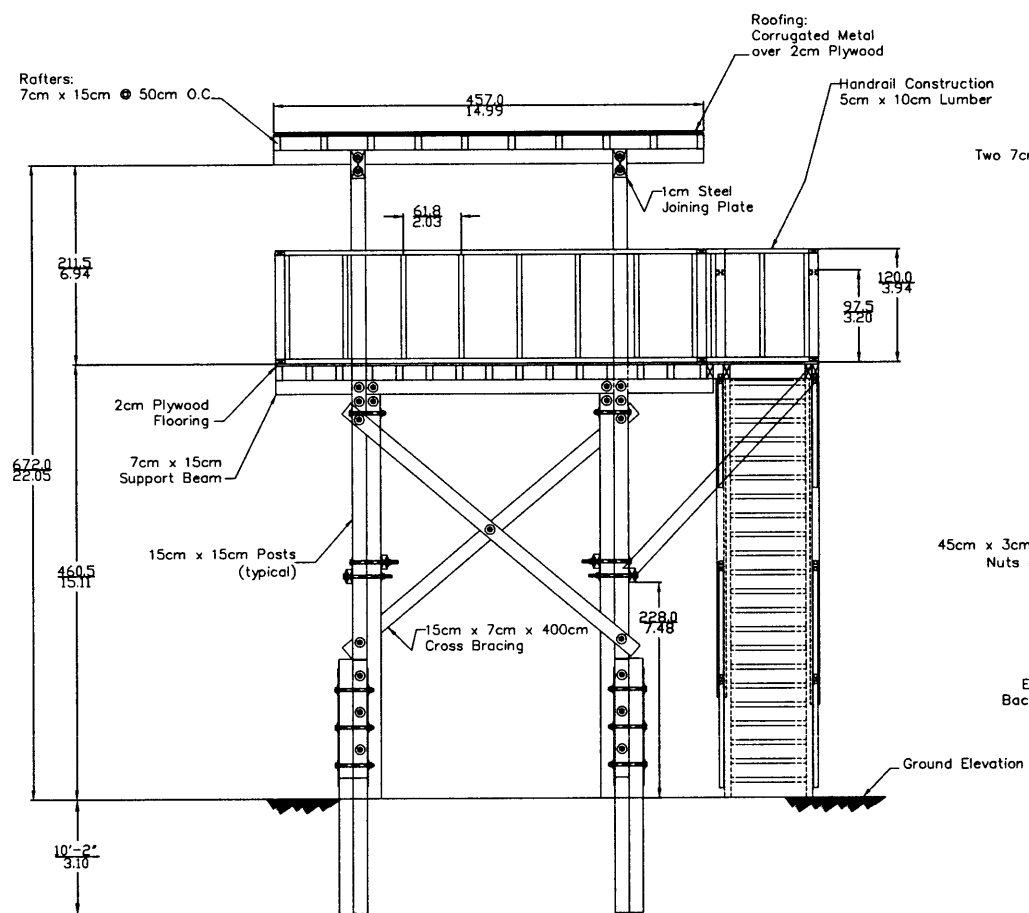
Stairs, Railing & Supports Elevation View
