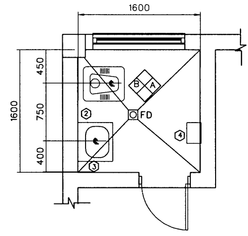
ENLARGED TOILET PLAN NOT TO SCALE
