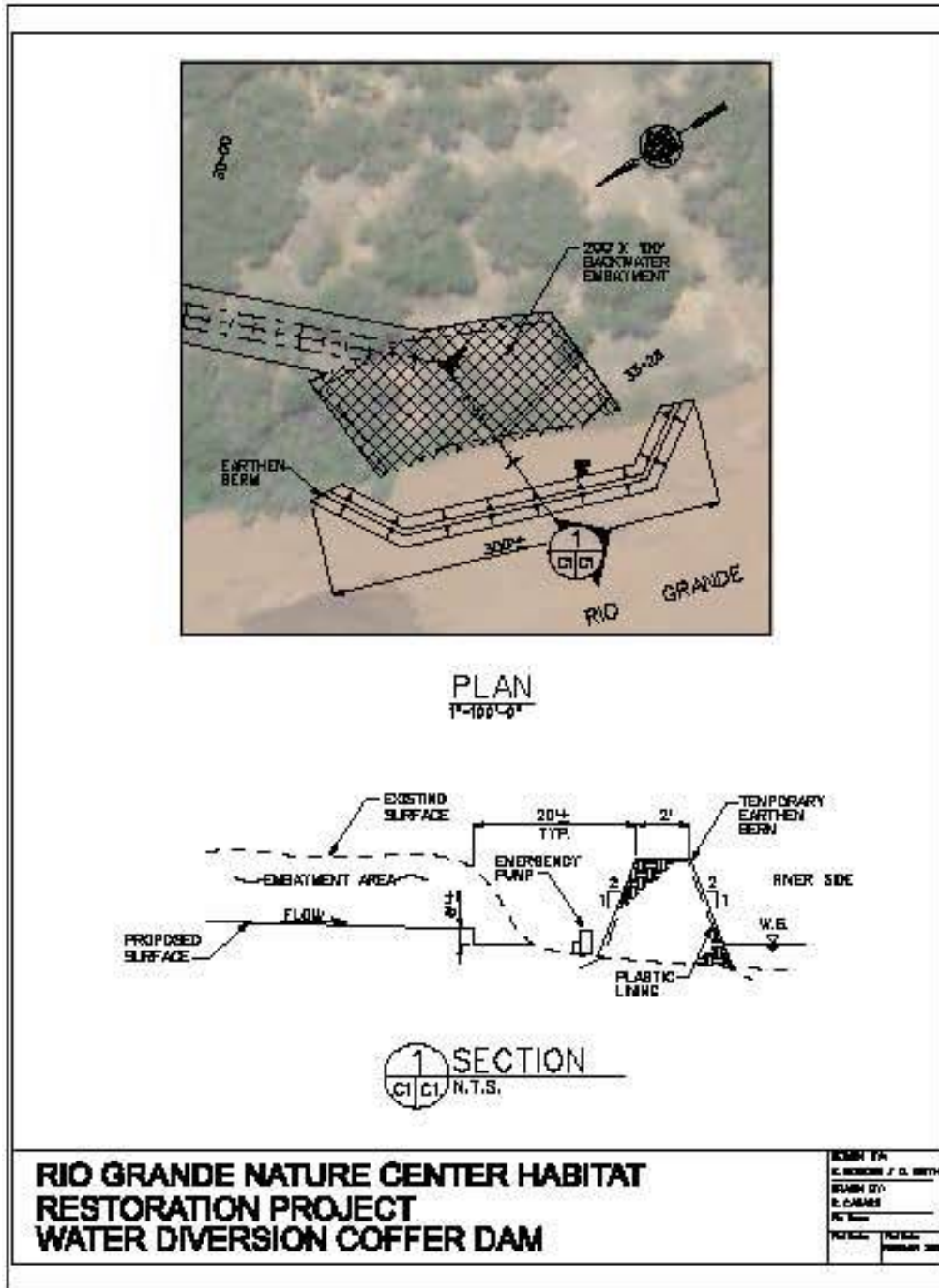
Figure 2. Proposed coffer dam for use during construction of channel openings.
