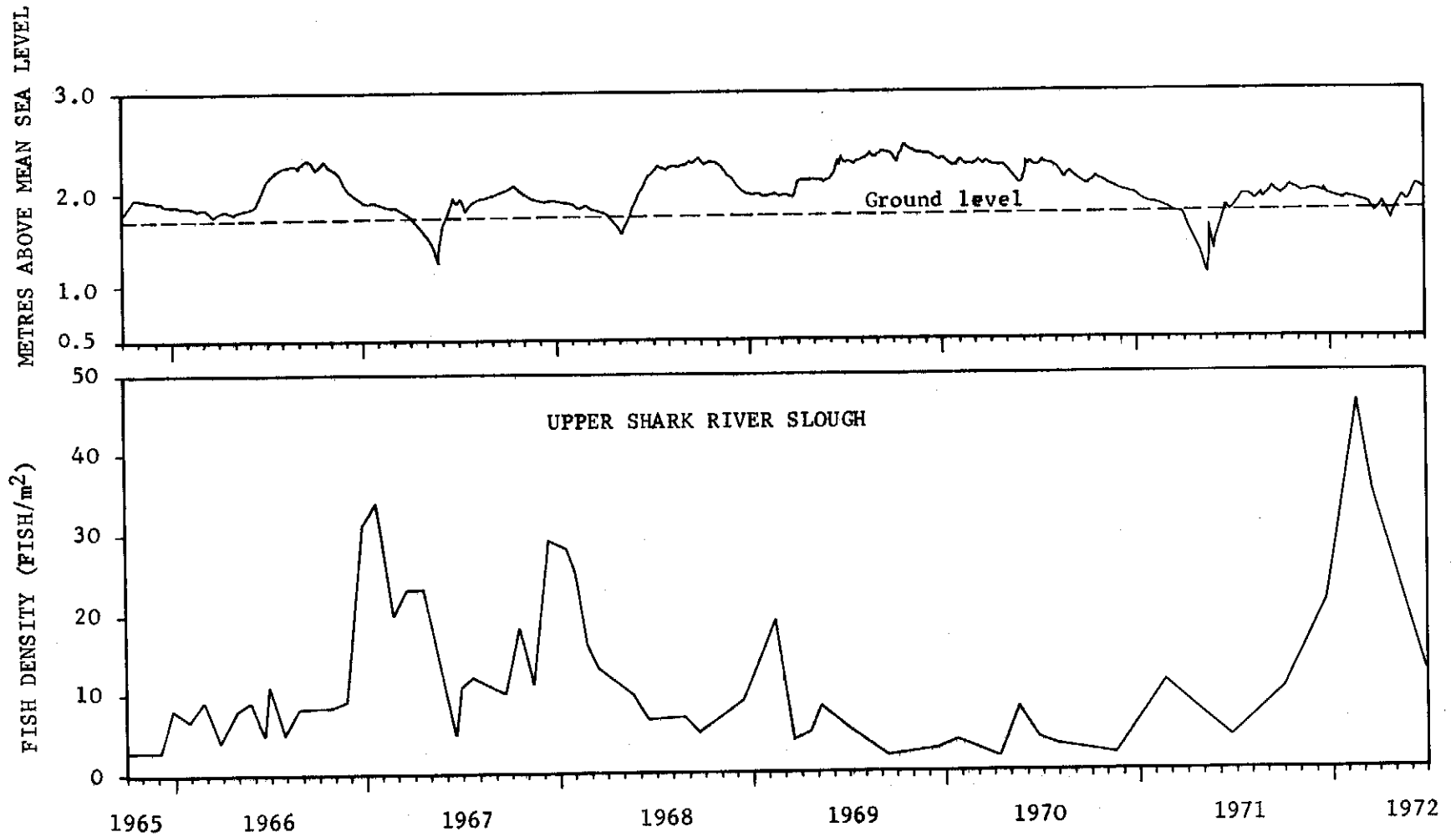
Figure 10.--Fluctuations of water level at P-33 and density of fish in Shark River Slough.
