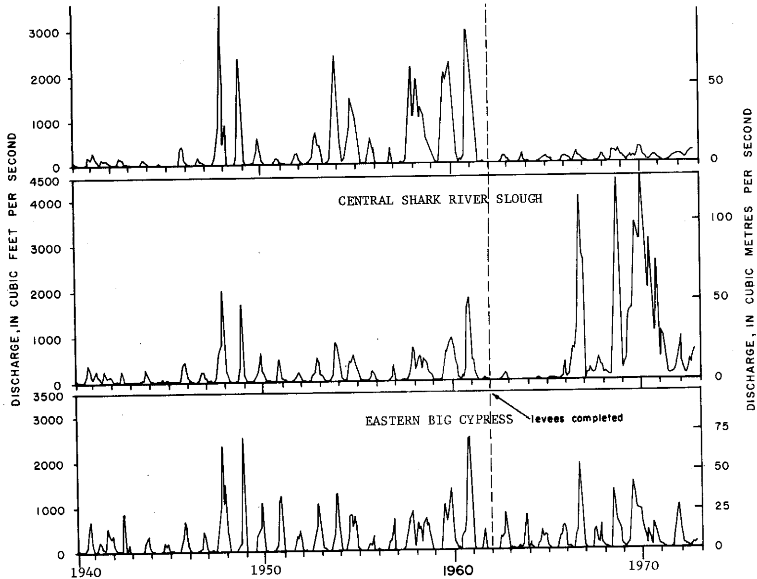
Figure 3.--Surface-water flow into two sections of Shark River Slough and through the eastern Big Cypress Swamp.
