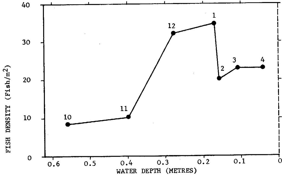
Figure 9.--Relation between fish density in the marshes of Shark River Slough and water level, October 1966 to April 1967. Numbers at data points indicate month of datum.
