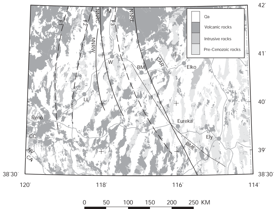
FIG. 2. Simplified geologic map of northern Nevada showing the association of Tertiary volcanic rocks with the mid-Miocene northern Nevada rift-east (NNRE) and associated features (northern Nevada rift-west [NNRW], northern Nevada rift-central [NNRC]). Modified from Stewart and Carlson (1978). Explanation as in Figure 1.
