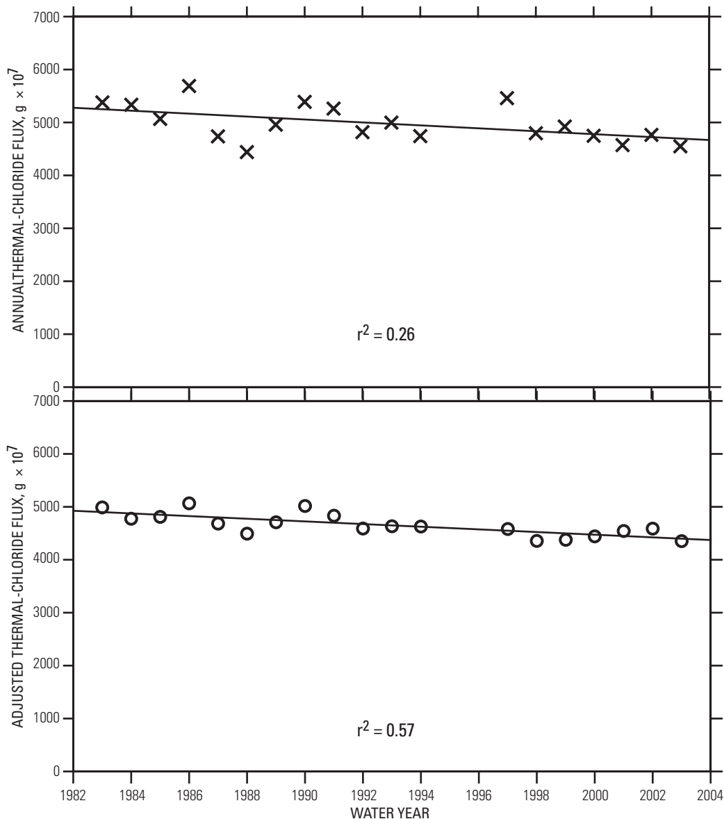
Figure 13. Graphs of the unadjusted and adjusted annual thermal-chloride flux out of Yellowstone Park for each water year.
