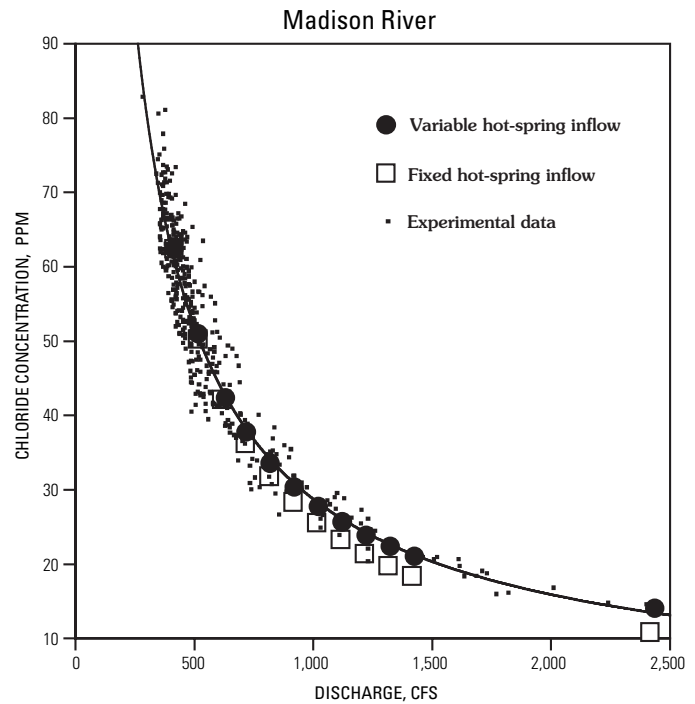
Figure 8. Graph of chloride concentration versus discharge for the Madison River showing experimental data and models of inflow to the river from various sources.
