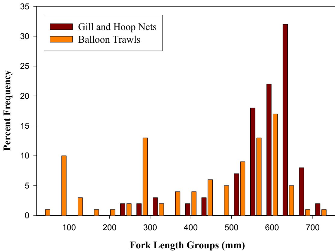
Figure 5. Percent length frequency of shovelnose sturgeon captured in slingshot balloon trawls, gill nets and hoop nets at six sites on the Lower Missouri River in 2001.
