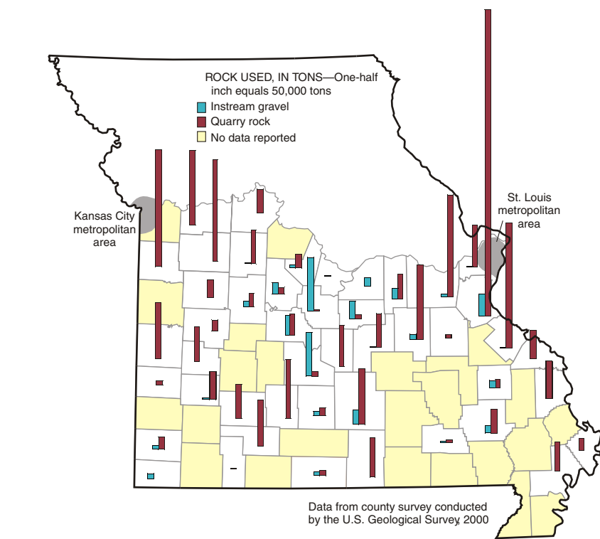
Figure 2. Rock use by county highway departments, 1999.
