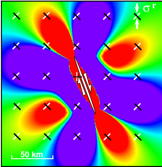
N-S Regional Compression
