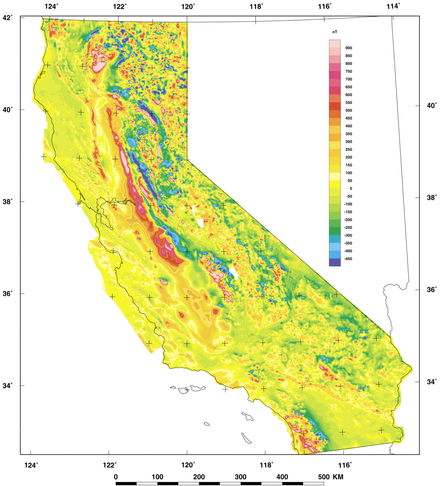
Figure 2. Preliminary aeromagnetic anomaly map of California.
