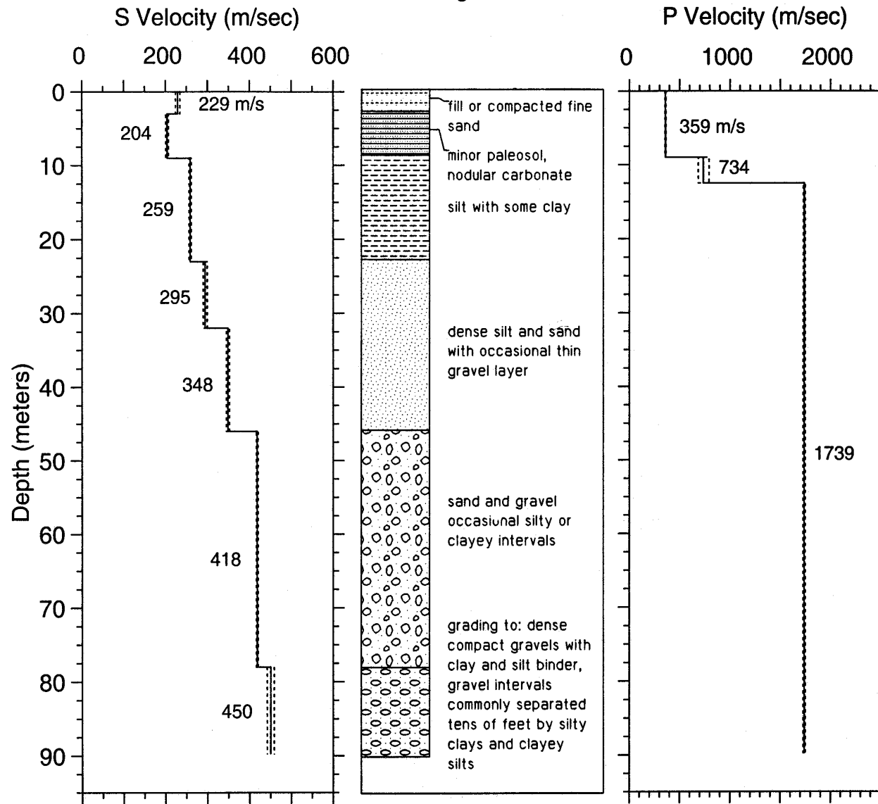
Figure A-15. Velocity profiles for the borehole at Cerritos College Police Building. Generalized geology is shown for correlation with velocities. Dashed lines are one standard deviation.
