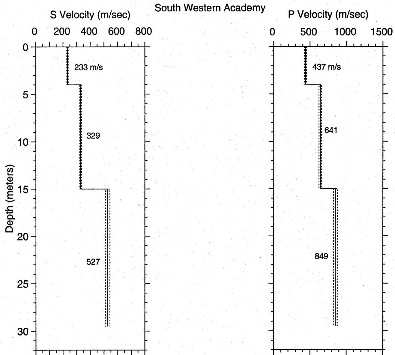
Figure A-60. S- and P-wave velocity profiles with dashed lines representing one standard deviation. Lithology is not available from this borehole.
