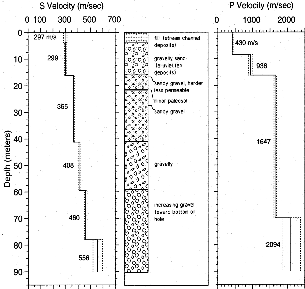
Figure A-50. S- and P-wave velocity profiles with dashed lines representing one standard deviation. Lithology is shown for correlation with velocities.
