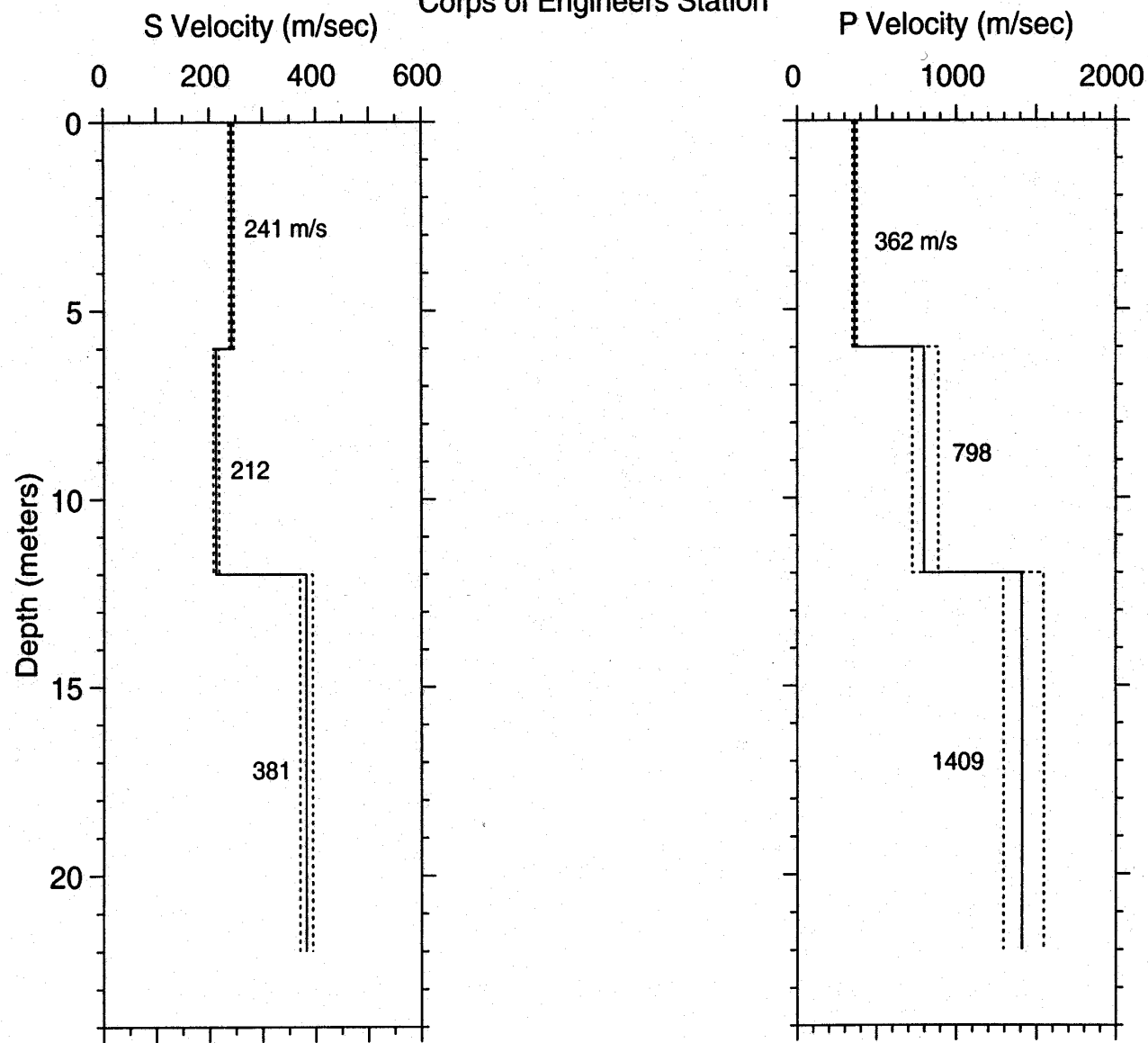
Figure A-20. S- and P-wave velocity profiles with dashed lines representing one standard deviation. Lithology is not available from this borehole.
