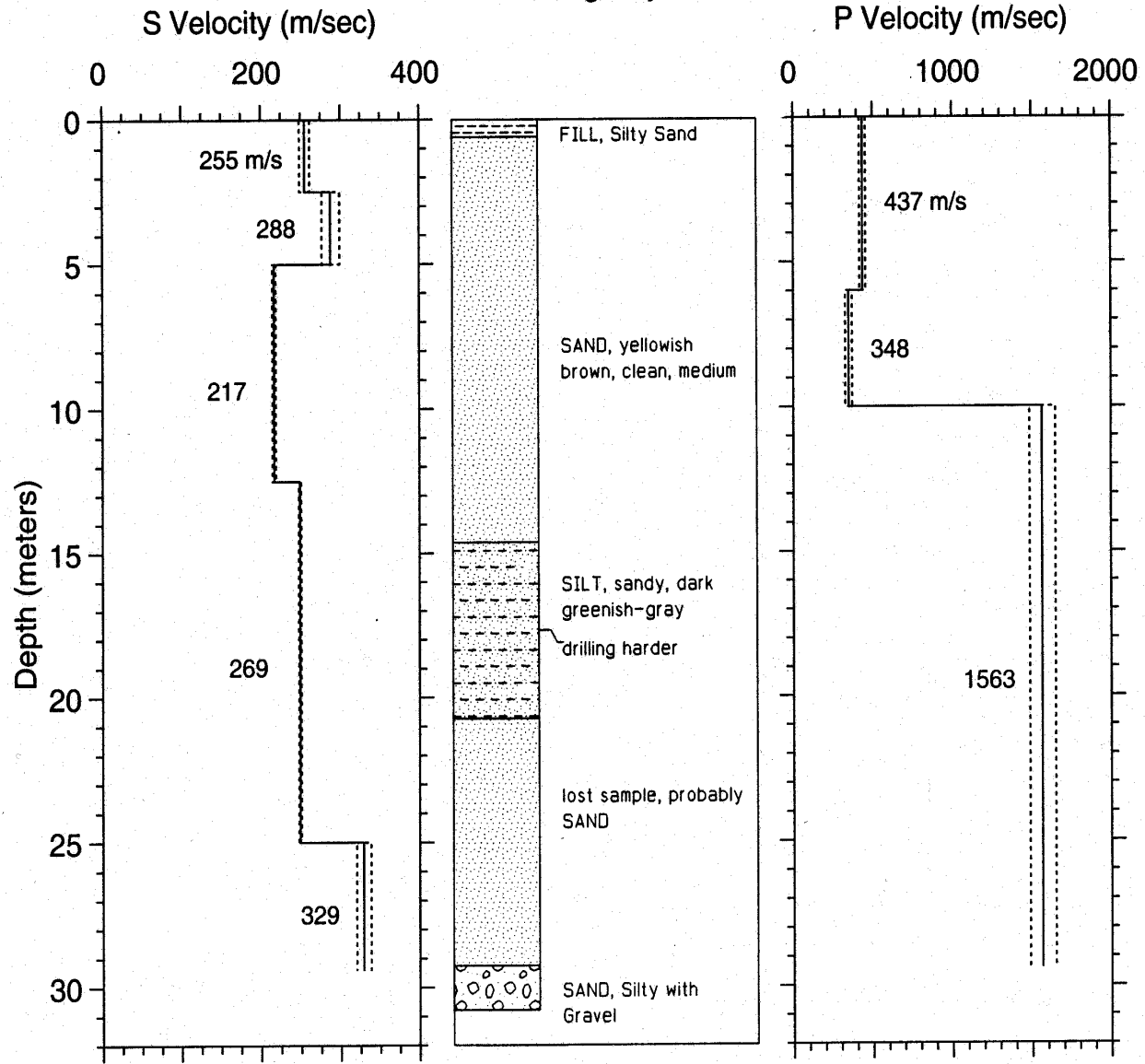
Figure A-5. S- and P-wave velocity profiles with dashed lines representing plus and minus one standard deviation. Generalized geologic log is shown for correlation with velocities.
