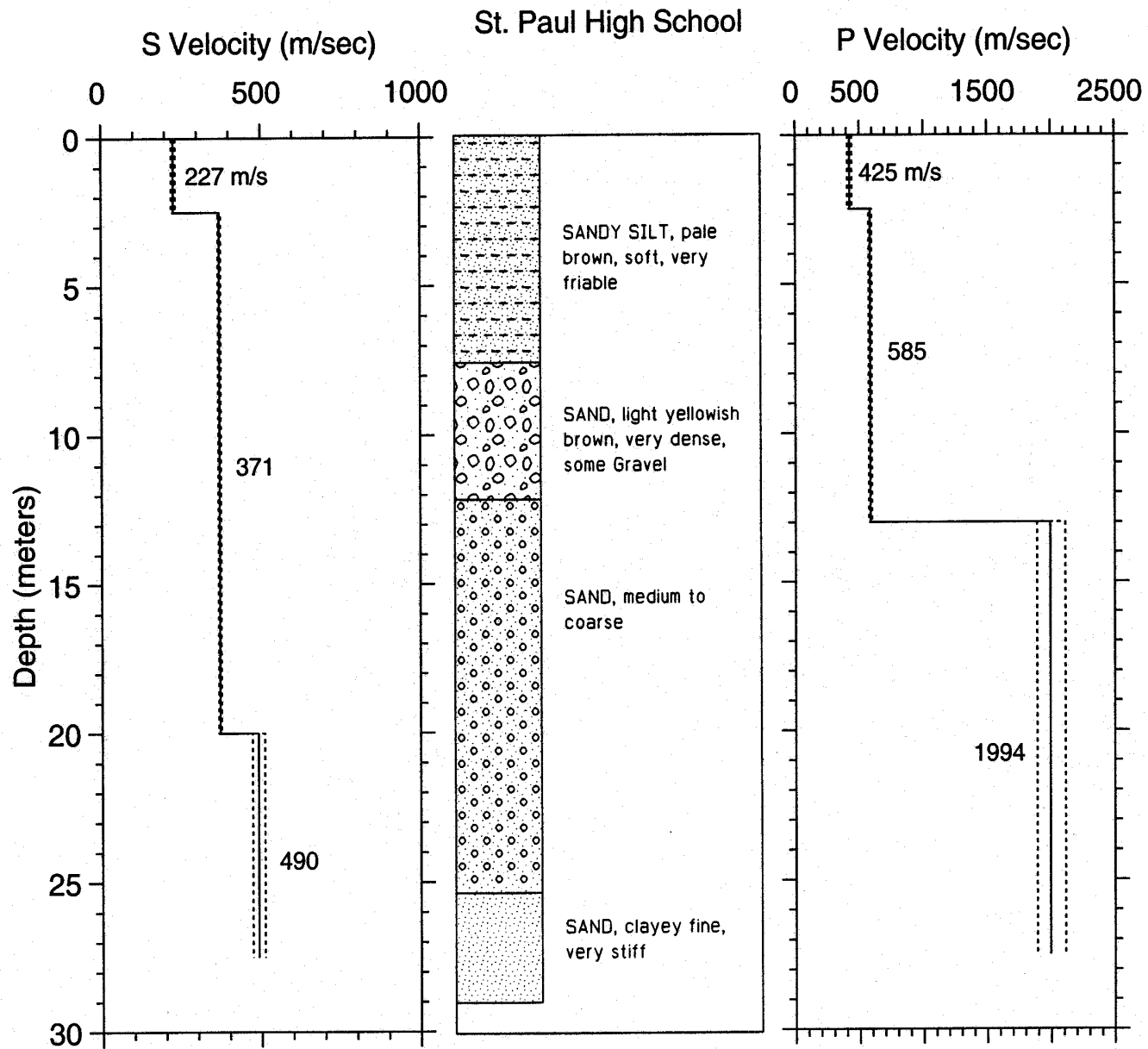
Figure A-65. S- and P-wave velocity profiles with dashed lines representing one standard deviation. Lithology is shown for correlation with velocities.
