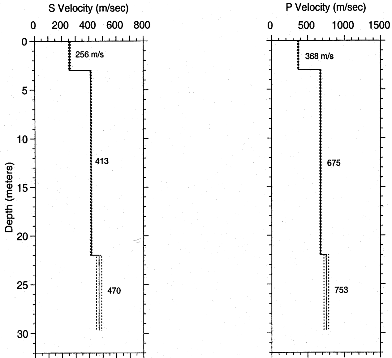
Figure A-30. S- and P-wave velocity profiles with dashed lines representing one standard deviation. Lithology is not available from this borehole.
