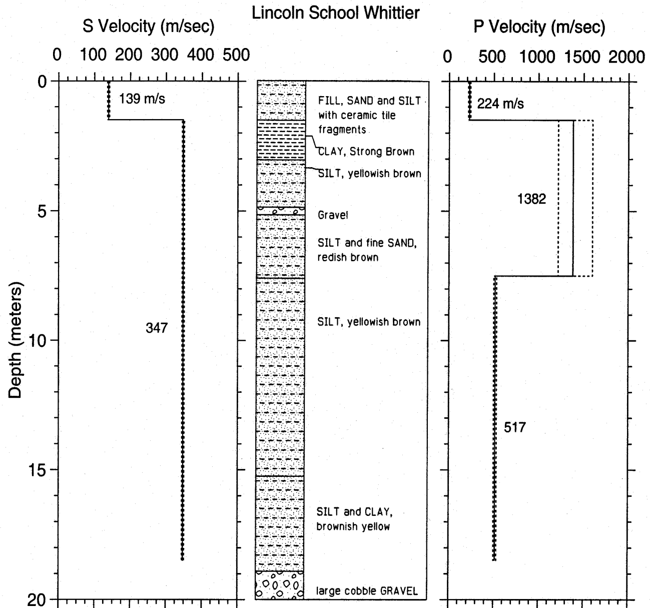
Figure A-35. S- and P-wave velocity profiles. Dashed lines represent one standard deviation. Lithology is shown for correlation with velocities.
