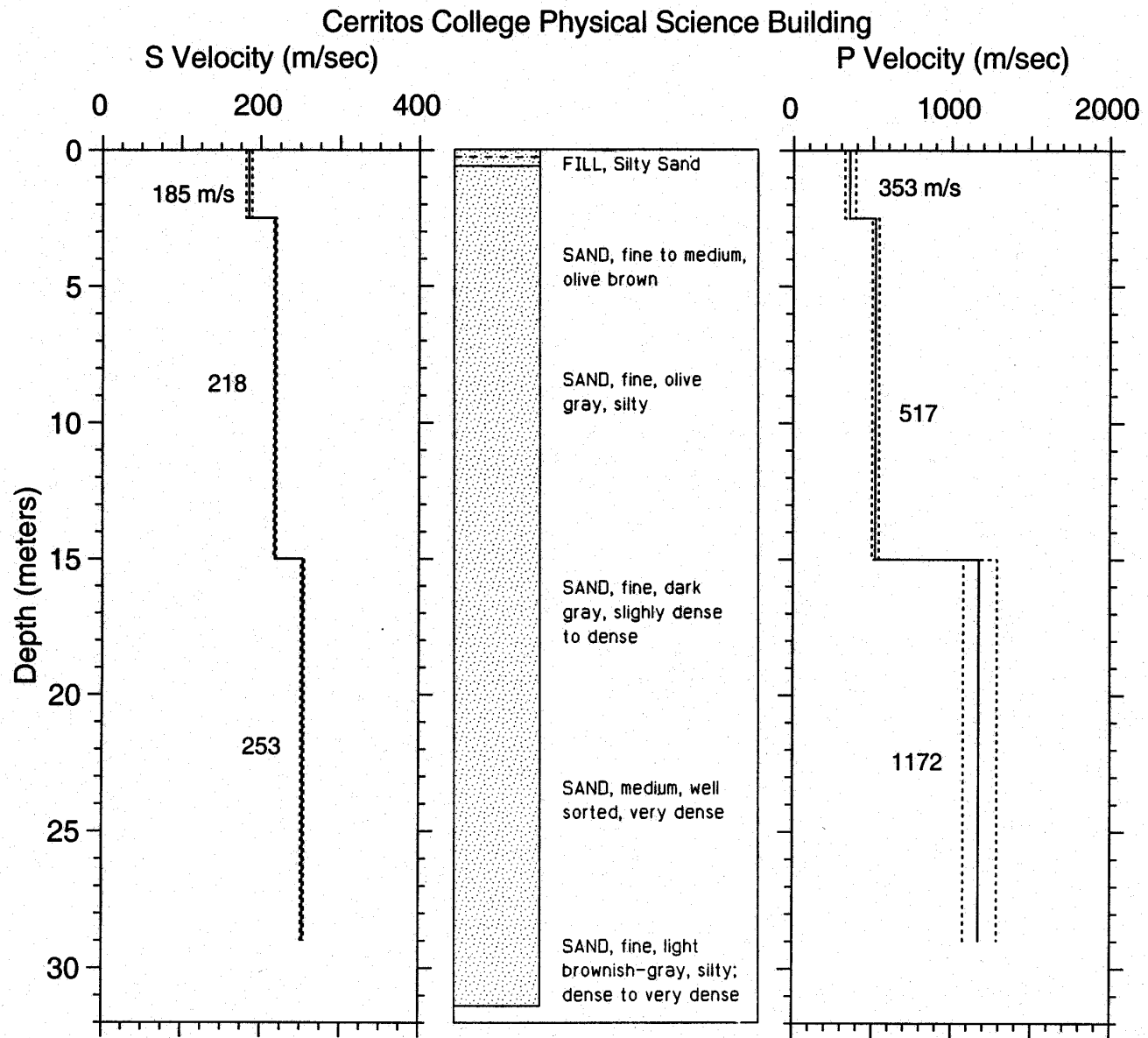
Figure A-10. S- and P-wave velocity profiles with generalized geologic log. Dashed lines represent plus and minus one standard deviation.
