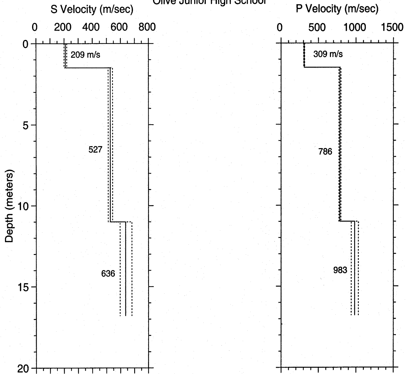
Figure A-45. S- and P-wave velocity profiles with dashed lines representing one standard deviation. Lithology is not available from this borehole.
