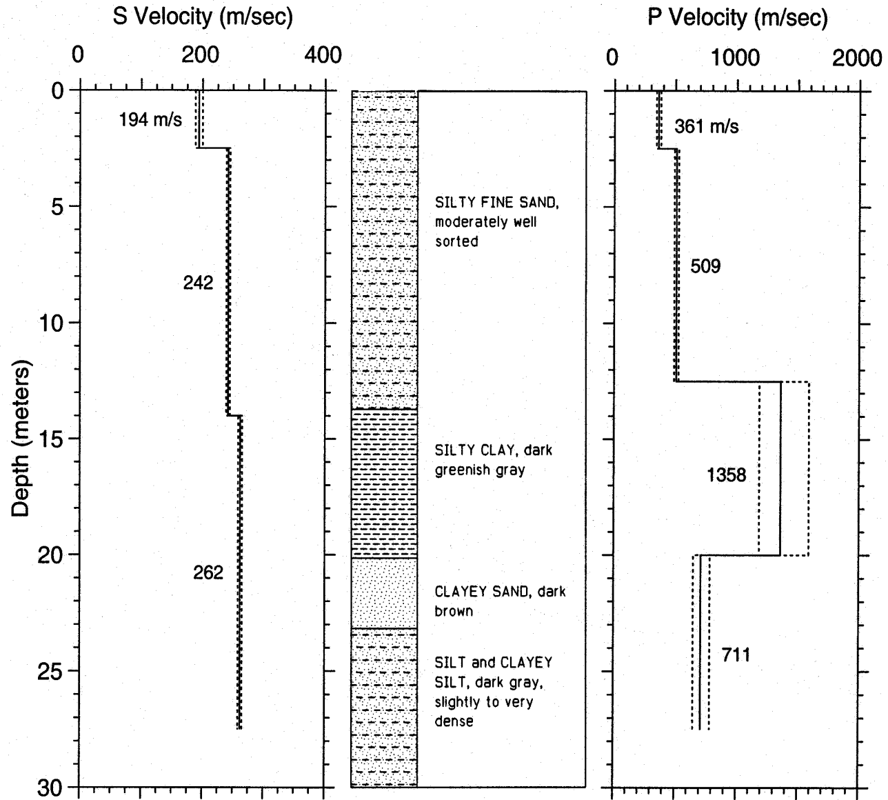
Figure A-40. S- and P-wave velocity profiles with dashed lines representing one standard deviation. Lithology is shown for correlation with velocities.
