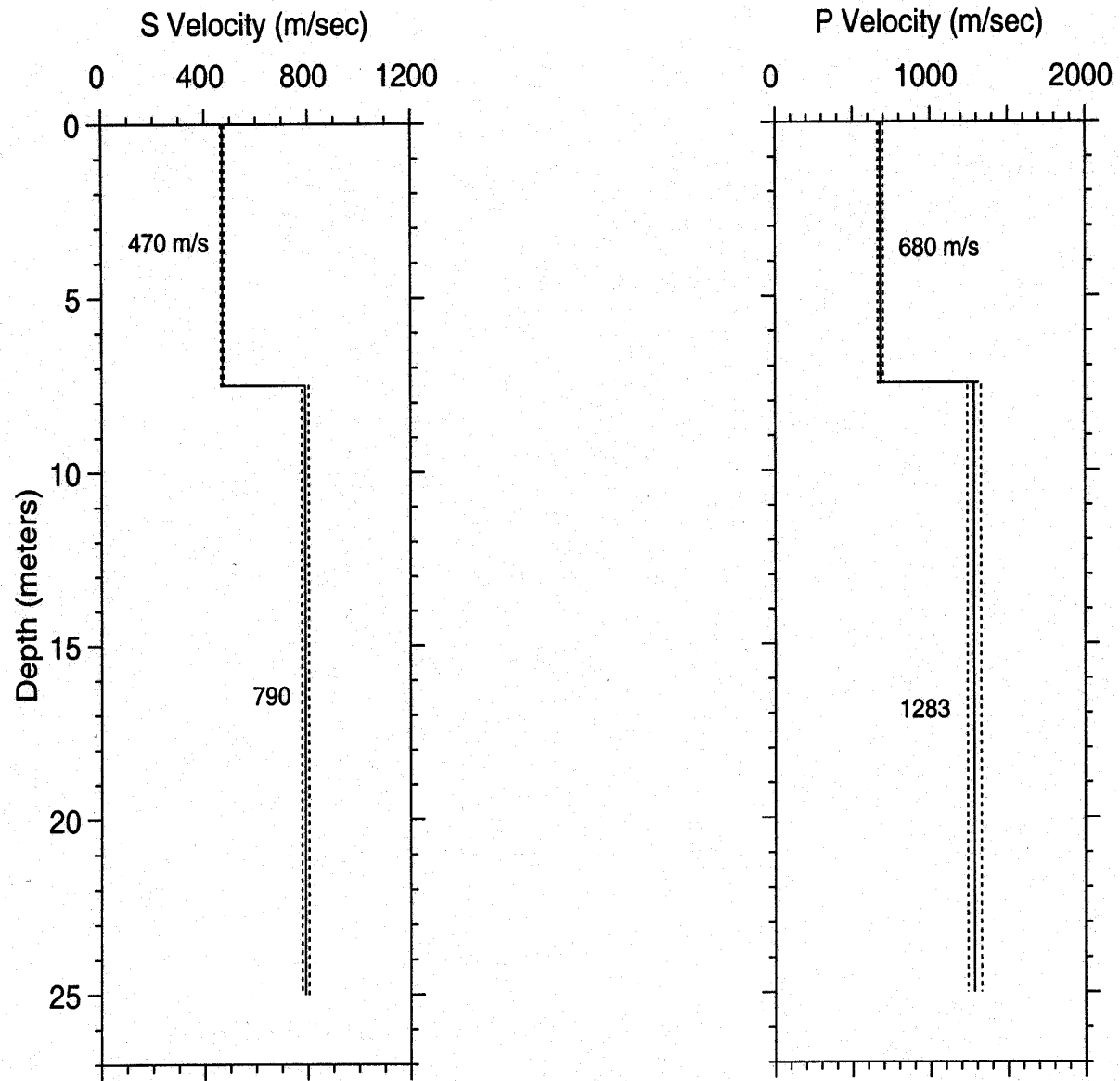
Figure A-25. S- and P-wave velocity profiles with dashed lines representing one standard deviation. Lithology is not available from this borehole.
