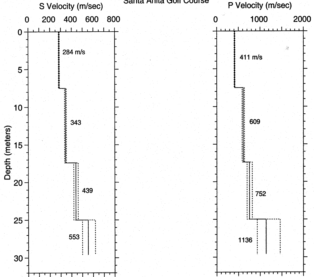
Figure A-55. S- and P-wave velocity profiles with dashed lines representing one standard deviation. Lithology is not available from this borehole.
