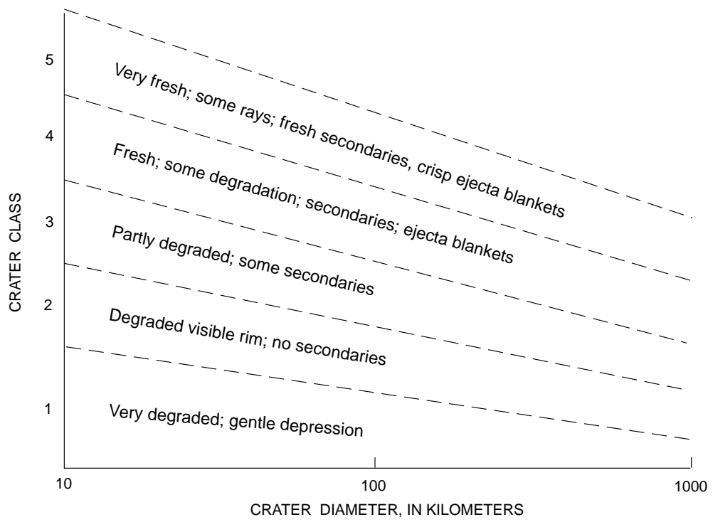
Figure 1. Diagrammatic representation of crater classes, showing effects of crater size on retention of morphological features.
