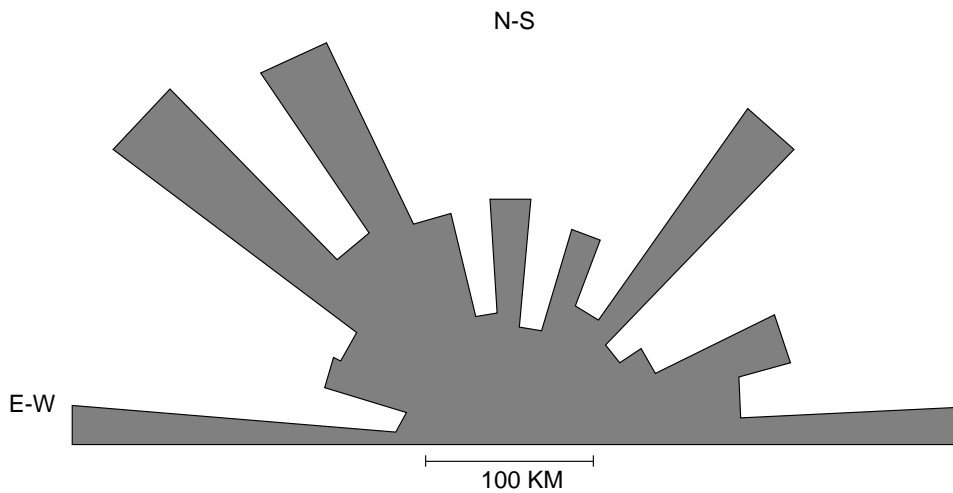
Figure 2. Azimuth-frequency distribution of cumulative lengths of linear crater-well segments.
