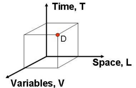
Figure 12: Data cube
