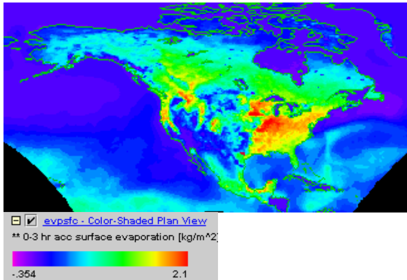
Figure 6. Surface evaporation over North America from the North American Regional Reanalysis of climate visualized with Unidata's Integrated Data Viewer.
