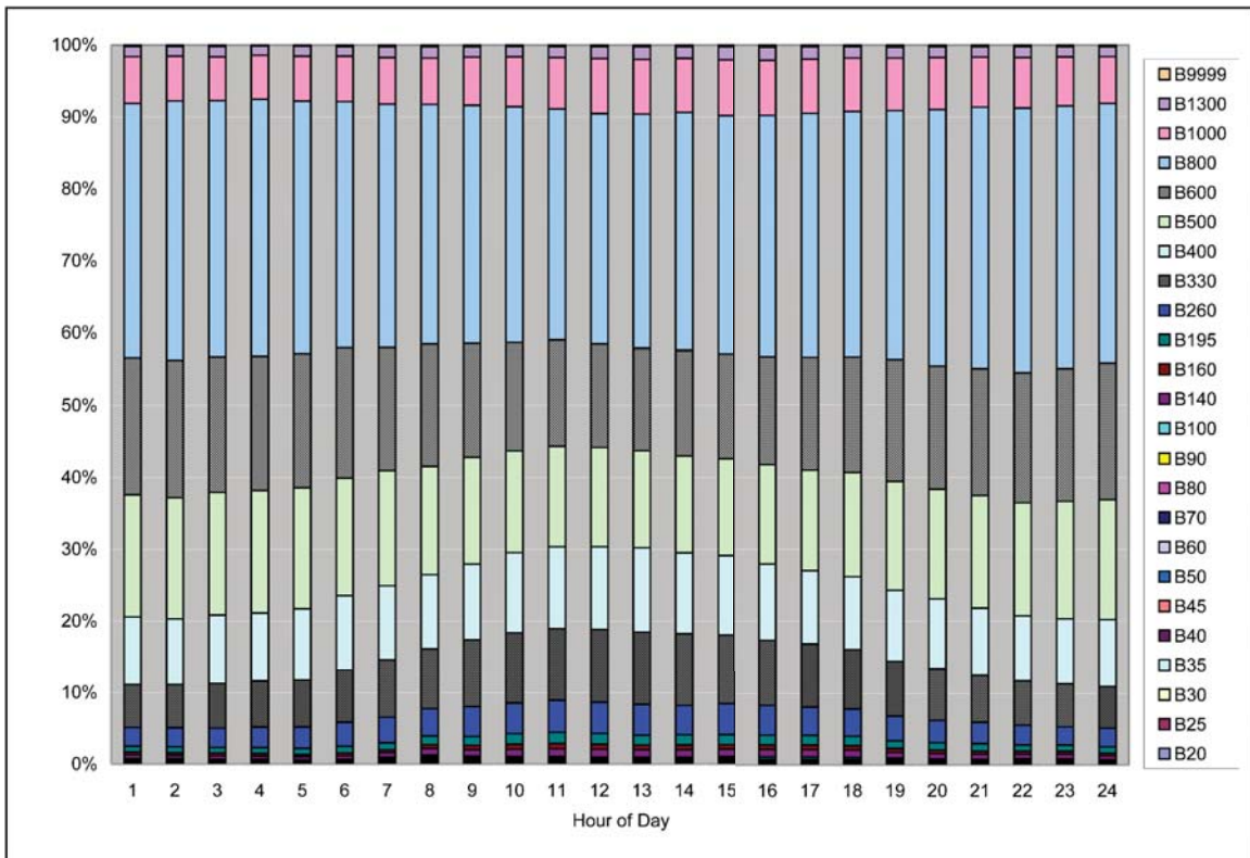
Figure 29. Vehicle group (8 – 13) weight bin distribution over an average Wednesday.
