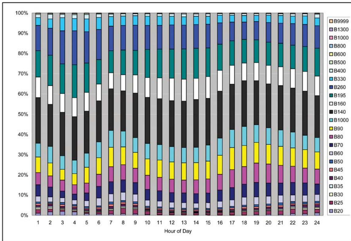
Figure 28. Vehicle 5 weight bin distribution over an average Wednesday.
