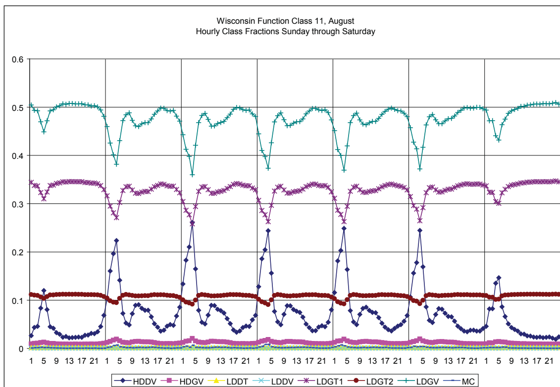
Figure B-1. Vehicle fractional mix over a week for urban interstates in Wisconsin.
