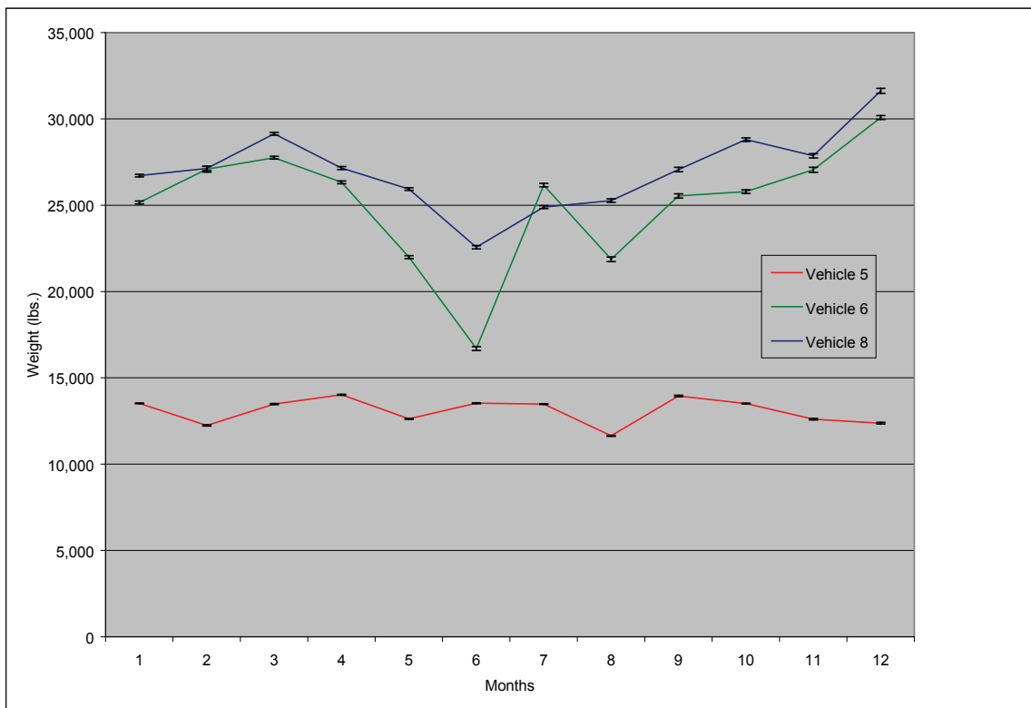
Figure 16. Average weight by month for lighter heavy vehicle classes in 1999 on road type 1. (Uncertainty ranges were based on 90% confidence levels of the sample.)
