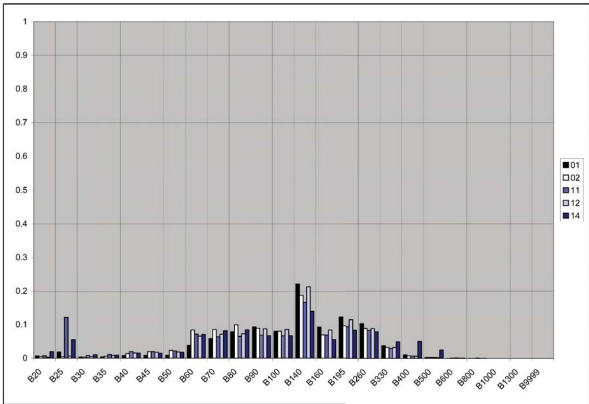
Figure 38. Vehicle 5 weight bin distribution in 1999 by functional class.
