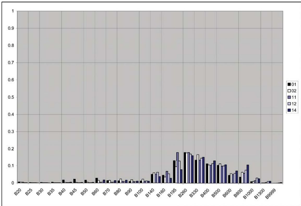
Figure 39. Vehicle 6 and 7 weight bin distribution in 1999 by functional class.
