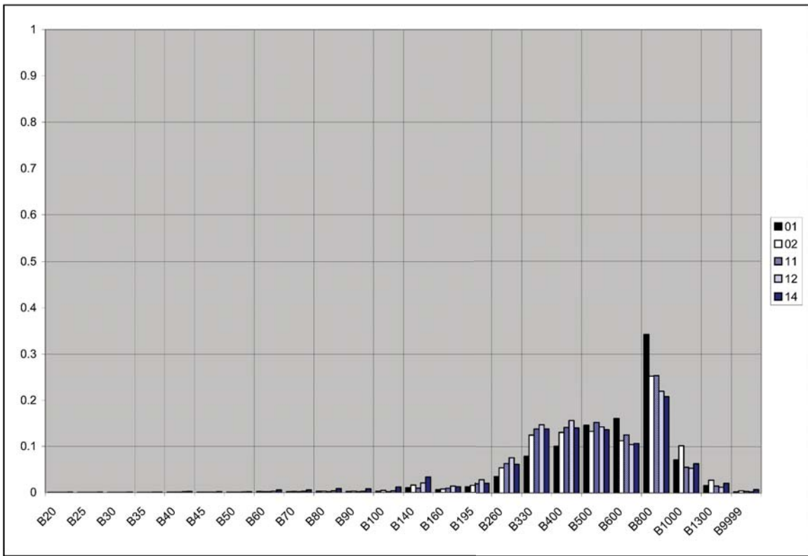
Figure 40. Vehicle 8-13 weight bin distribution in 1999 by functional class.
