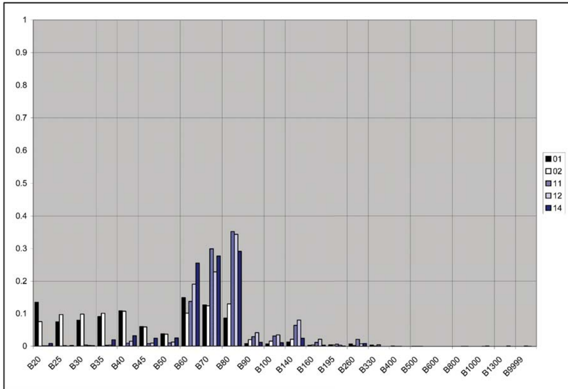
Figure 35. Vehicle 2 weight bin distribution in 1999 by functional class.
