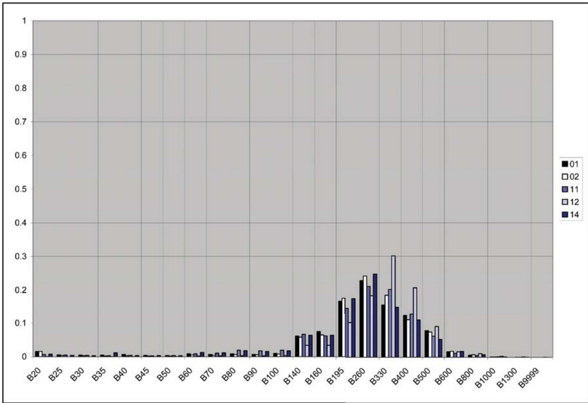
Figure 36. Vehicle 3 weight bin distribution in 1999 by functional class.
