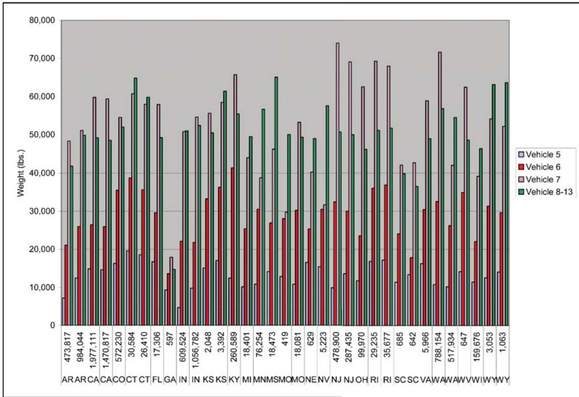
Figure 15. Average vehicle weight for vehicle classes 5 – 13 on urban interstates, road 11. (Number of site-days of observations used in the state average reported along axis.)
