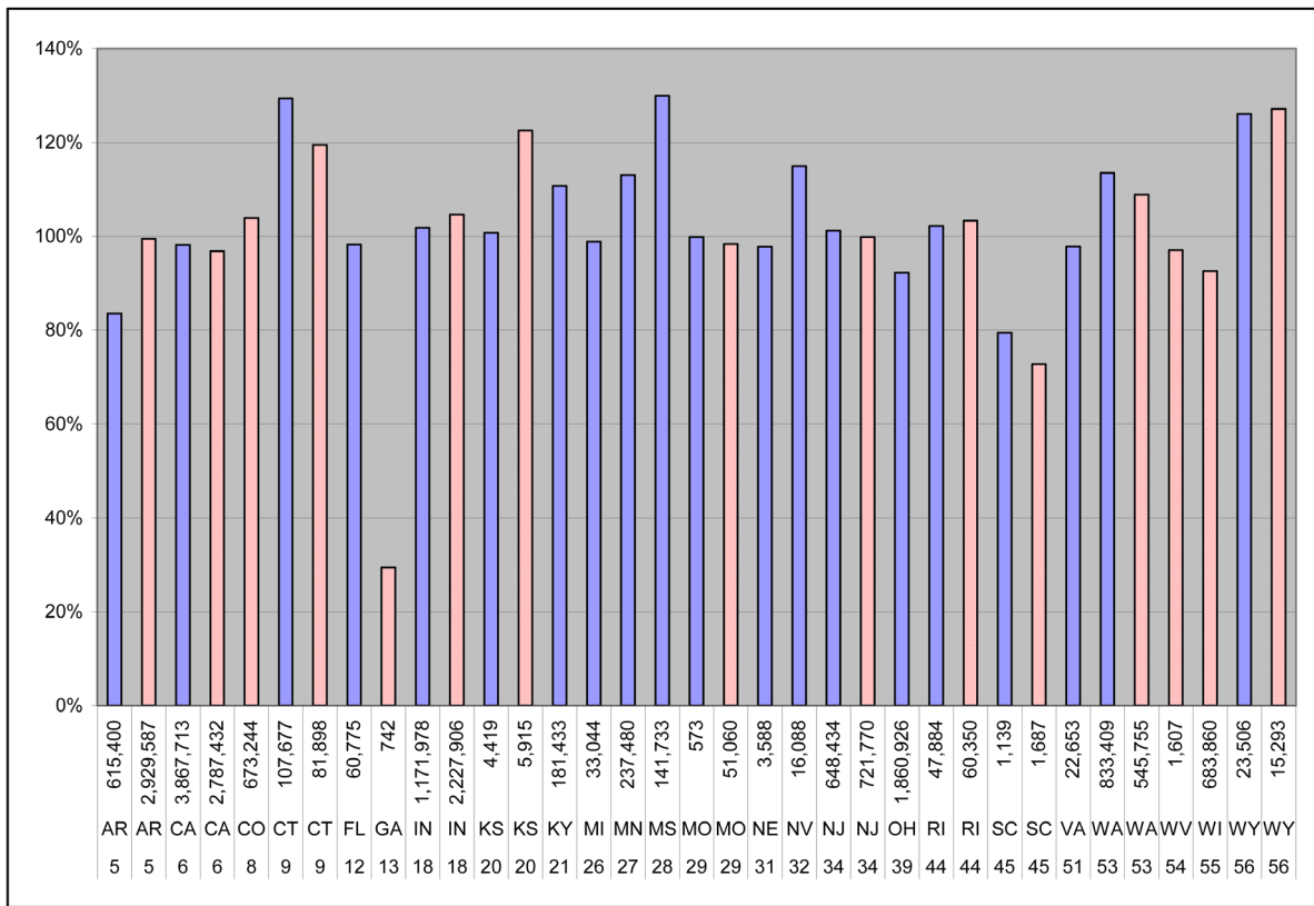
Figure 6. Relative average weight by state for vehicles 8 – 13 in 1999 and 2000 on road type 1, rural interstates. (Number of observations used for each state average reported along axis. 1999 data is solid blue and 2000 is red on white hash.)
