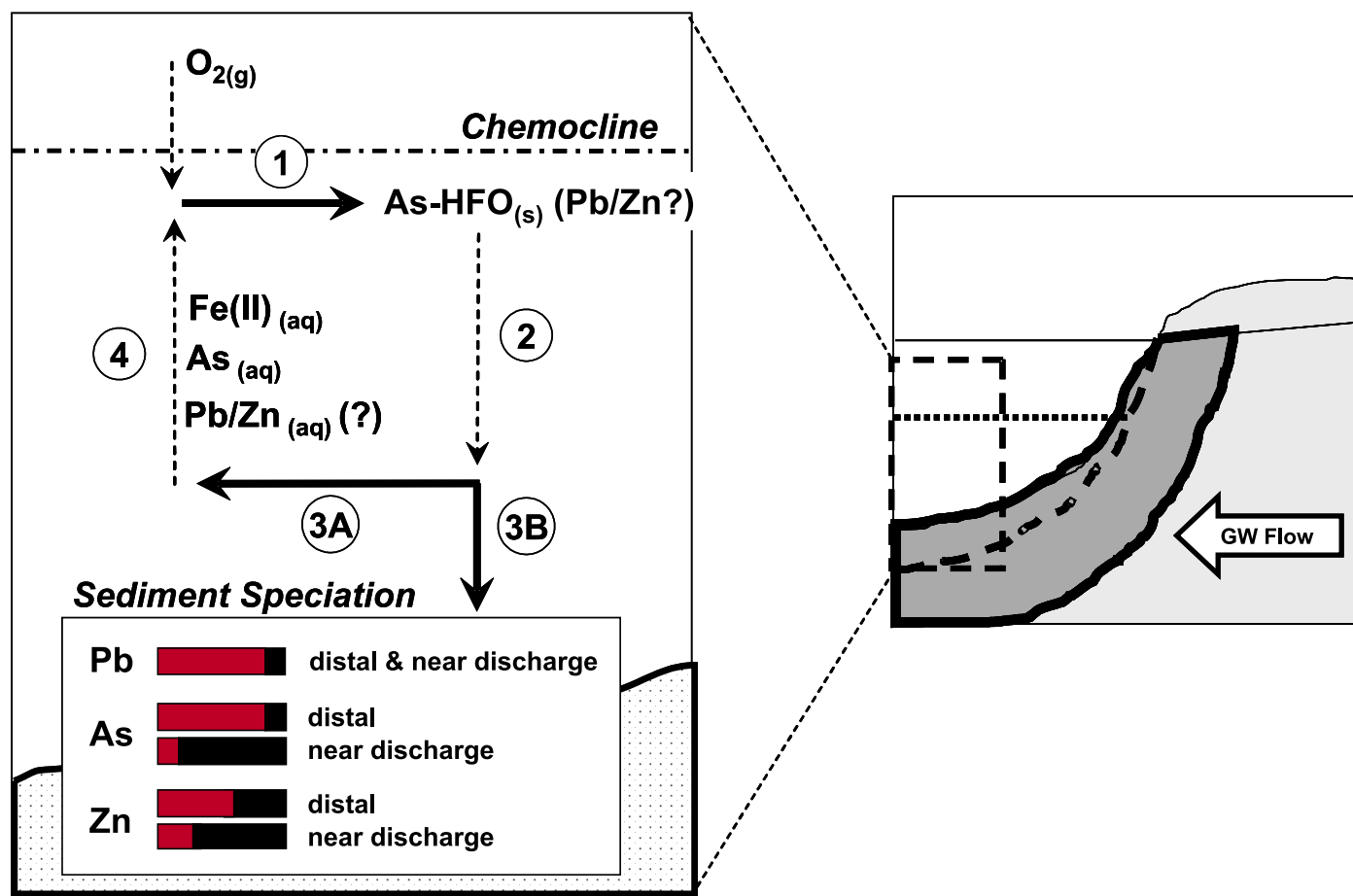
Figure 31 Illustration of the apparent geochemical processes controlling solid-solution partitioning of arsenic, lead, and zinc within the HBHA Pond: 1) Fe(II) oxidation near chemocline upon encountering dissolved oxygen and coprecipitation of As with iron (hydr)oxides, 2) settling of precipitated iron (hydr)oxides, 3A) reductive dissolution of a fraction of settling iron (hydr)oxides generating dissolved Fe(II) and arsenic, 3B) deposition and diagenesis of a fraction of precipitated iron (hydr)oxides – partial conversion to iron sulfides, and 4) vertical transport of dissolved Fe(II) and As up to the chemocline. The speciation of arsenic, lead, and zinc in sediments located near and distal to the primary zone of contaminated ground-water discharge is shown (red = oxide association; black = sulfide association).
