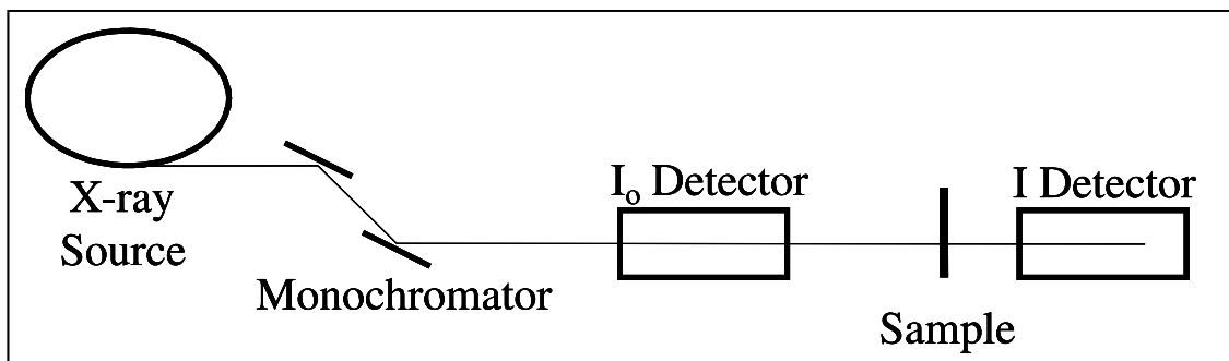
Figure C.3 Experimental configuration for transmission data collection.
