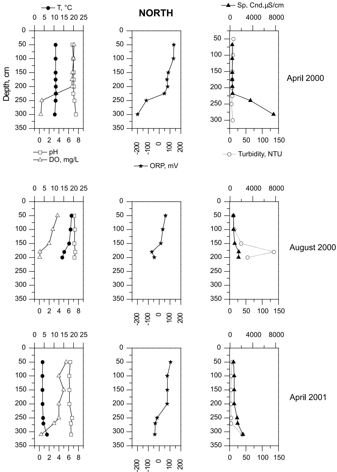
Figure 9 Vertical patterns in water quality within the northern part of the HBHA Pond on sampling dates in April 2000, August 2000, and April 2001. Symbols: T = temperature, DO = dissolved oxygen, ORP = oxidation-reduction potential, and Sp. Cnd. = specific conductance.
