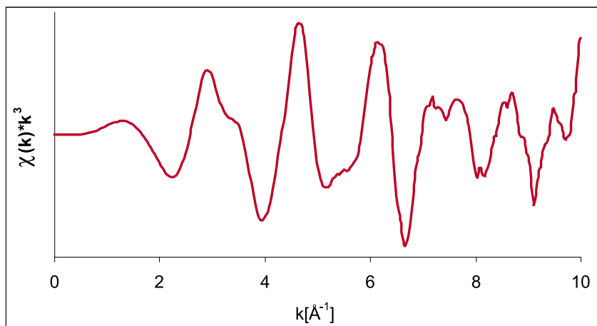
Figure C.13 The k^3 -weighted \chi -function of Figure C.12. The oscillations describe the photoelectron wave number as the photoelectron constructively and destructively interacts with neighboring atoms around PC.
