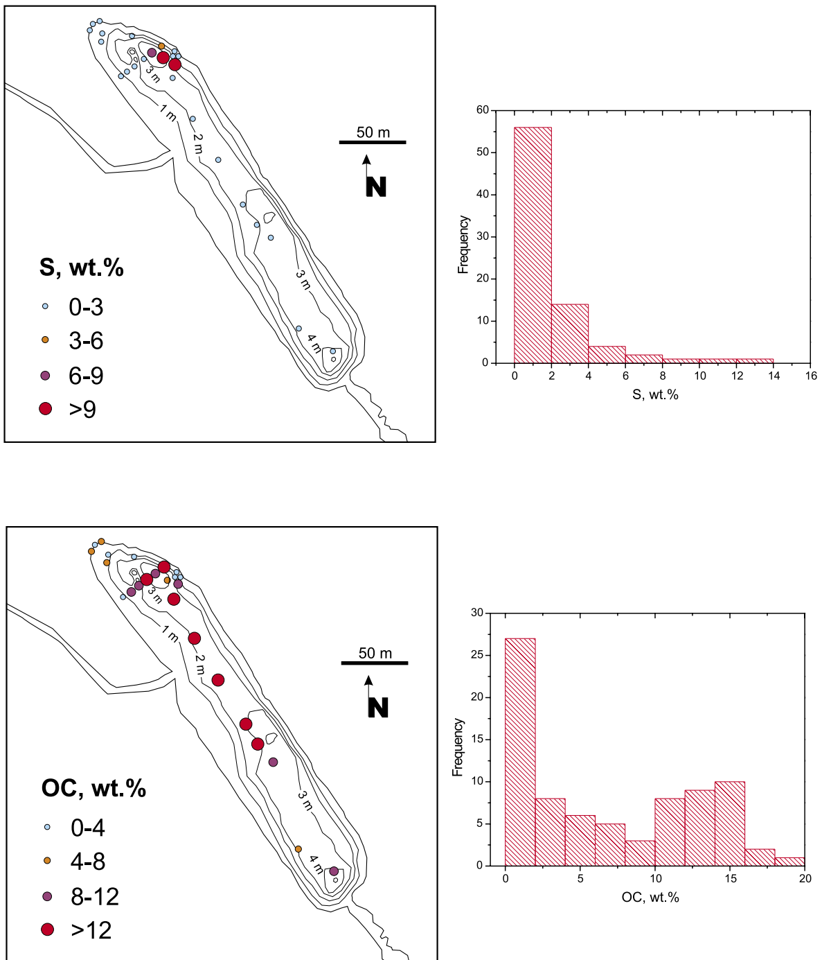
Figure 19 The distribution of sulfur (S) and organic carbon (OC) in sediments collected from the HBHA Pond. The aerial distributions of sulfur and organic carbon are based on grab samples and the top 2-cm interval of core samples; contour lines delineate depth to sediment (meters). The frequency plot includes all grab samples and all sediment core depth intervals; data are compiled in Appendix B.
