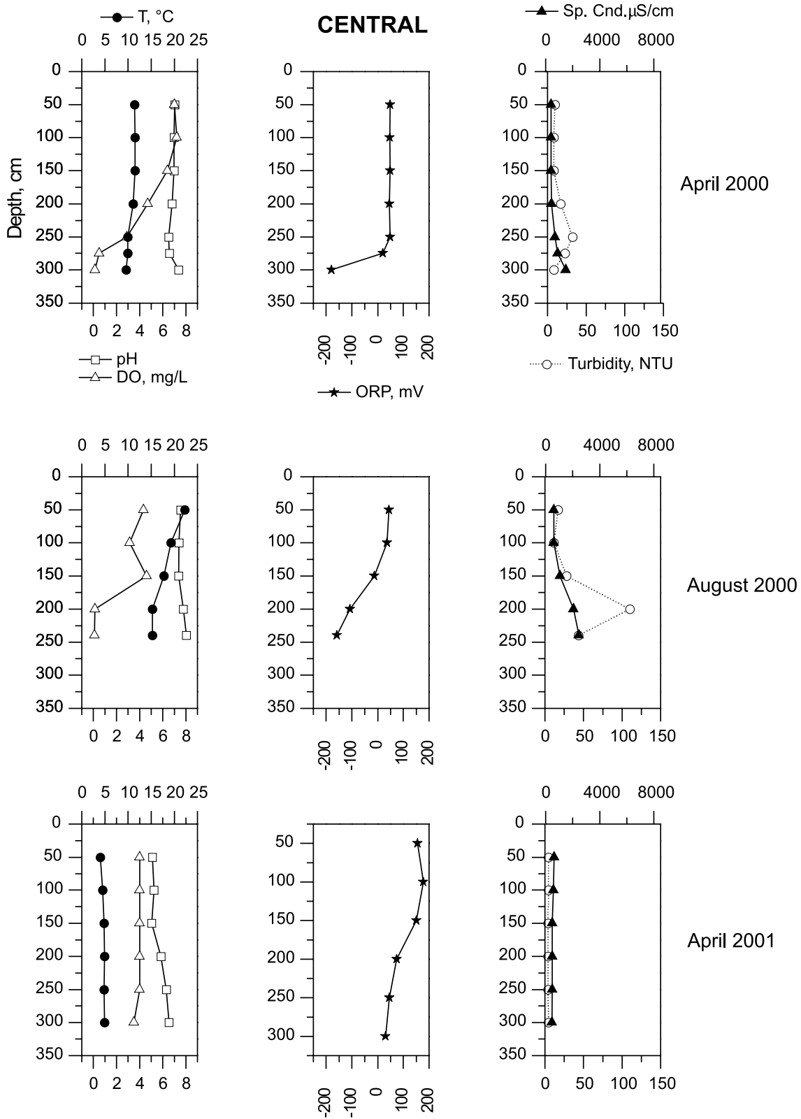
Figure 10 Vertical patterns in water quality within the central part of the HBHA Pond on sampling dates in April 2000, August 2000, and April 2001. Symbols: T = temperature, DO = dissolved oxygen, ORP = oxidation-reduction potential, and Sp. Cnd. = specific conductance.
