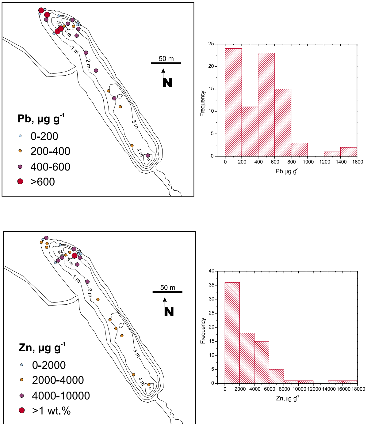
Figure 17 The distribution of lead (Pb) and zinc (Zn) in sediments collected from the HBHA Pond. The aerial distributions of lead and zinc are based on grab samples and the top 2-cm interval of core samples; contour lines delineate depth to sediment (meters). The frequency plot includes all grab samples and all sediment core depth intervals; data are compiled in Appendix B.
