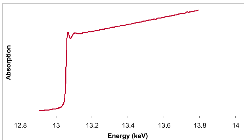
Figure C.10 Raw fluorescence data Pb sorption on ferrihydrite
