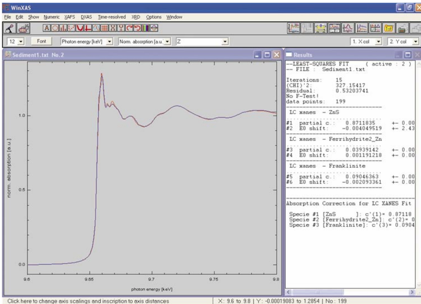
Figure C.20 Linear combination fitting of X-ray absorption near edge spectroscopy data (LCF-XANES) for a sediment (Sediment1) sample with multiple Zn species. The red curve is the sample data, and the blue curve is the fitted result. The LCF-XANES results indicate Zn speciation as 87% ZnS, 4% Zn sorbed to ferrihydrite, and 9% \text{ZnFe}_2\text{O}_4 (franklinite).
