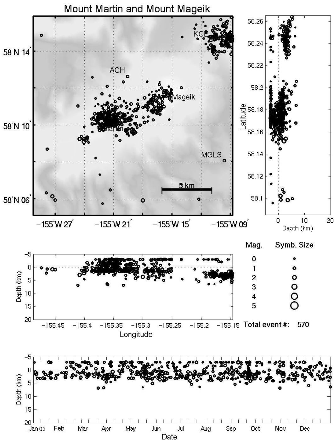
Figure A11. Summary plots of 570 earthquakes located near Mount Mageik and Mount Martin in the Katmai volcanic group in 2002. Open circles scaled with magnitude show hypocenter locations shallower than 20 km. Hypocenters with depths of 20 km and deeper are shown by open triangles scaled with magnitude. Seismic stations are shown by open squares and labeled by station code. (See Appendix B for station information). Closed circles are used to show other points of interest.
