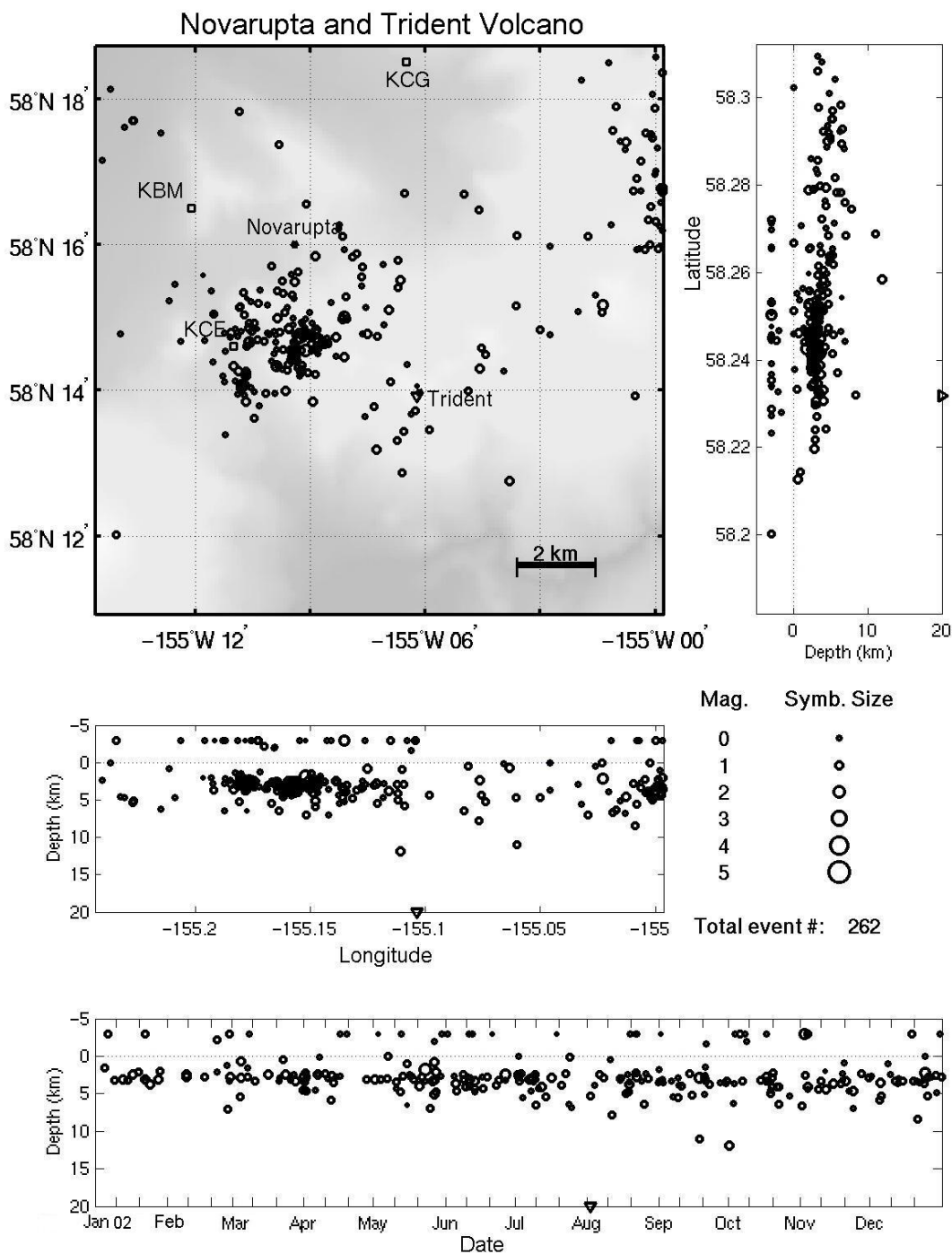
Figure A10. Summary plots of 262 earthquakes located near Novarupta and Trident Volcano in the Katmai volcanic group in 2002. Open circles scaled with magnitude show hypocenter locations shallower than 20 km. Hypocenters with depths of 20 km and deeper are shown by open triangles scaled with magnitude. Seismic stations are shown by open squares and labeled by station code. (See Appendix B for station information). Closed circles are used to show other points of interest.
