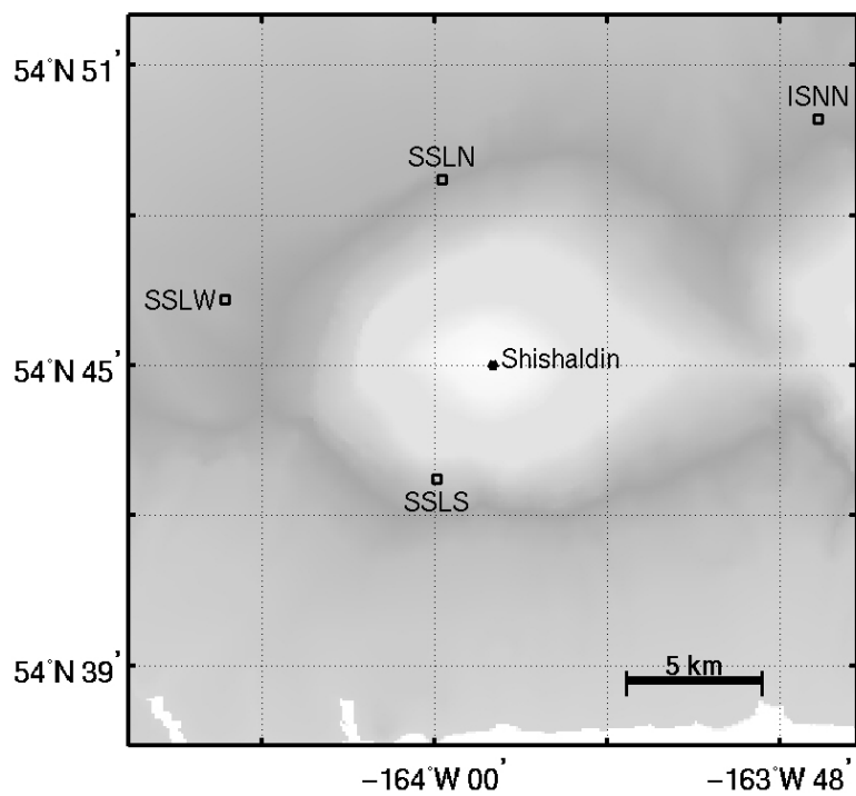
Figure C14. AVO seismic stations near Shishaldin Volcano.
