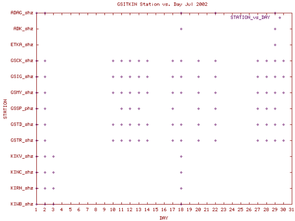
Station Use Plot for the Great Sitkin subnetwork for July 2002
