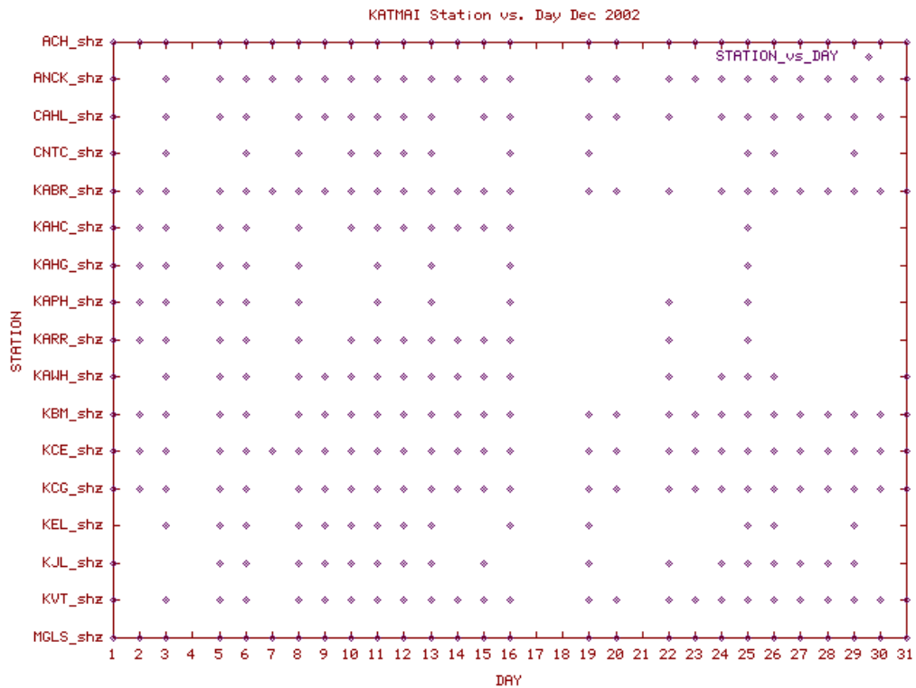
Station Use Plot for the Katmai volcanic group subnetwork for December 2002
