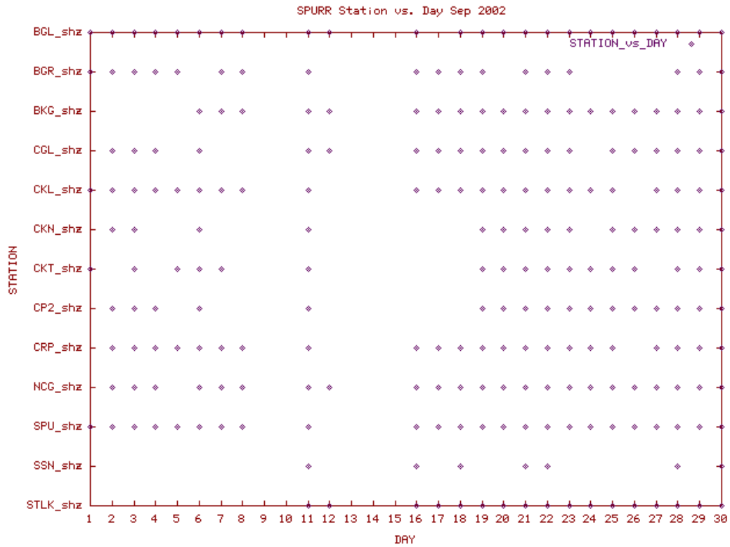
Station Use Plot for the Spurr subnetwork for September 2002
