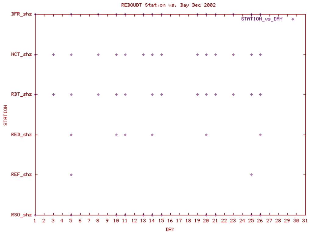
Station Use Plot for the Redoubt subnetwork for December 2002
