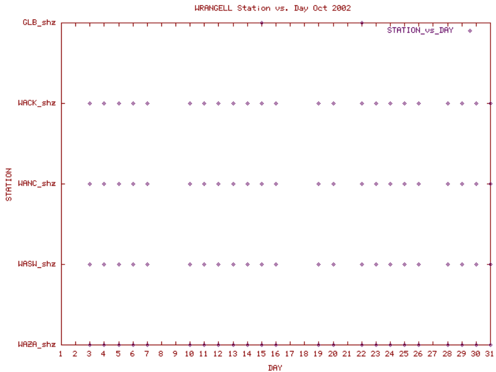
Station Use Plot for the Wrangell subnetwork for October 2002
