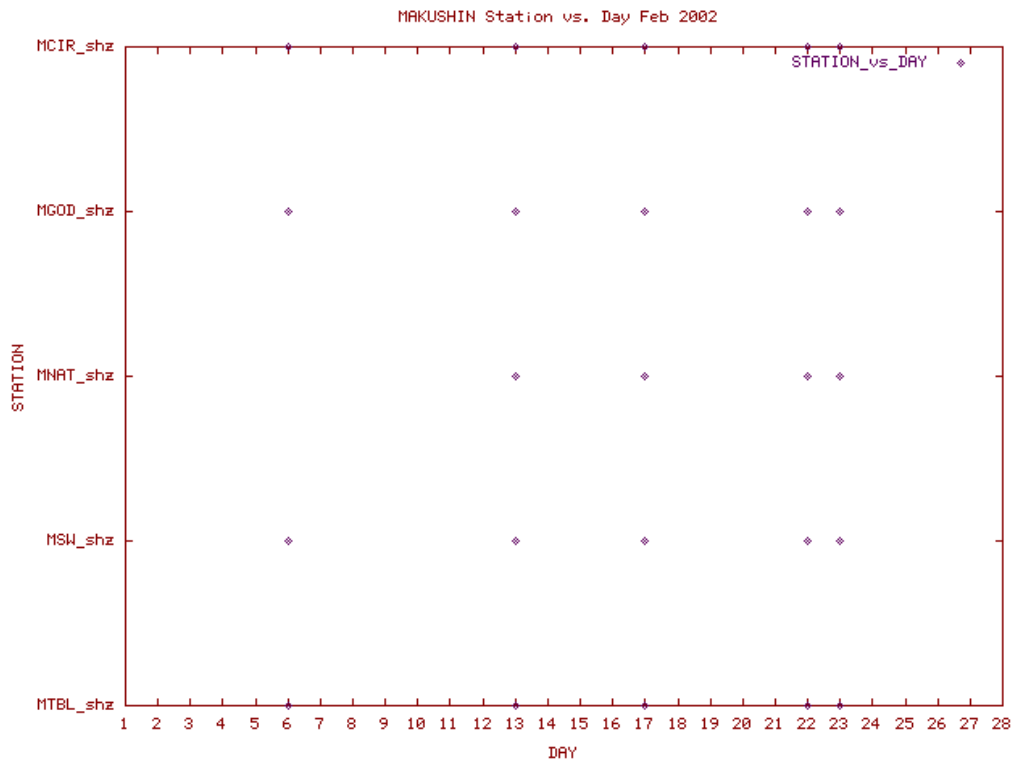
Station Use Plot for the Makushin subnetwork for February 2002
