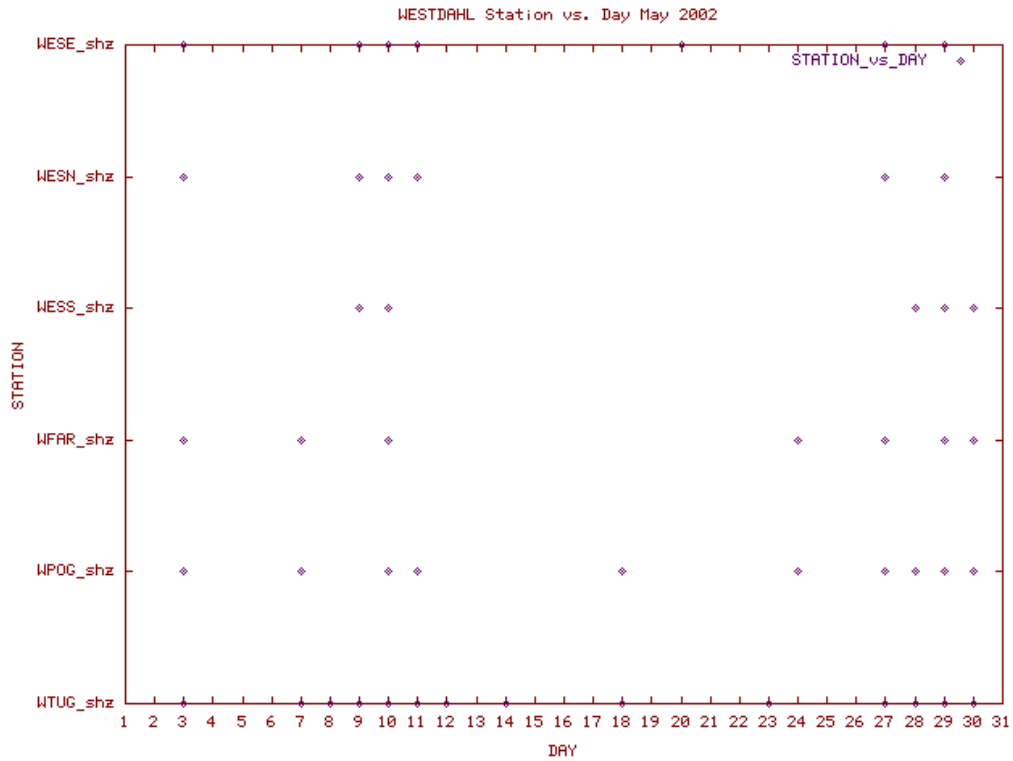
Station Use Plot for the Westdahl subnetwork for May 2002
