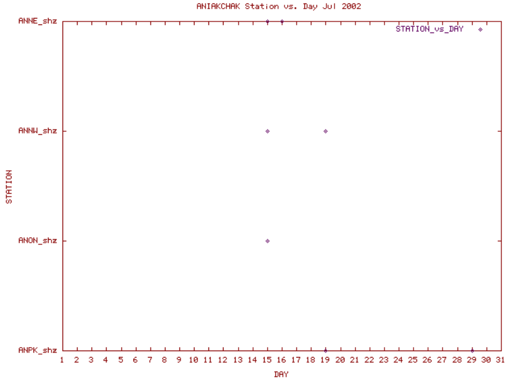
Station Use Plot for the Aniakchak subnetwork for July 2002
