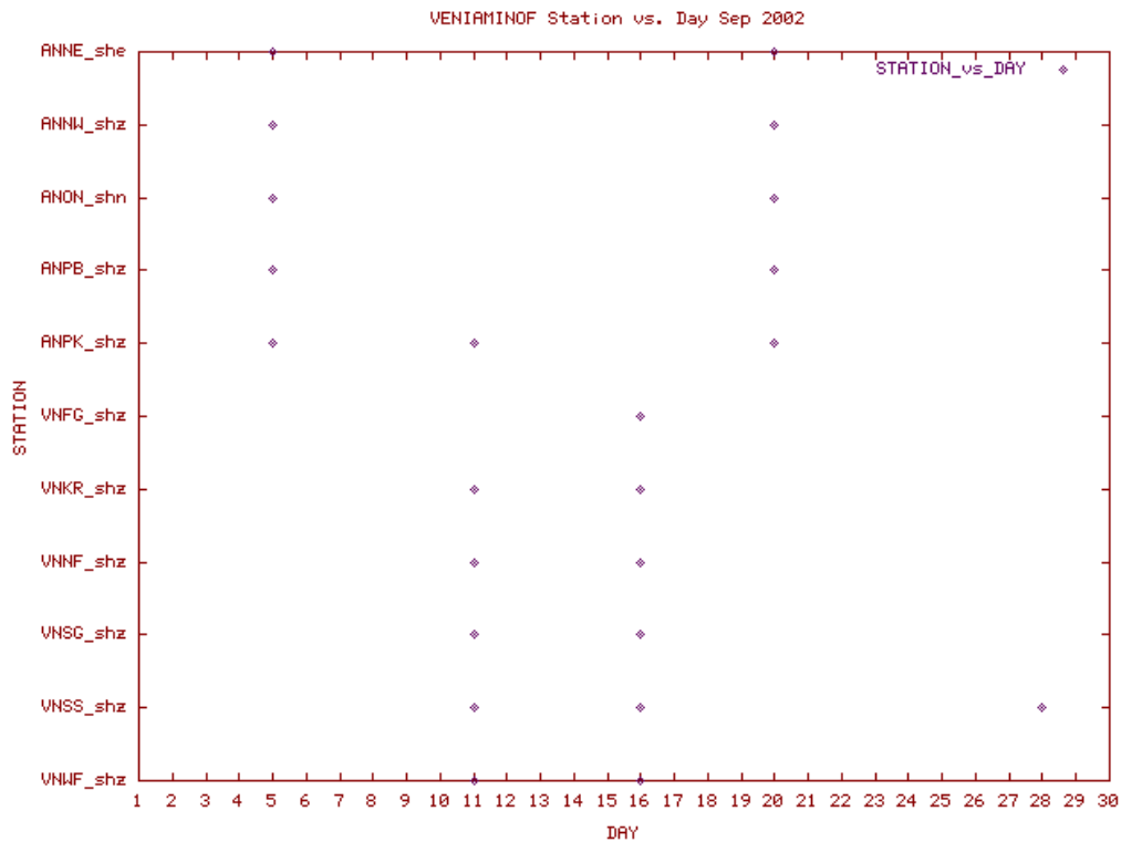
Station Use Plot for the Veniaminof subnetwork for September 2002
