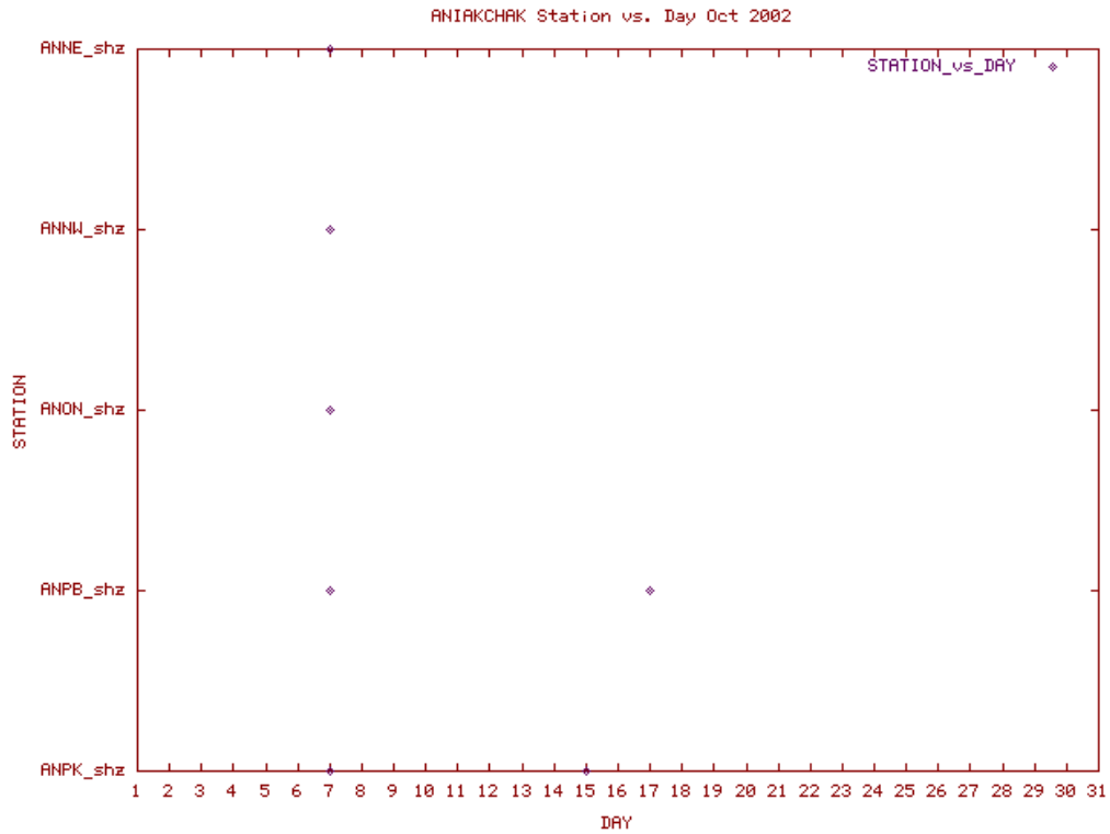
Station Use Plot for the Aniakchak subnetwork for October 2002
