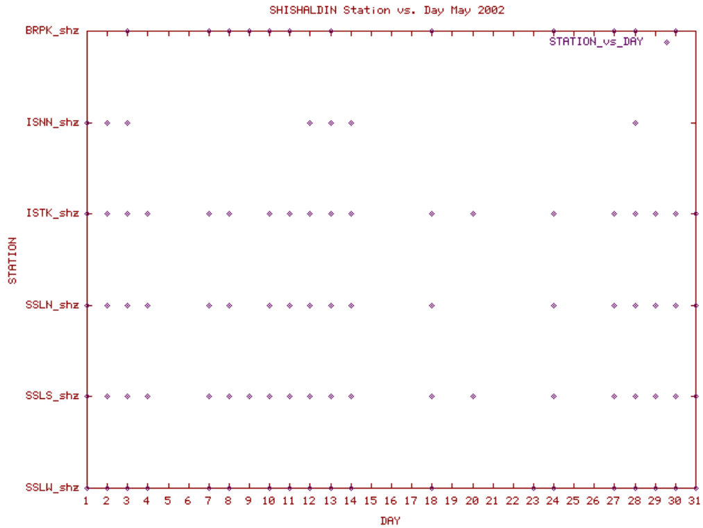
Station Use Plot for the Shishaldin subnetwork for May 2002
