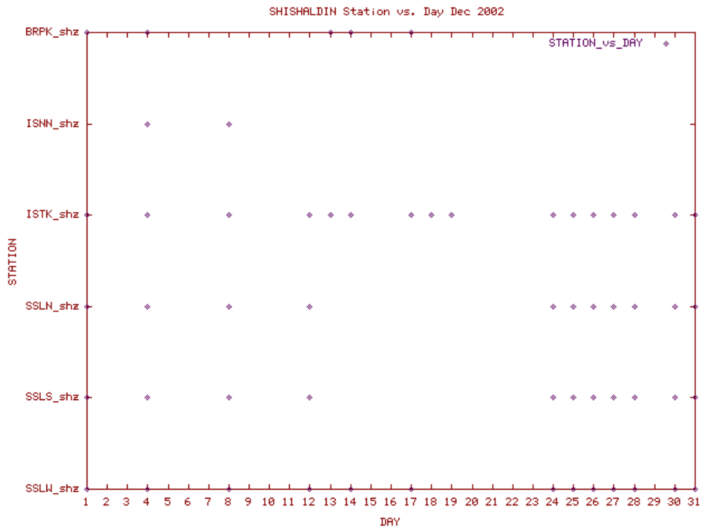
Station Use Plot for the Shishaldin subnetwork for December 2002
