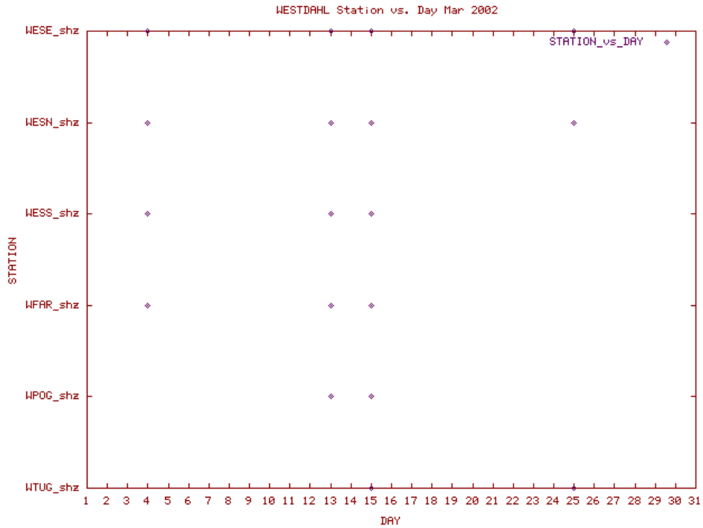
Station Use Plot for the Westdahl subnetwork for March 2002
