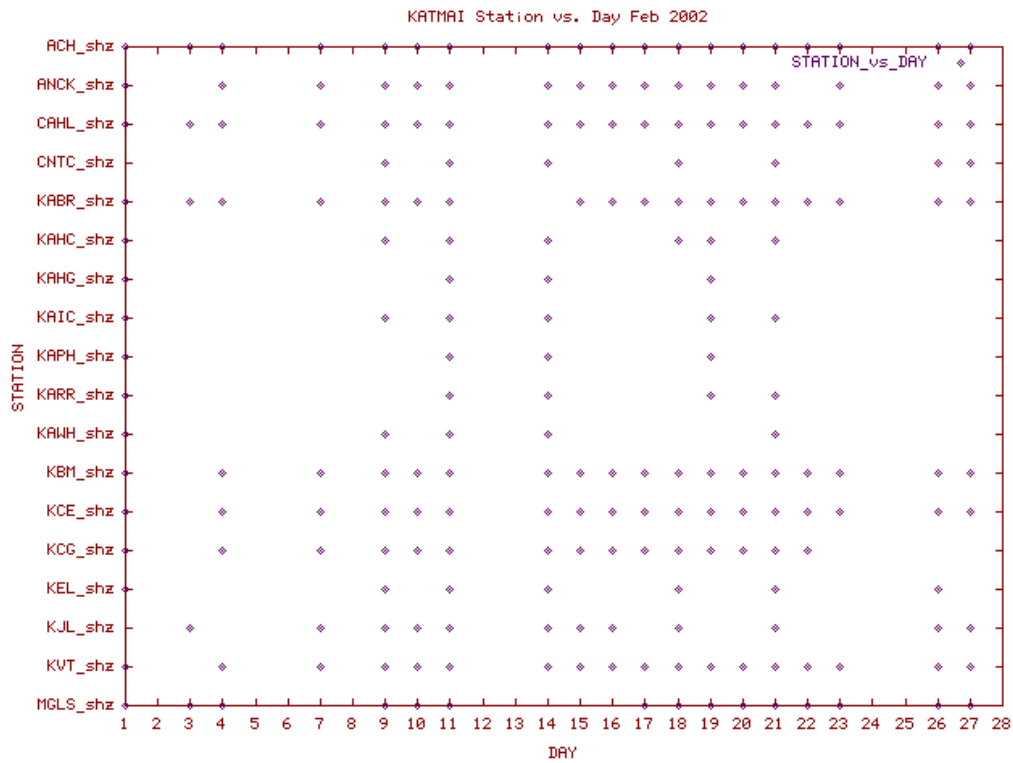
Station Use Plot for the Katmai volcanic group subnetwork for February 2002
