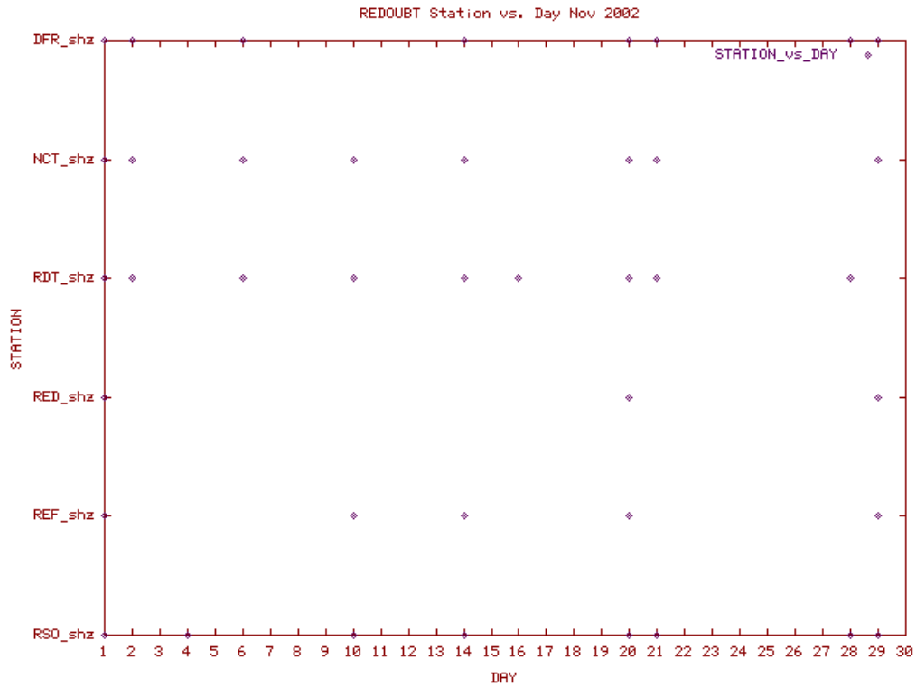
Station Use Plot for the Redoubt subnetwork for November 2002
