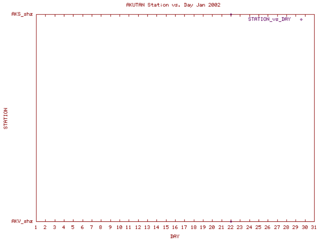
Station Use Plot for the Akutan subnetwork for January 2002
