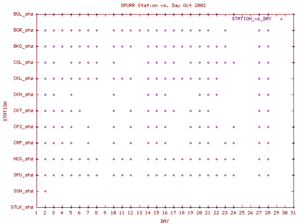
Station Use Plot for the Spurr subnetwork for October 2002
