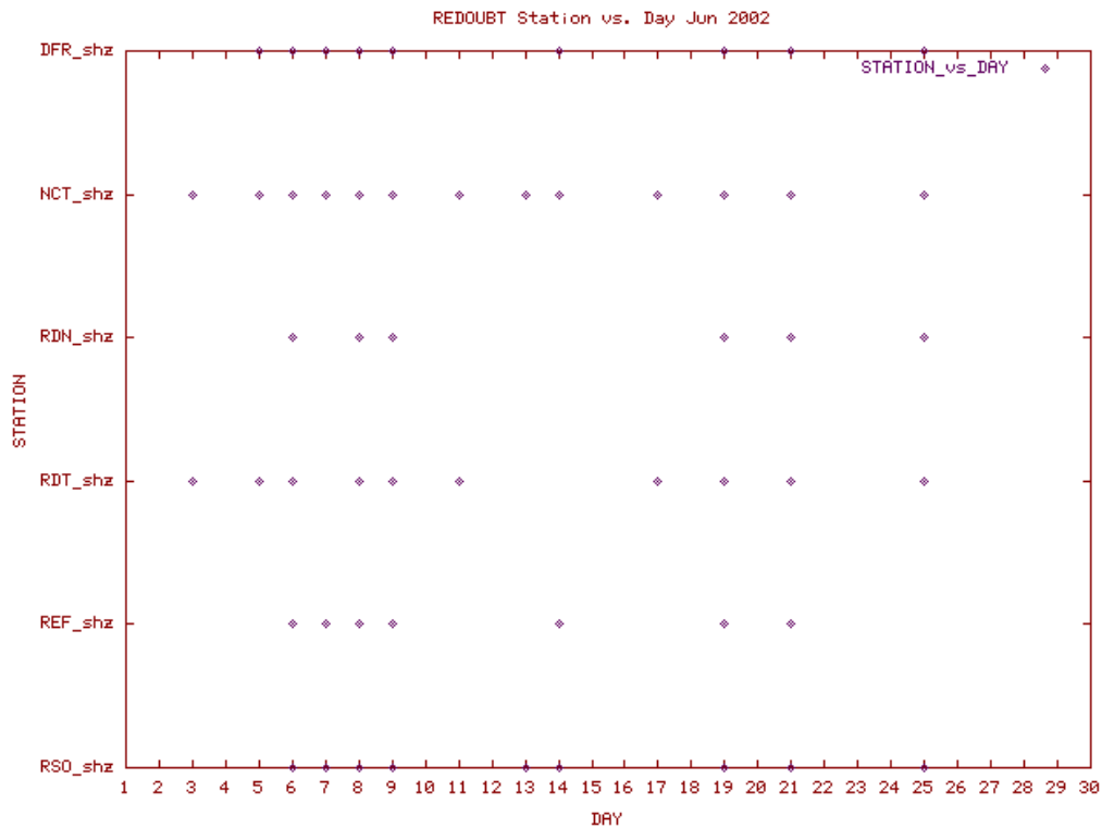
Station Use Plot for the Redoubt subnetwork for June 2002
