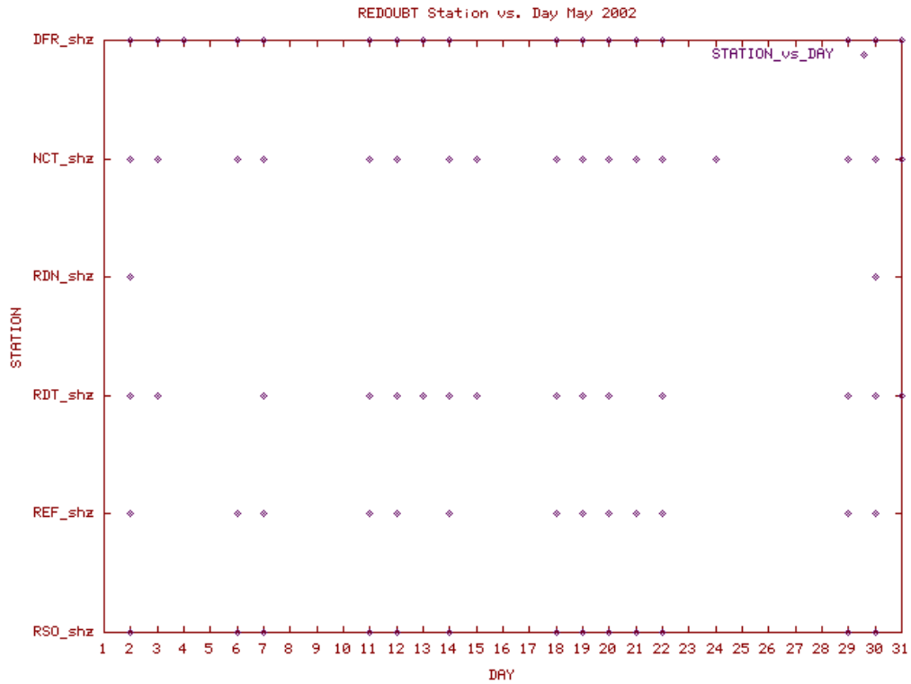
Station Use Plot for the Redoubt subnetwork for May 2002
