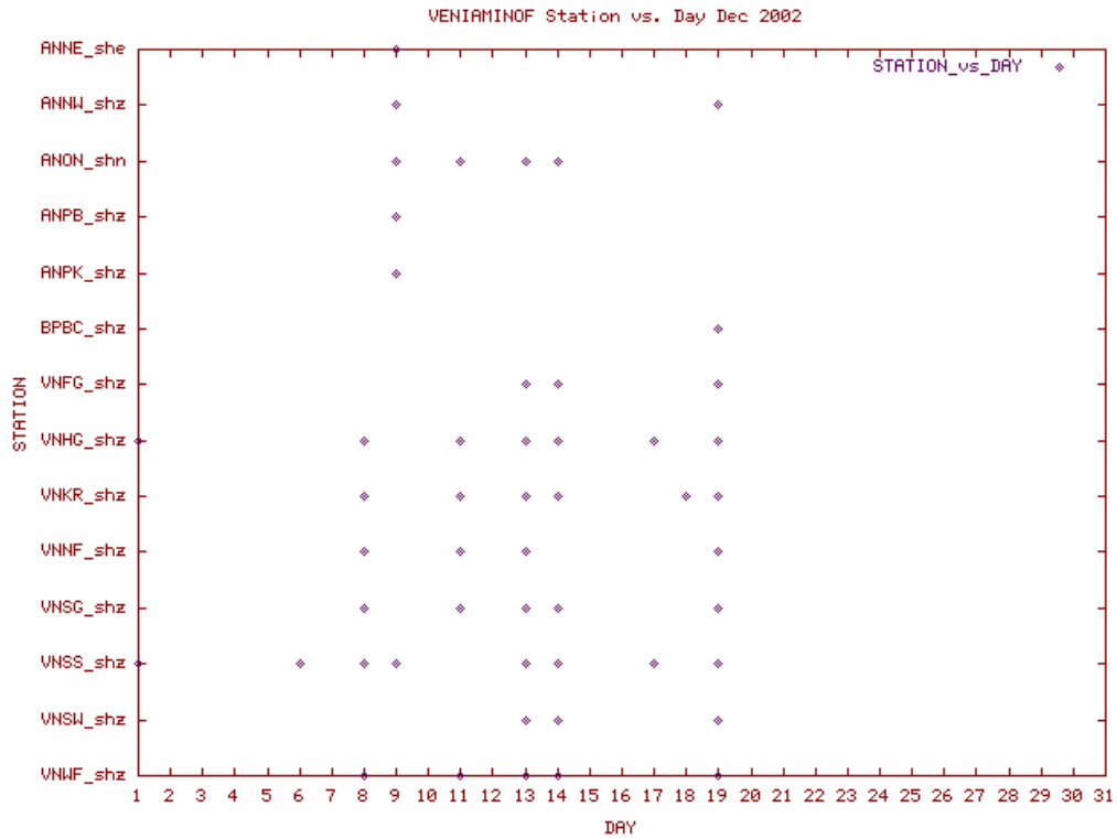
Station Use Plot for the Veniaminof subnetwork for December 2002
