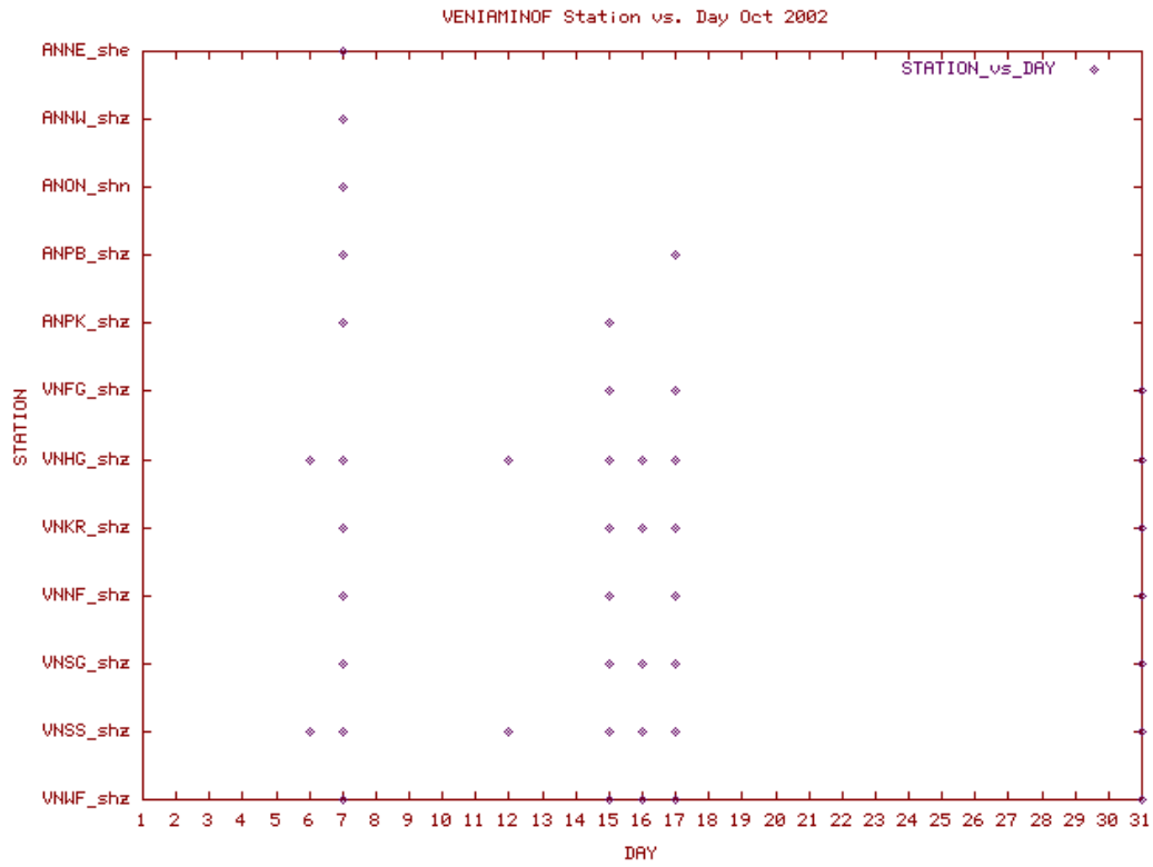
Station Use Plot for the Veniaminof subnetwork for October 2002
