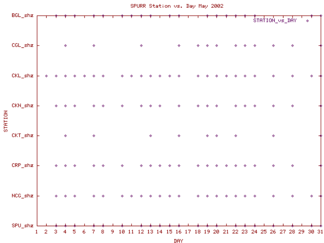
Station Use Plot for the Spurr subnetwork for May 2002
