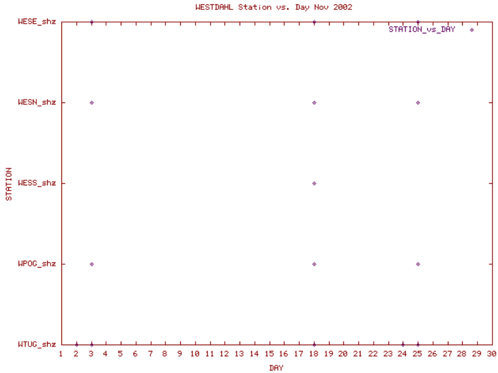
Station Use Plot for the Westdahl subnetwork for November 2002
