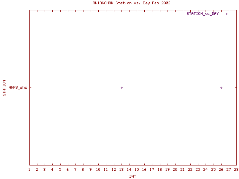
Station Use Plot for the Aniakchak subnetwork for February 2002
