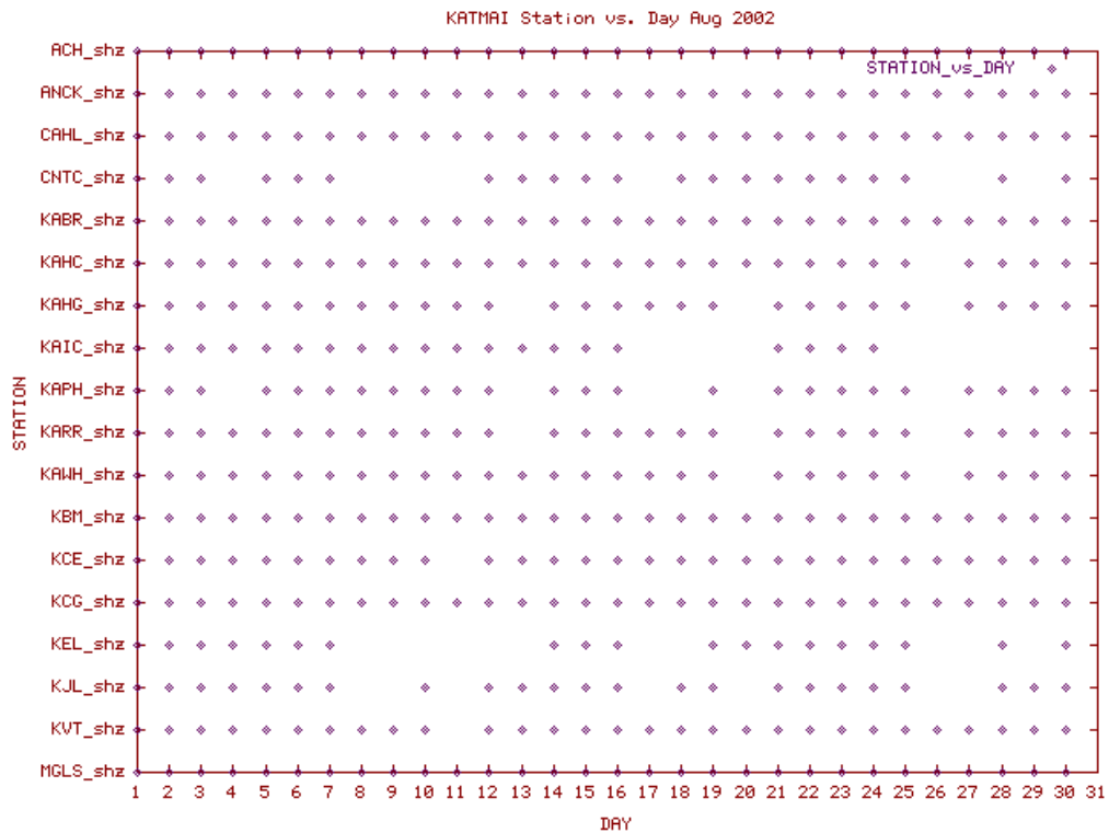
Station Use Plot for the Katmai volcanic group subnetwork for August 2002
