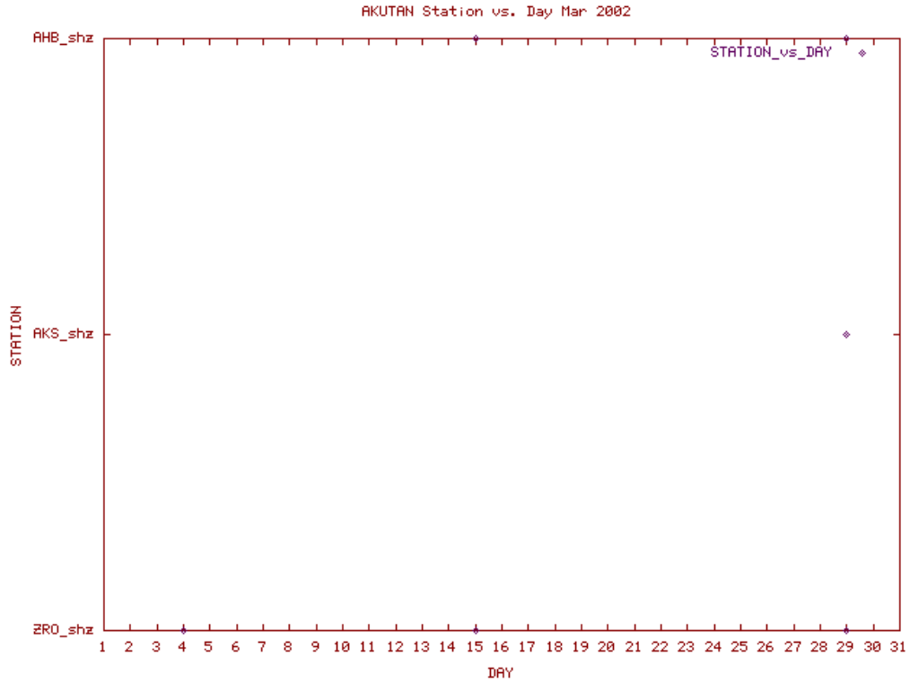
Station Use Plot for the Akutan subnetwork for March 2002
