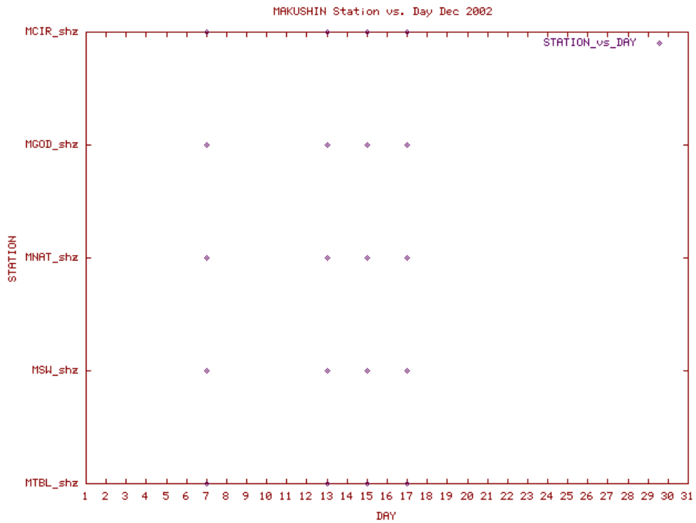
Station Use Plot for the Makushin subnetwork for December 2002
