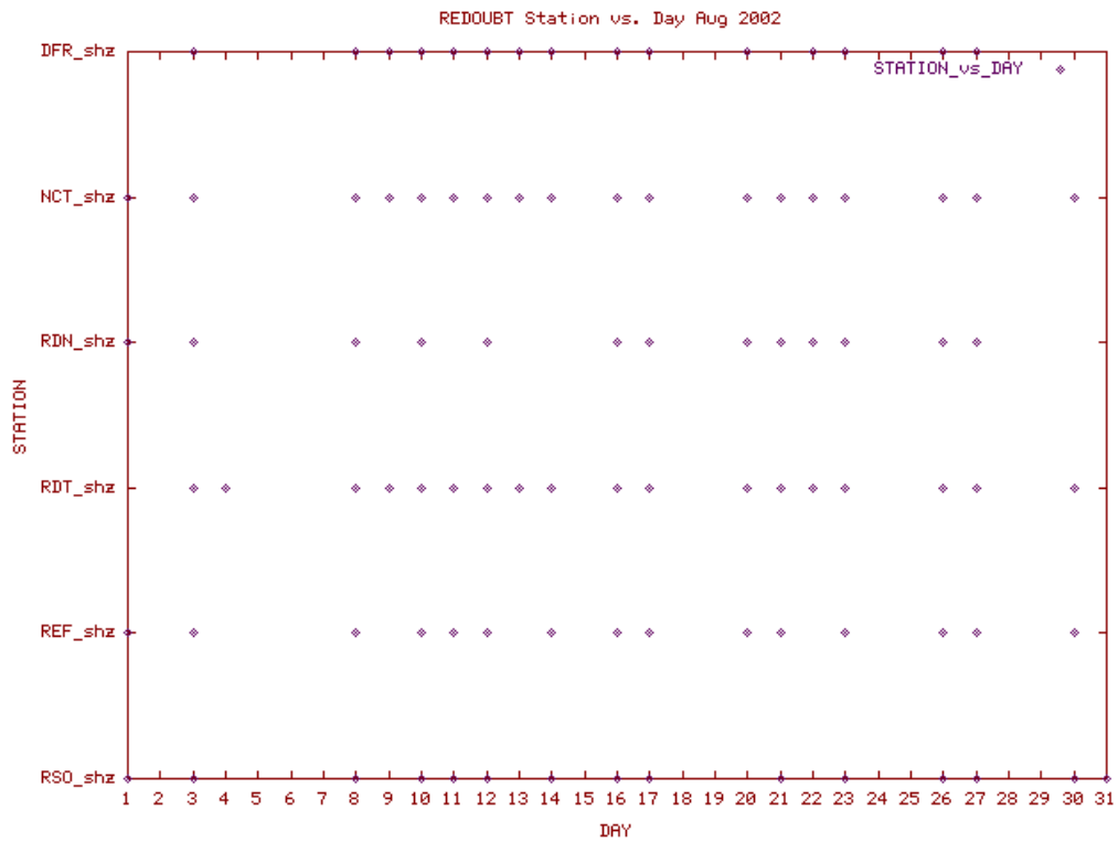
Station Use Plot for the Redoubt subnetwork for August 2002
