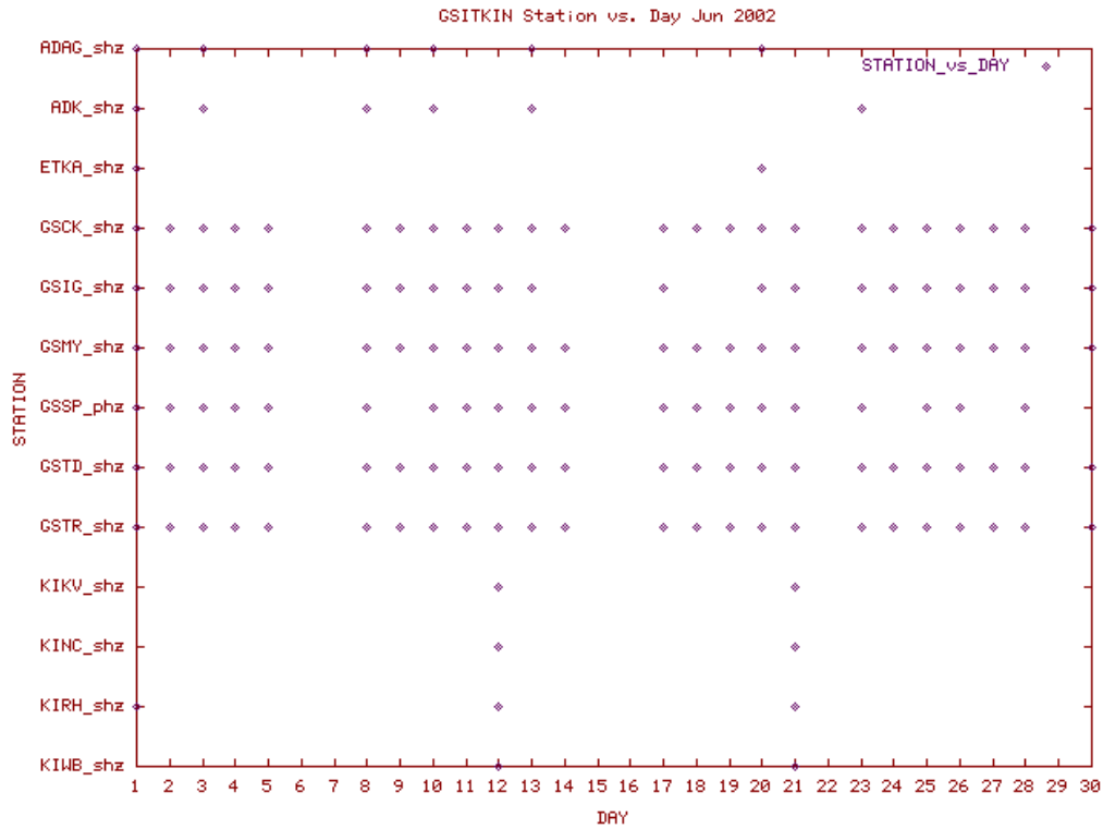
Station Use Plot for the Great Sitkin subnetwork for June 2002
