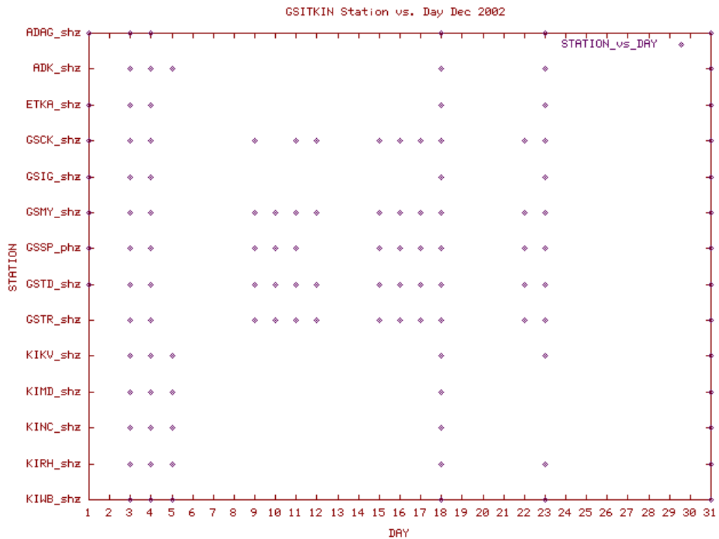
Station Use Plot for the Great Sitkin subnetwork for December 2002
