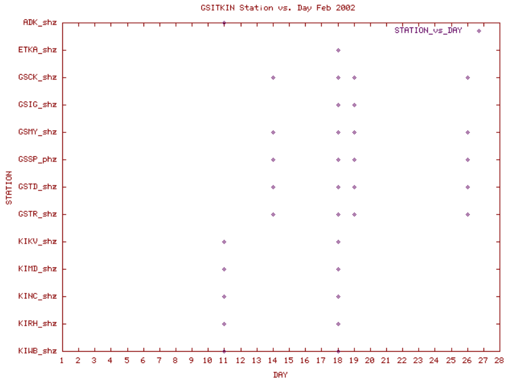
Station Use Plot for the Great Sitkin subnetwork for February 2002
