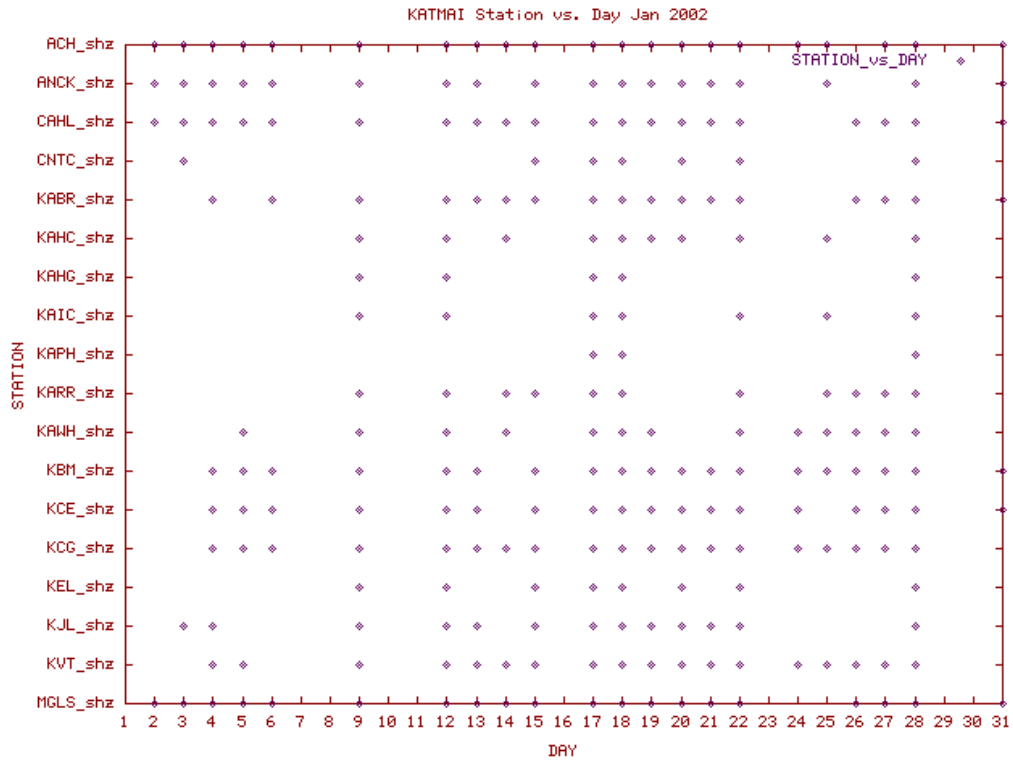
Station Use Plot for the Katmai volcanic group subnetwork for January 2002
