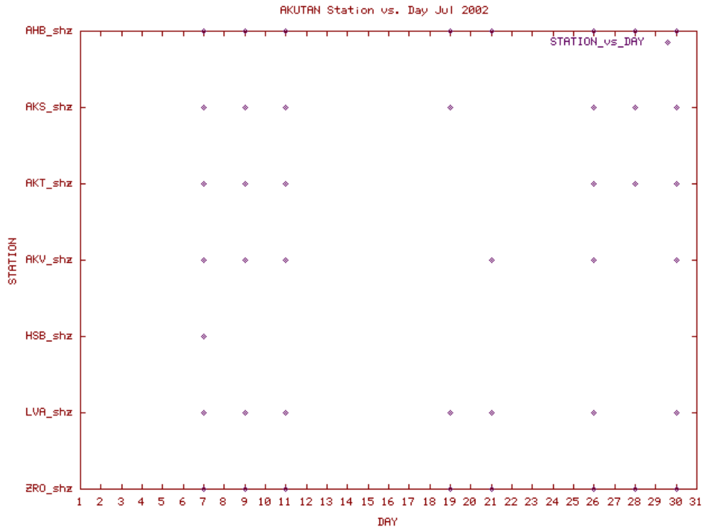
Station Use Plot for the Akutan subnetwork for July 2002
