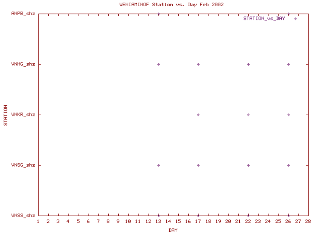
Station Use Plot for the Veniaminof subnetwork for February 2002
