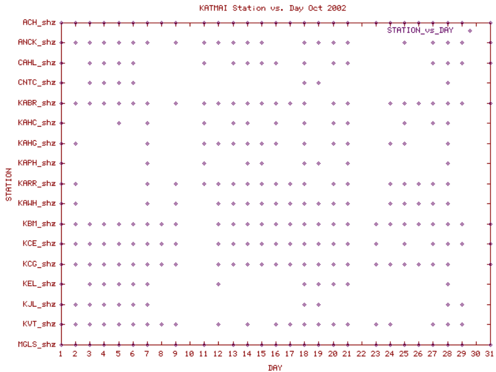
Station Use Plot for the Katmai volcanic group subnetwork for October 2002
