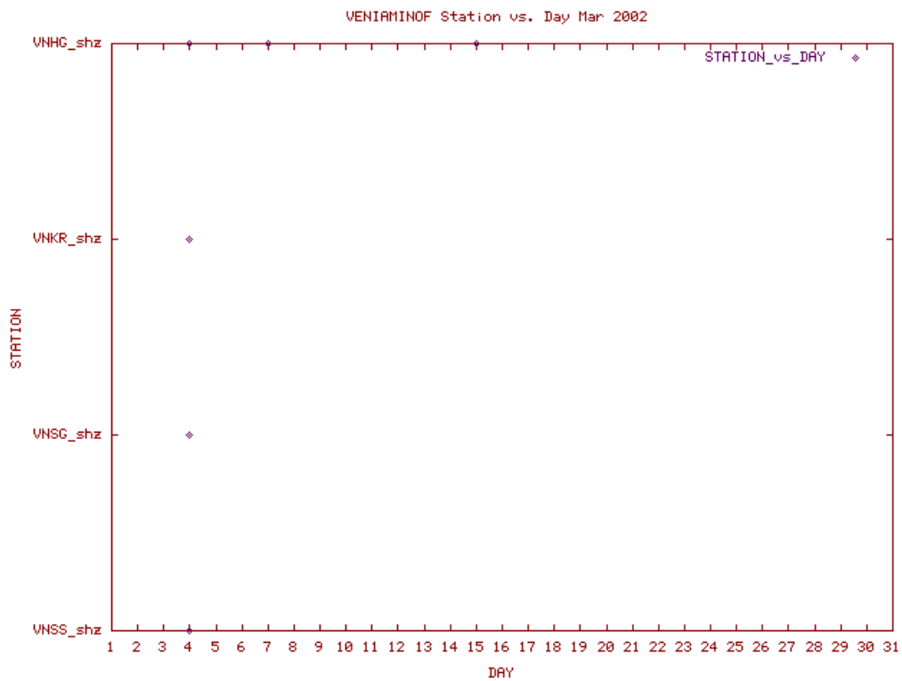
Station Use Plot for the Veniaminof subnetwork for March 2002
