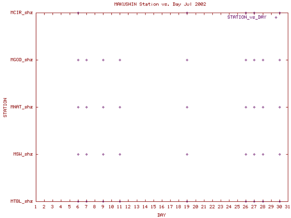
Station Use Plot for the Makushin subnetwork for July 2002
