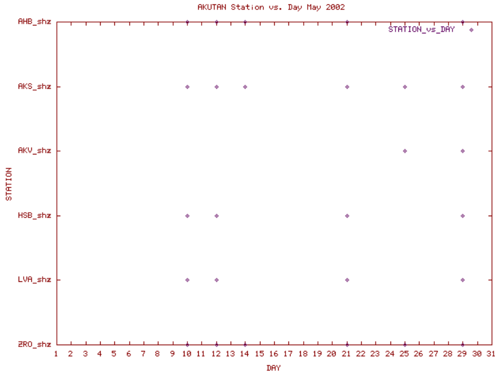
Station Use Plot for the Akutan subnetwork for May 2002
