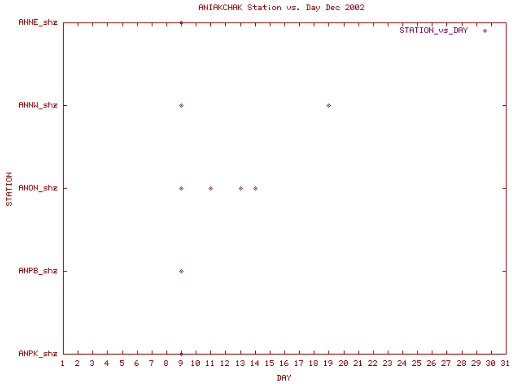
Station Use Plot for the Aniakchak subnetwork for December 2002
