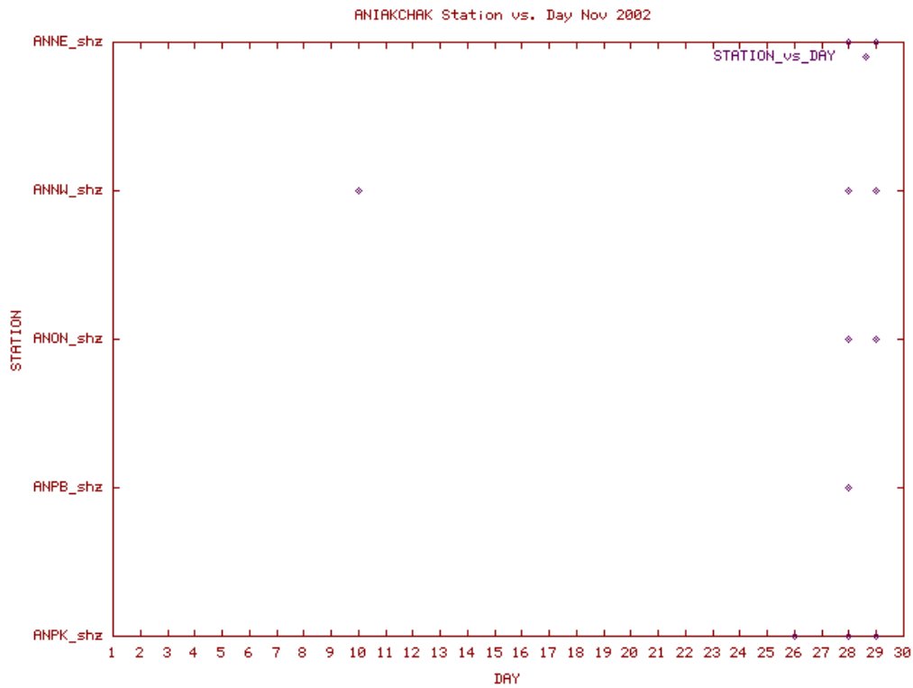
Station Use Plot for the Aniakchak subnetwork for November 2002
