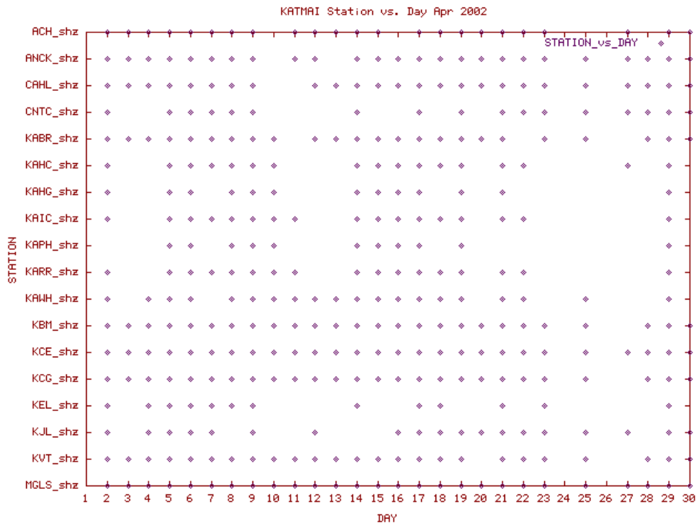
Station Use Plot for the Katmai volcanic group subnetwork for April 2002
