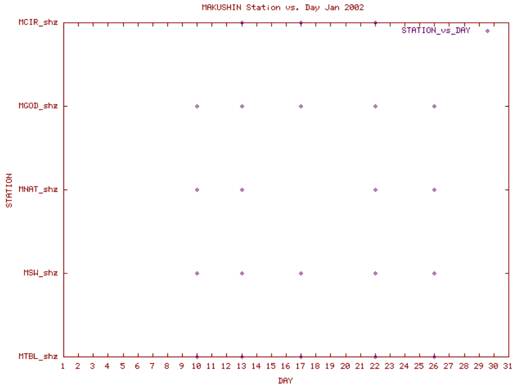
Station Use Plot for the Makushin subnetwork for January 2002
