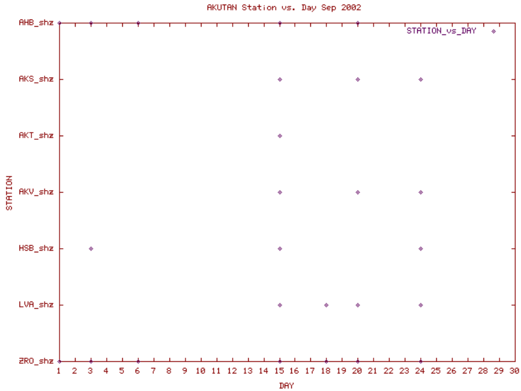
Station Use Plot for the Akutan subnetwork for September 2002
