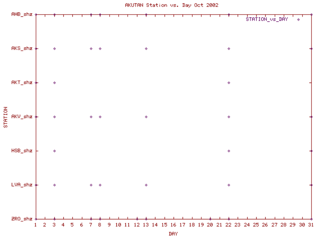
Station Use Plot for the Akutan subnetwork for October 2002
