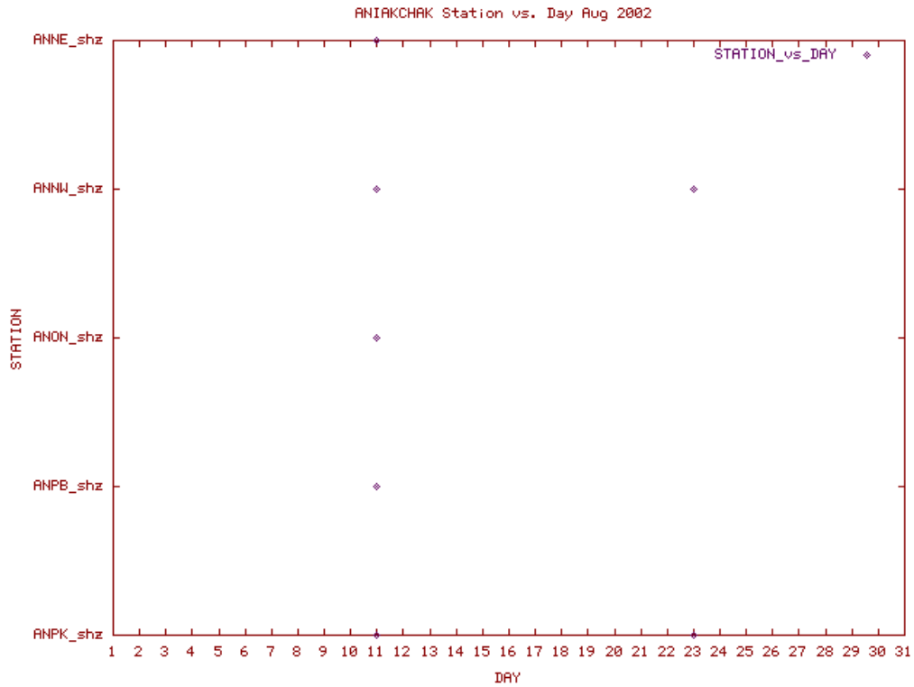
Station Use Plot for the Aniakchak subnetwork for August 2002
