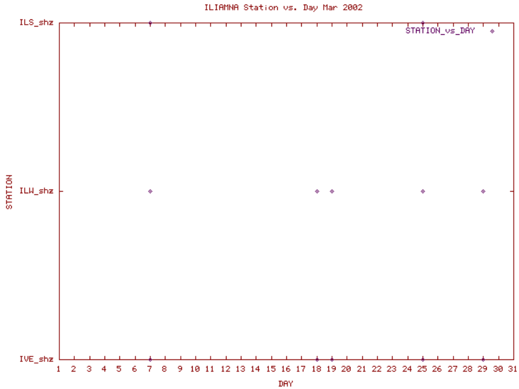
Station Use Plot for the Iliamna subnetwork for March 2002
