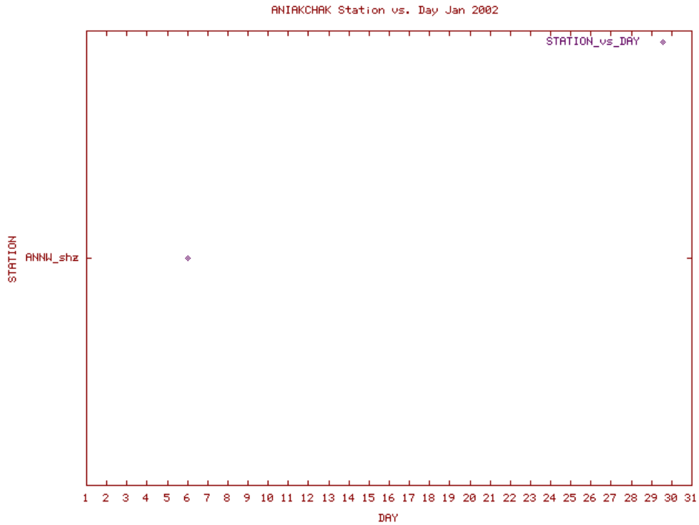
Station Use Plot for the Aniakchak subnetwork for January 2002
