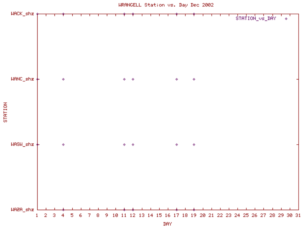
Station Use Plot for the Wrangell subnetwork for December 2002
