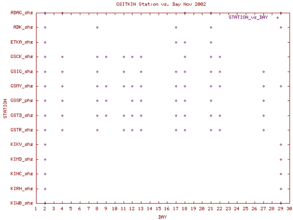
Station Use Plot for the Great Sitkin subnetwork for November 2002
