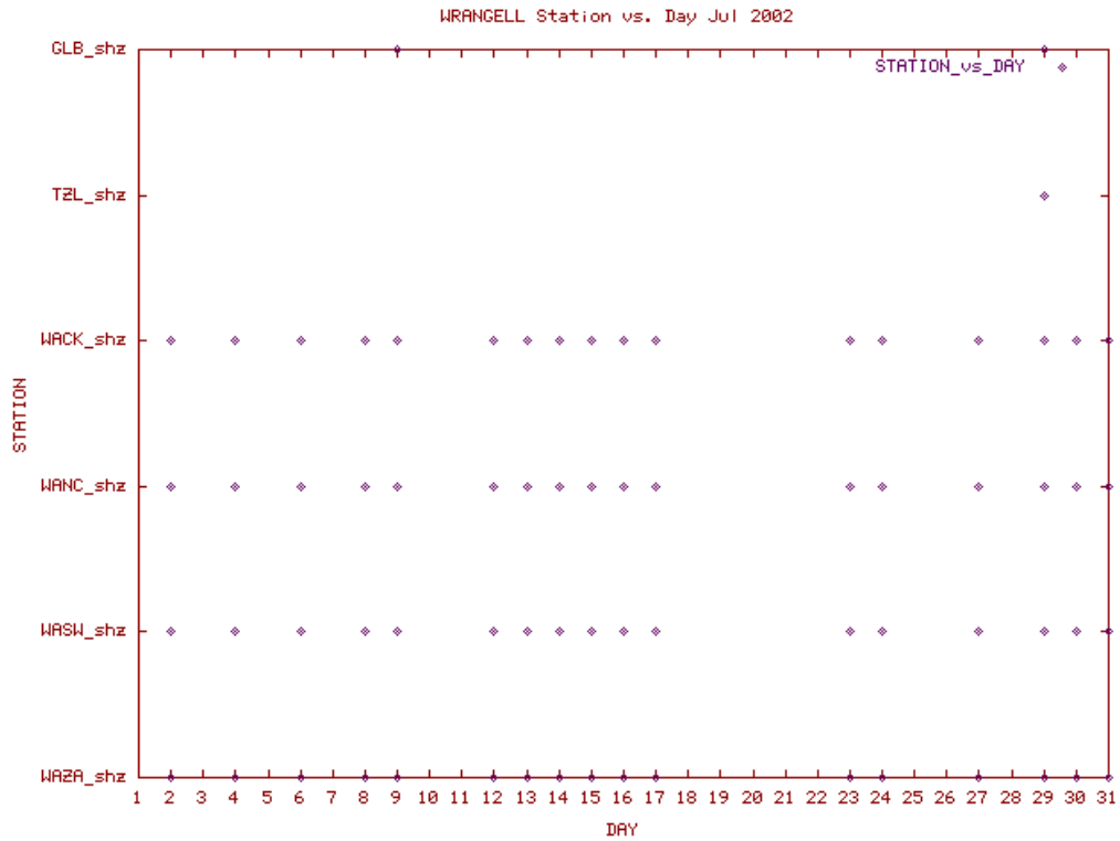
Station Use Plot for the Wrangell subnetwork for July 2002
