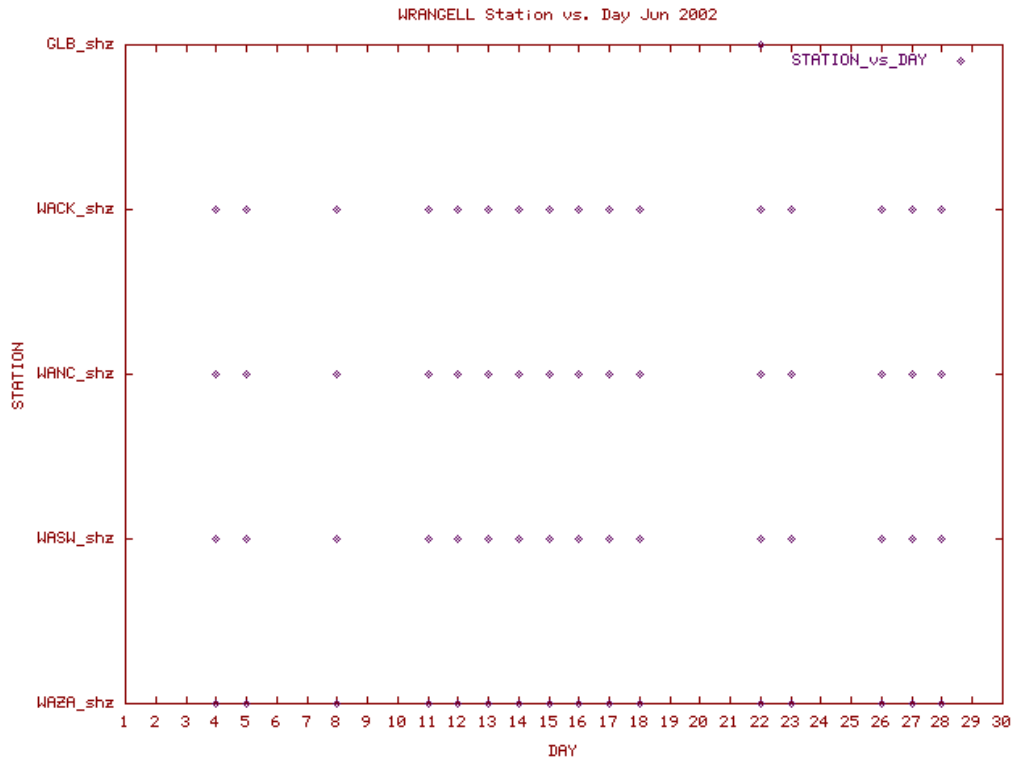
Station Use Plot for the Wrangell subnetwork for June 2002
