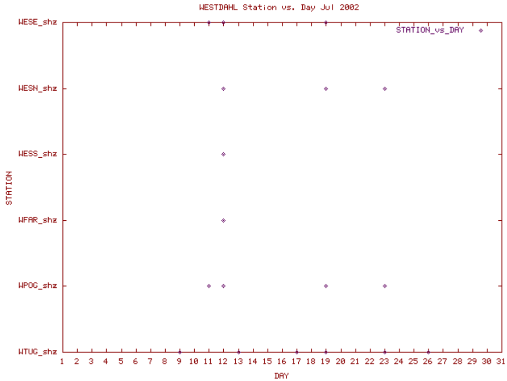
Station Use Plot for the Westdahl subnetwork for July 2002
