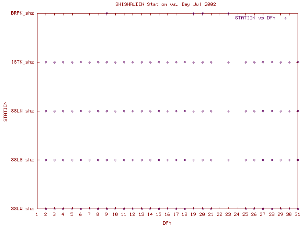
Station Use Plot for the Shishaldin subnetwork for July 2002
