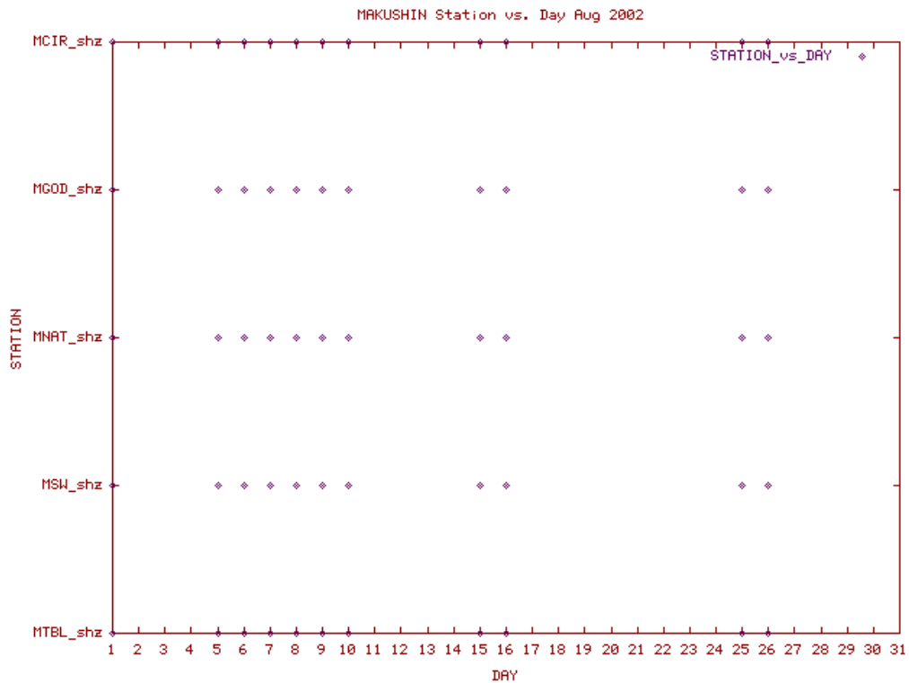
Station Use Plot for the Makushin subnetwork for August 2002
