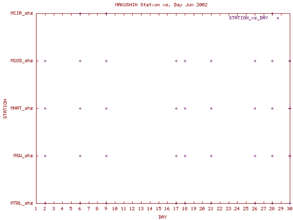
Station Use Plot for the Makushin subnetwork for Jun 2000
