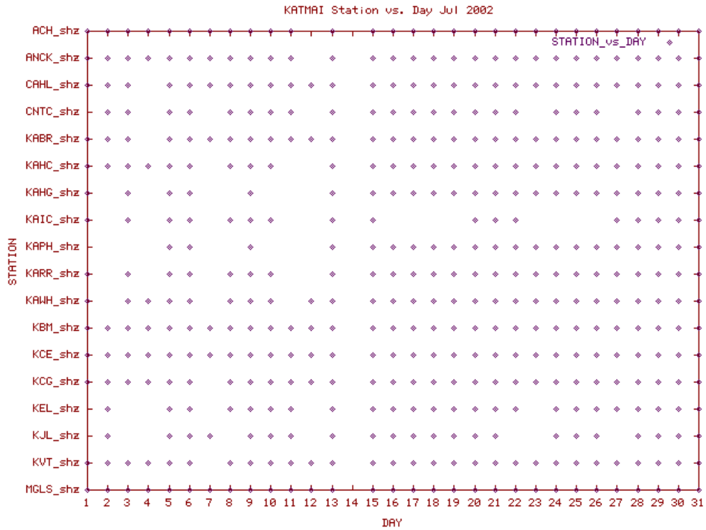
Station Use Plot for the Katmai volcanic group subnetwork for July 2002
