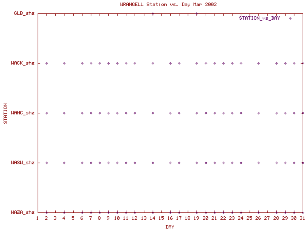
Station Use Plot for the Wrangell subnetwork for March 2002
