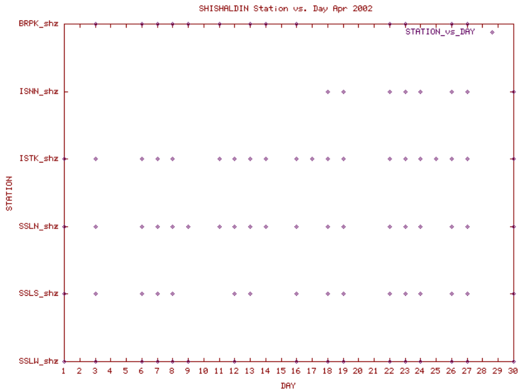
Station Use Plot for the Shishaldin subnetwork for April 2002
