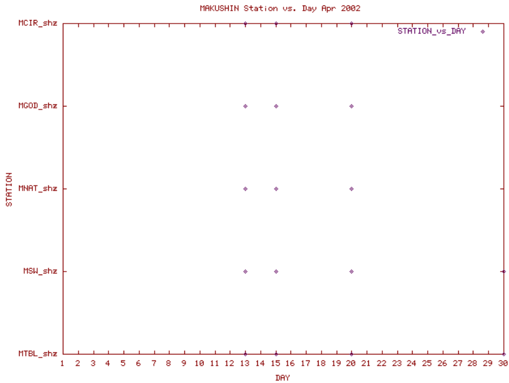
Station Use Plot for the Makushin subnetwork for April 2002
