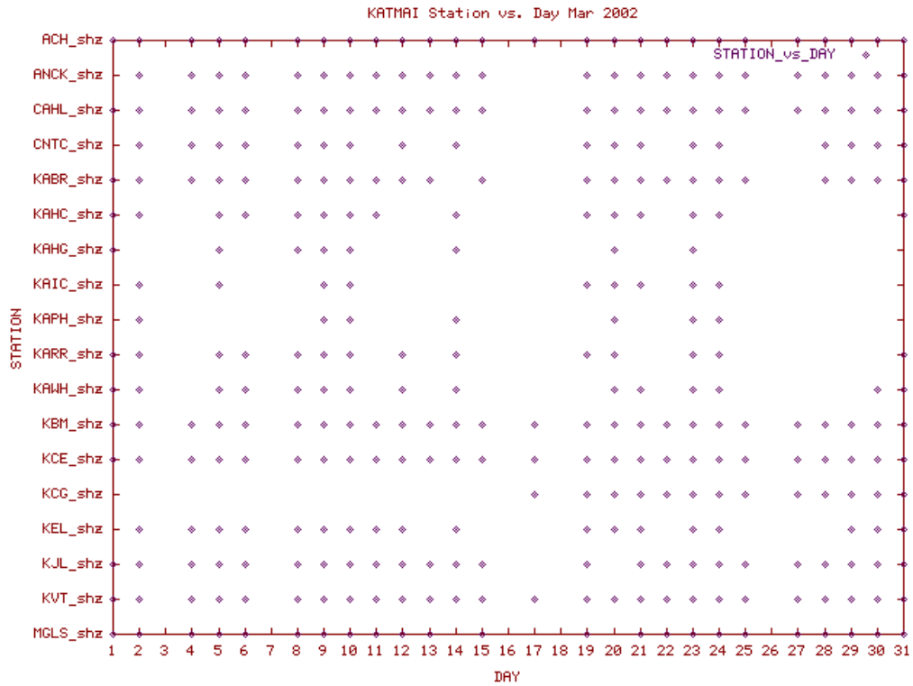
Station Use Plot for the Katmai volcanic group subnetwork for March 2002
