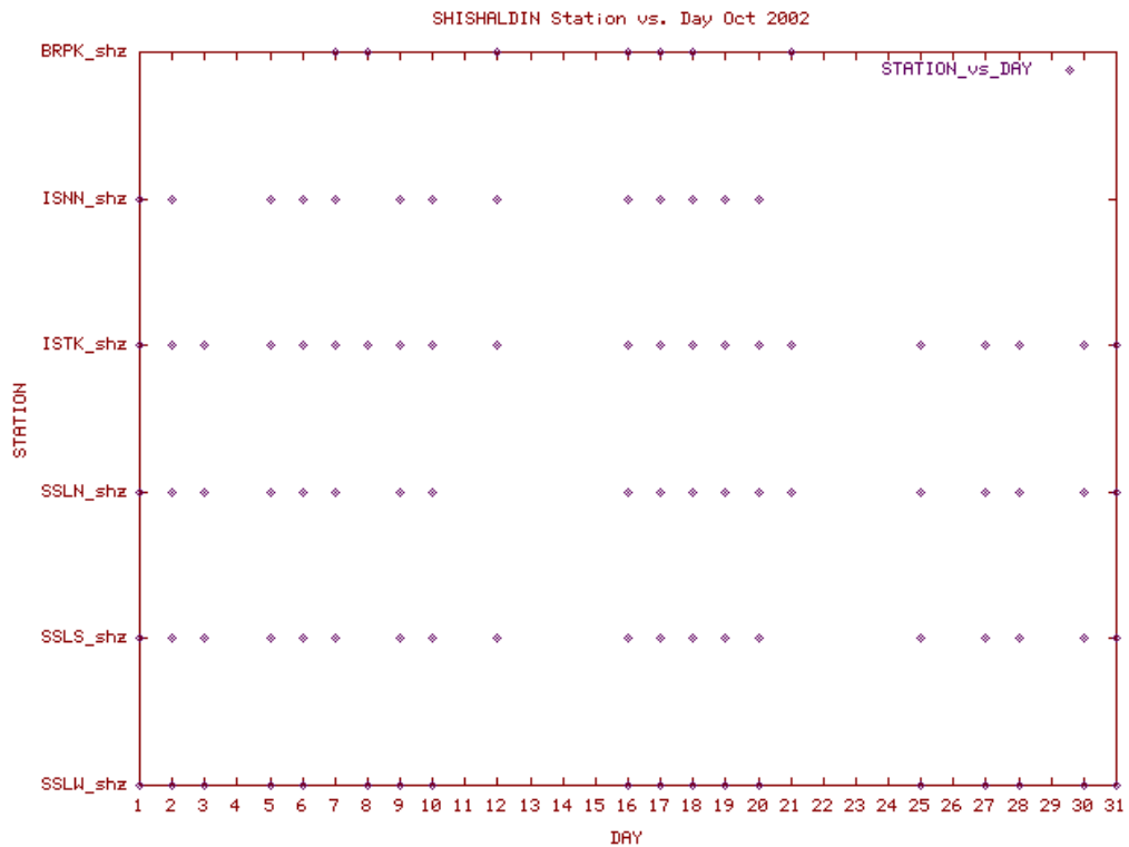
Station Use Plot for the Shishaldin subnetwork for October 2002
