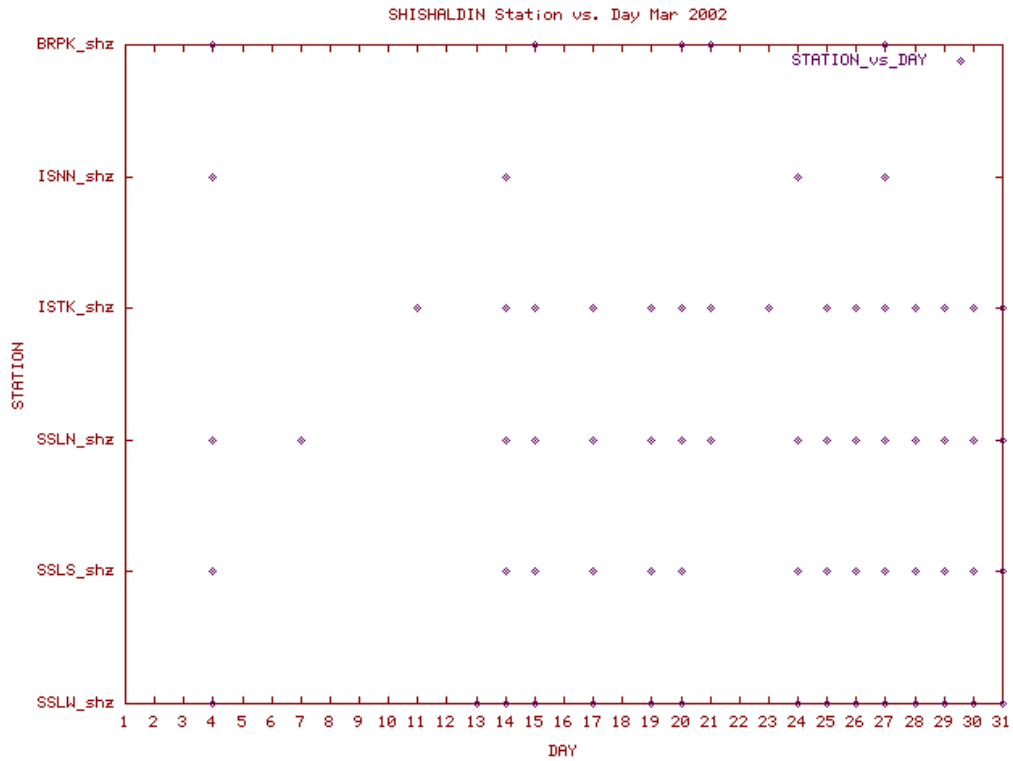
Station Use Plot for the Shishaldin subnetwork for March 2002
