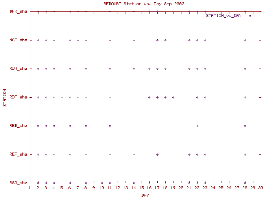
Station Use Plot for the Redoubt subnetwork for September 2002
