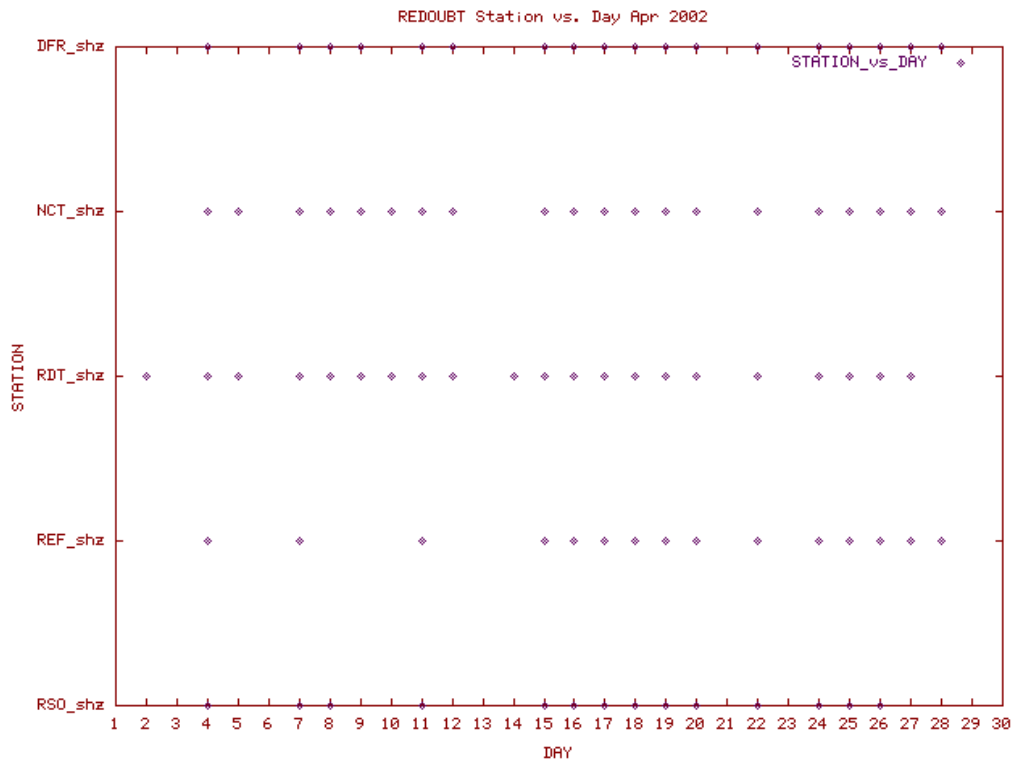
Station Use Plot for the Redoubt subnetwork for April 2002
