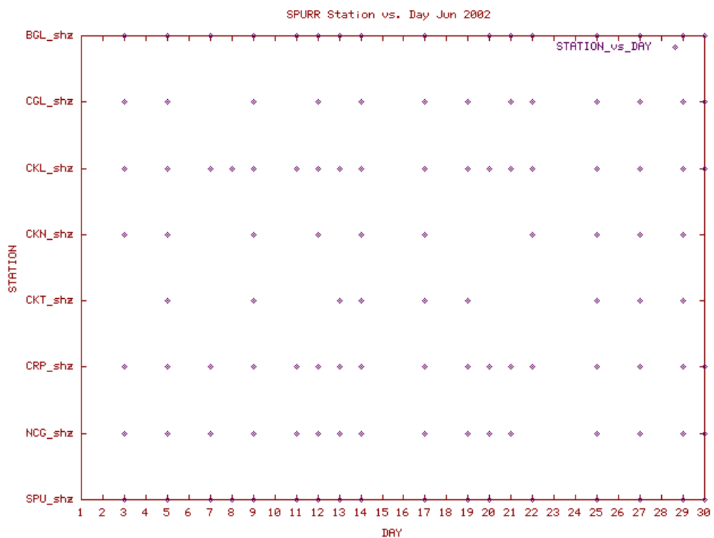
Station Use Plot for the Spurr subnetwork for June 2002
