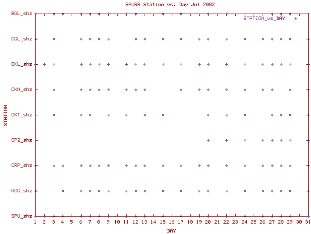
Station Use Plot for the Spurr subnetwork for July 2002
