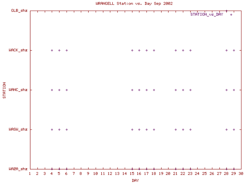
Station Use Plot for the Wrangell subnetwork for September 2002
