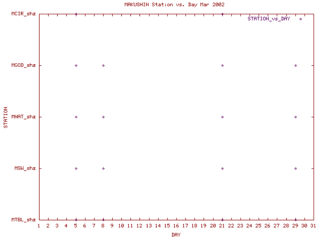
Station Use Plot for the Makushin subnetwork for March 2002
