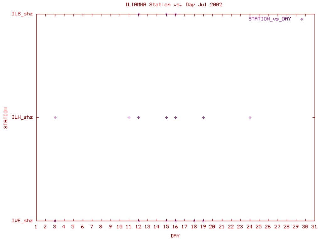
Station Use Plot for the Iliamna subnetwork for July 2002
