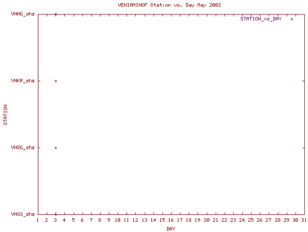
Station Use Plot for the Veniaminof subnetwork for May 2002
