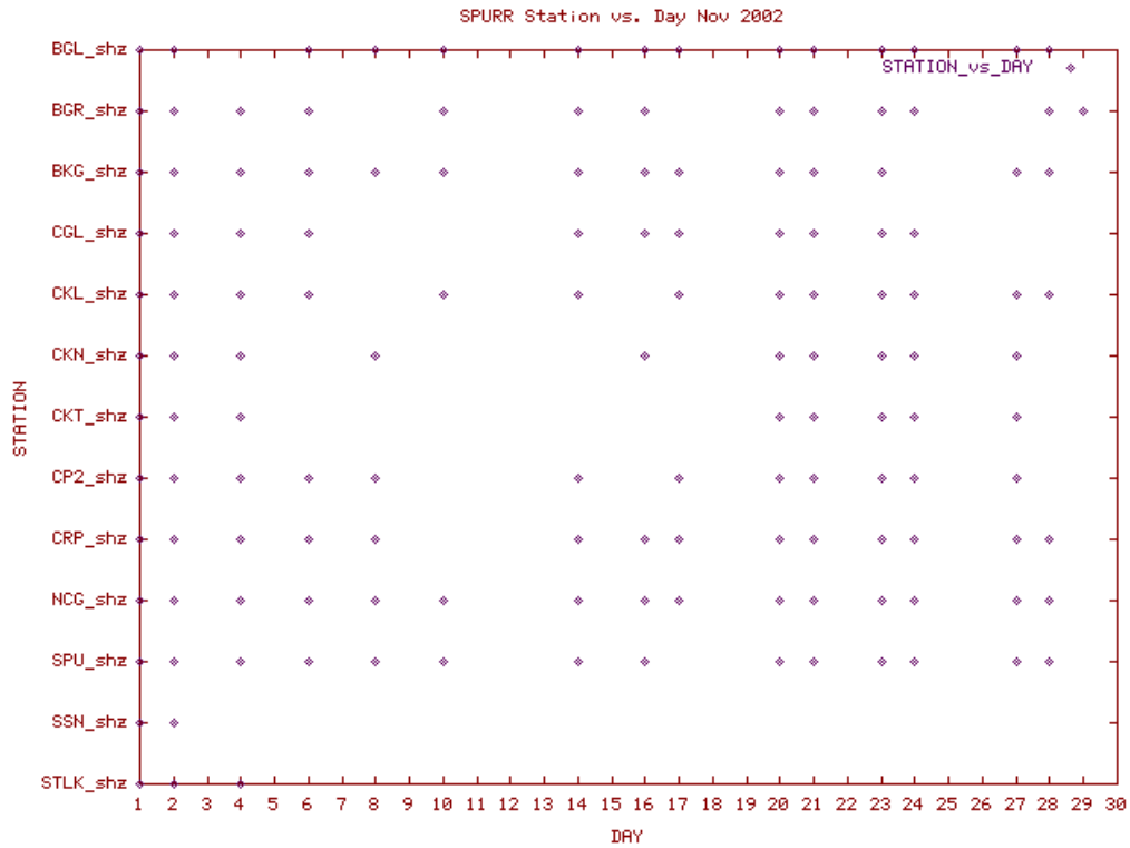
Station Use Plot for the Spurr subnetwork for November 2002
