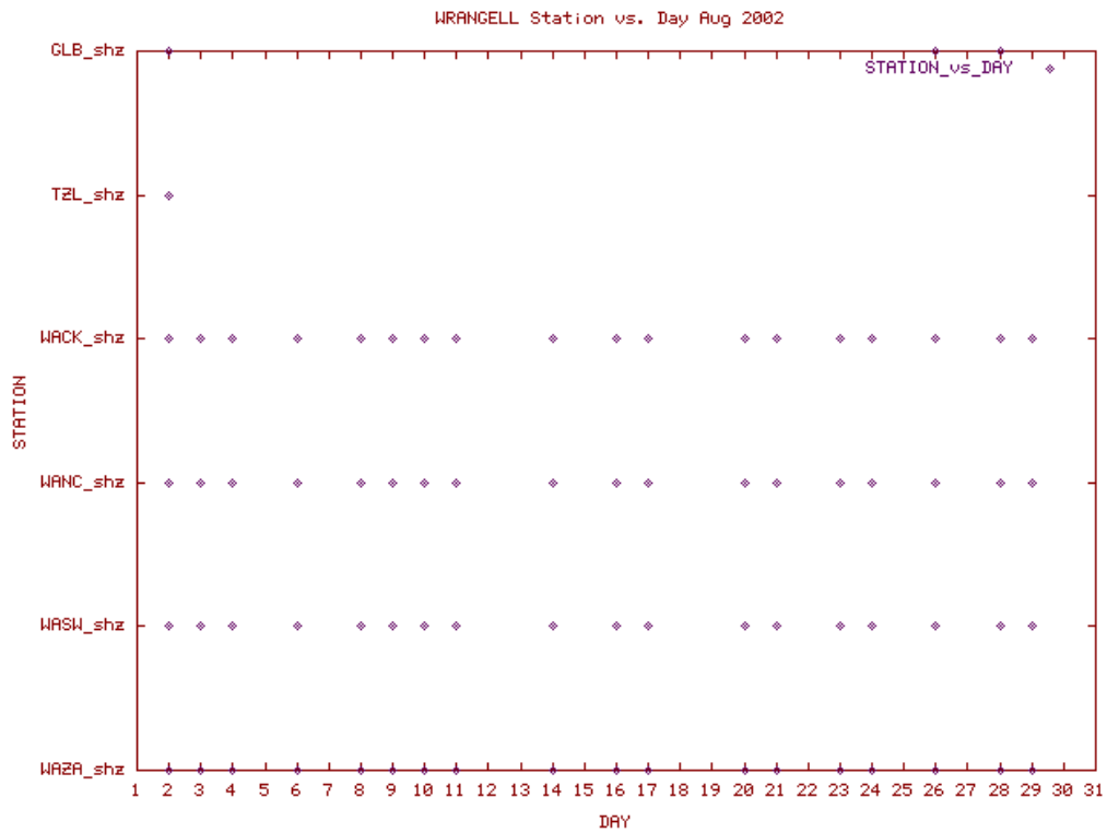
Station Use Plot for the Wrangell subnetwork for August 2002
