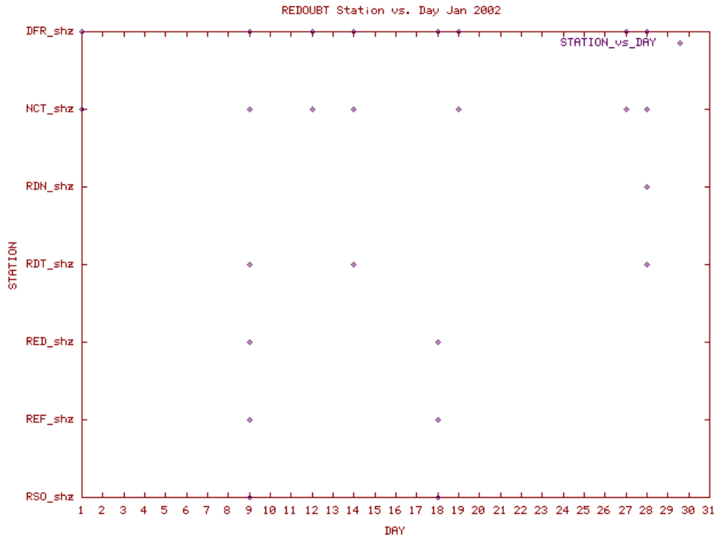
Station Use Plot for the Redoubt subnetwork for January 2002
