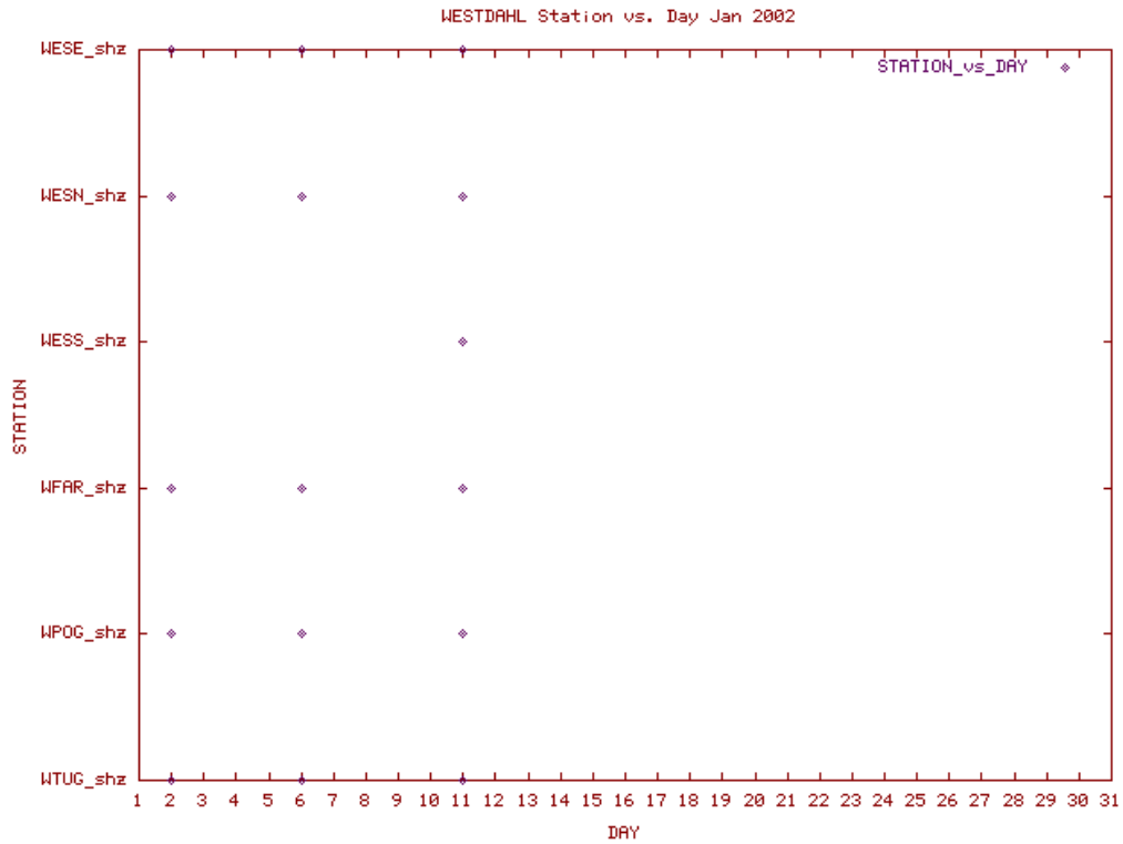
Station Use Plot for the Westdahl subnetwork for January 2002
