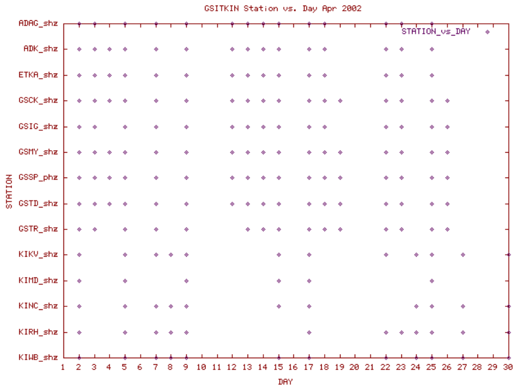
Station Use Plot for the Great Sitkin subnetwork for April 2002
