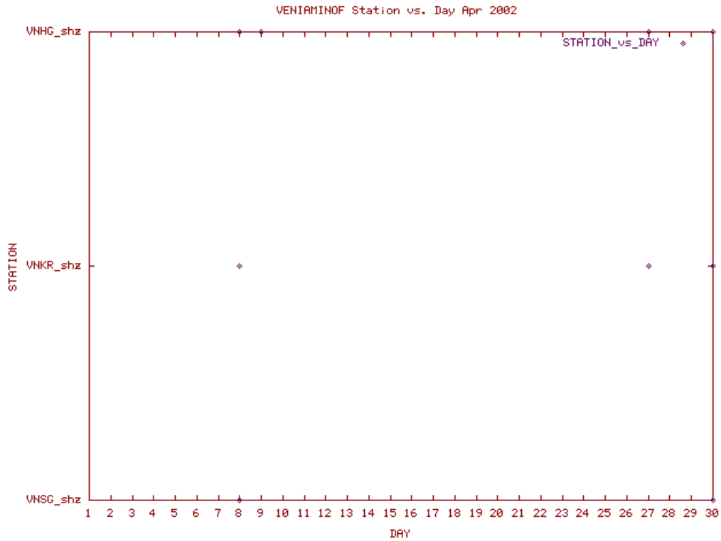
Station Use Plot for the Veniaminof subnetwork for April 2002
