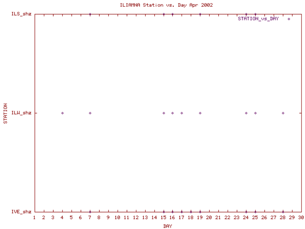
Station Use Plot for the Iliamna subnetwork for April 2002
