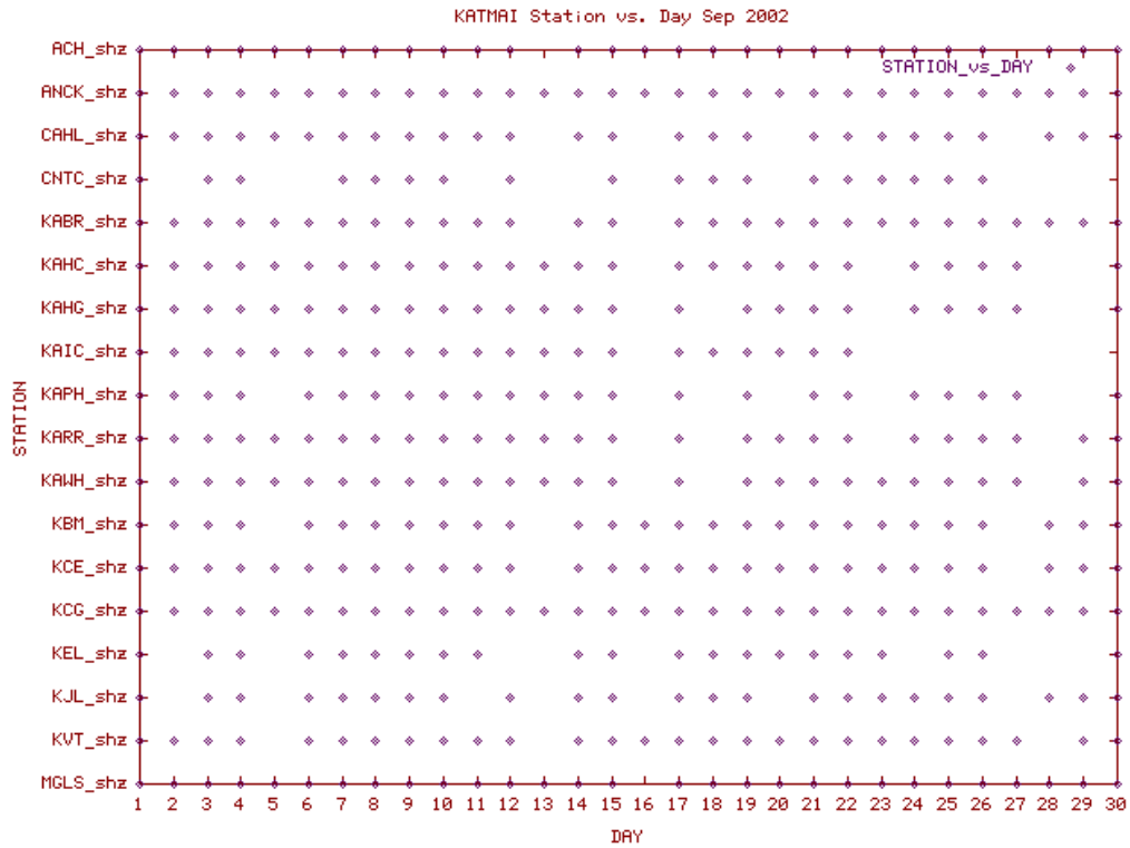
Station Use Plot for the Katmai volcanic group subnetwork for September 2002
