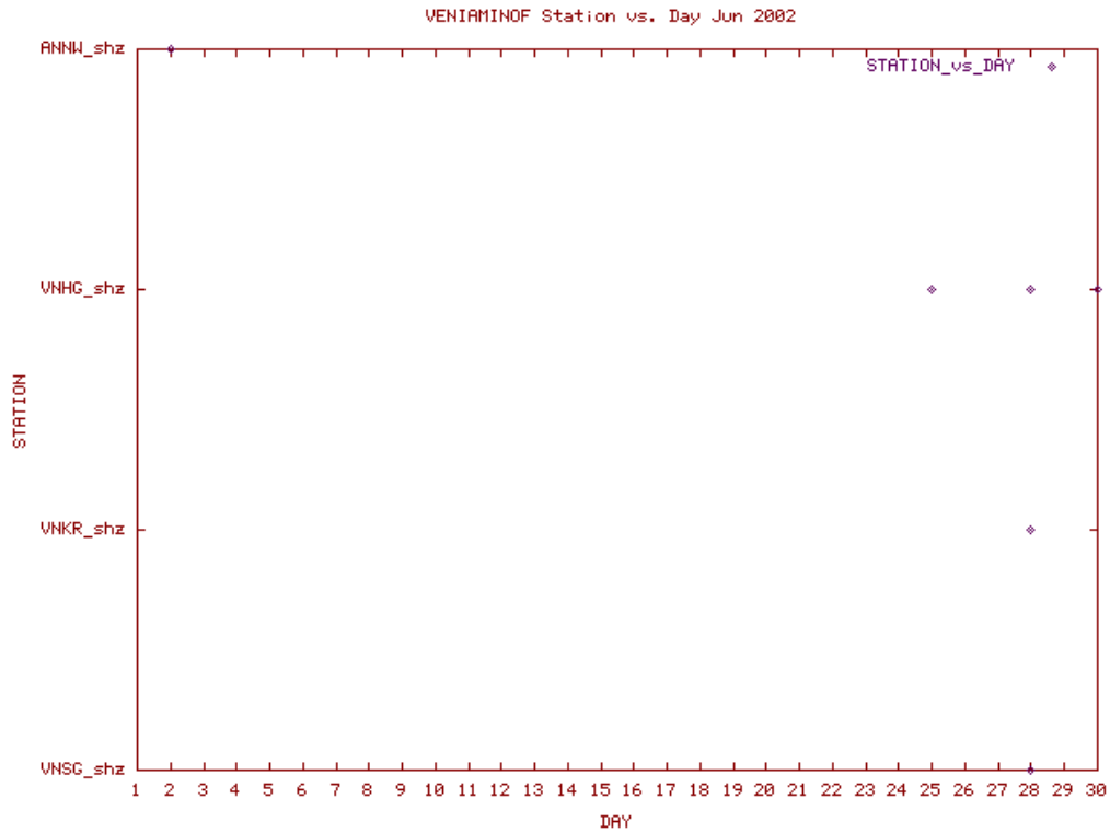
Station Use Plot for the Veniaminof subnetwork for June 2002
