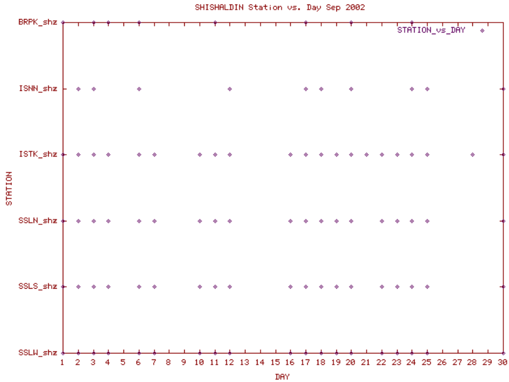
Station Use Plot for the Shishaldin subnetwork for September 2002
