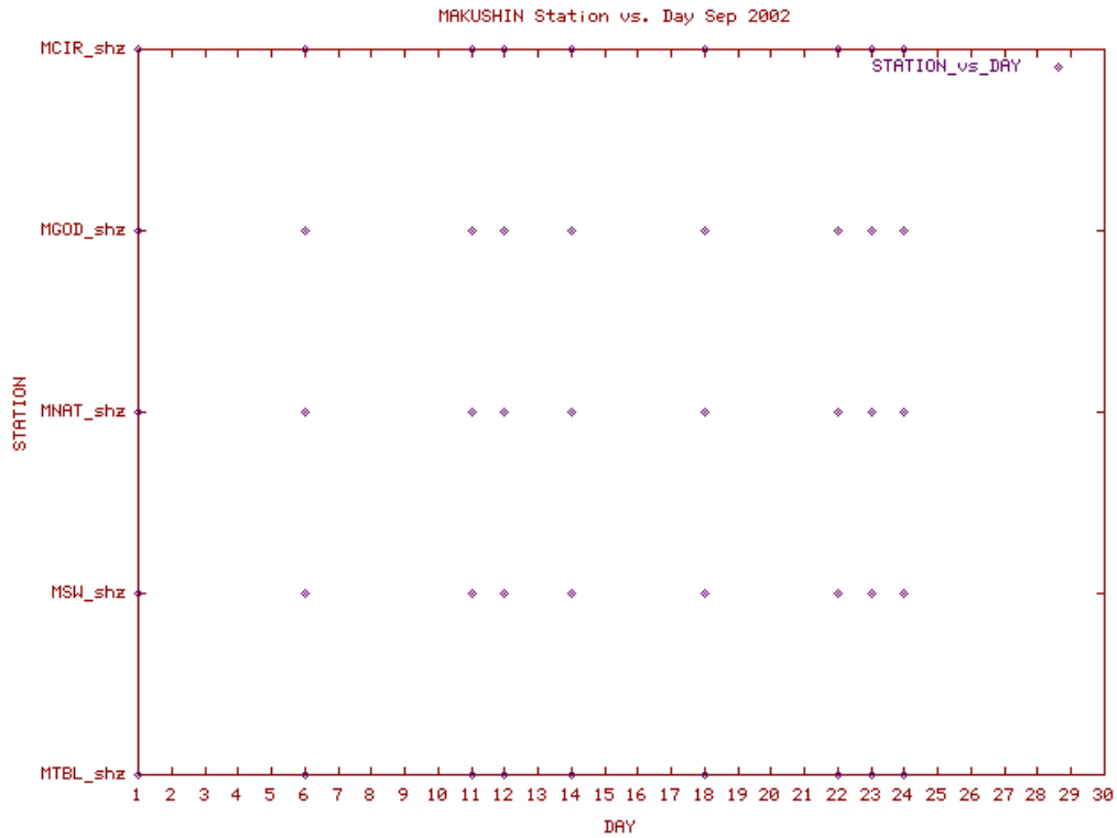
Station Use Plot for the Makushin subnetwork for September 2002
