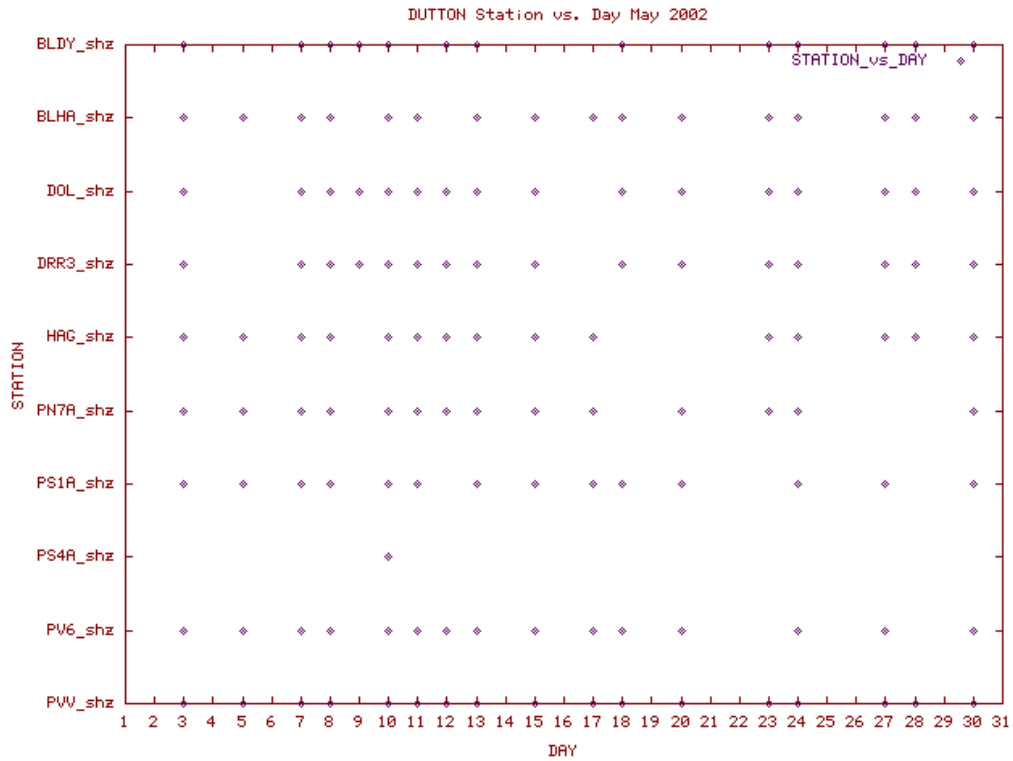
Station Use Plot for the Dutton and Pavlof subnetworks for May 2002
