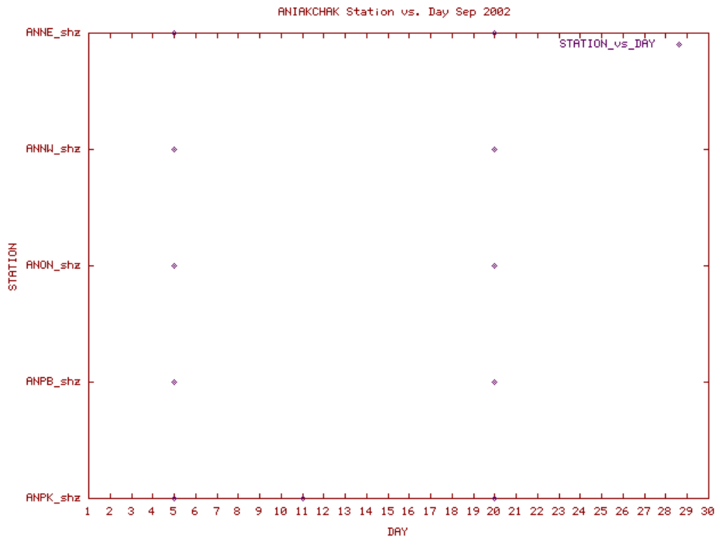
Station Use Plot for the Aniakchak subnetwork for September 2002
