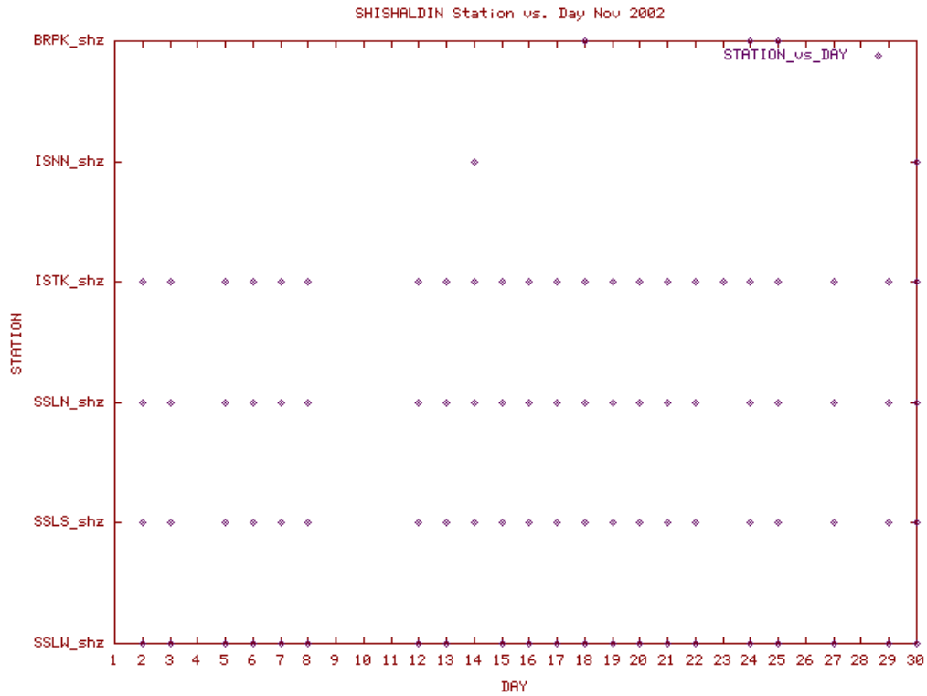
Station Use Plot for the Shishaldin subnetwork for November 2002
