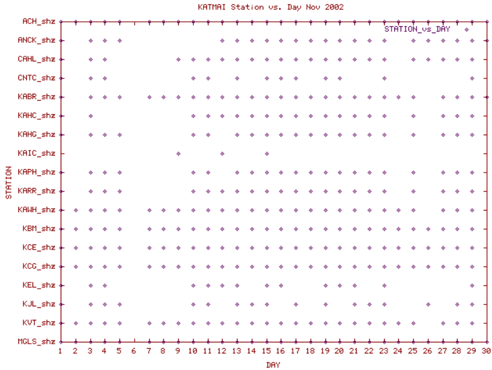
Station Use Plot for the Katmai volcanic group subnetwork for November 2002
