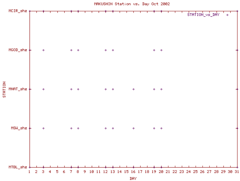
Station Use Plot for the Makushin subnetwork for October 2002
