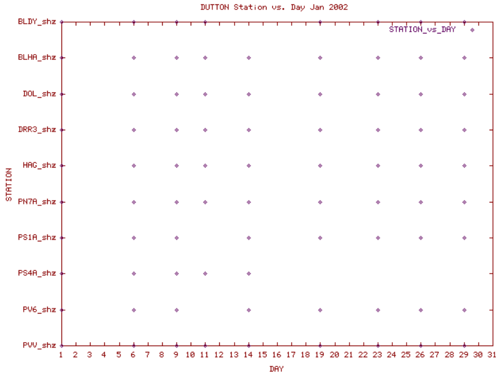
Station Use Plot for the Dutton and Pavlof subnetworks for January 2002
