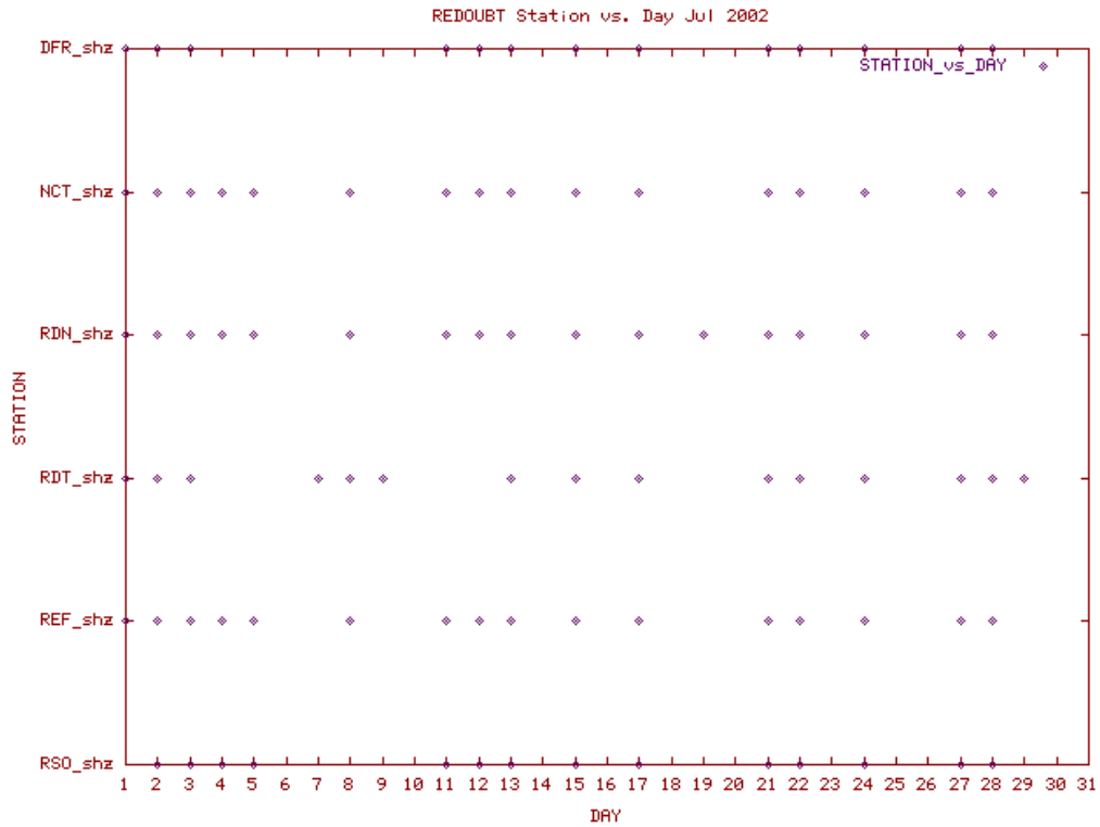
Station Use Plot for the Redoubt subnetwork for July 2002
