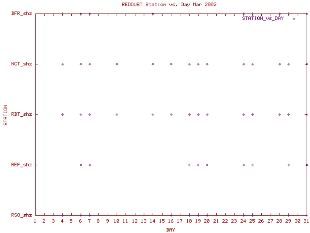
Station Use Plot for the Redoubt subnetwork for March 2002
