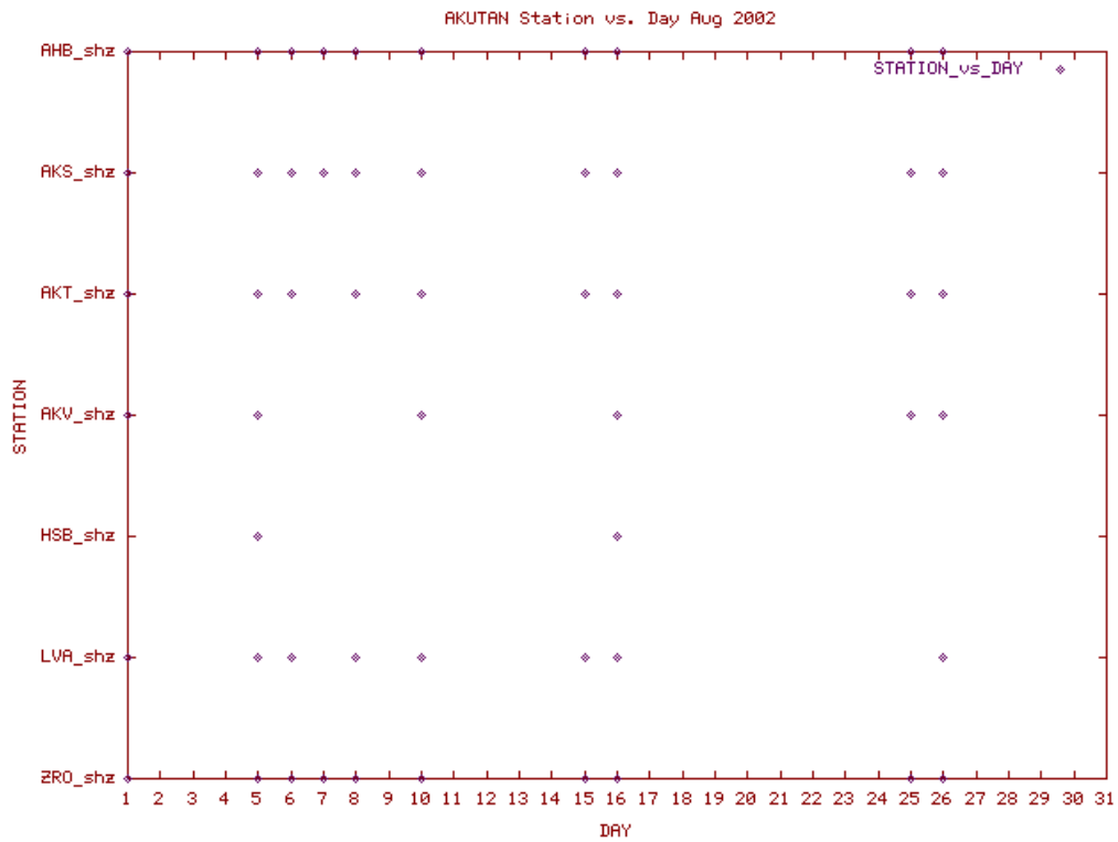
Station Use Plot for the Akutan subnetwork for August 2002
