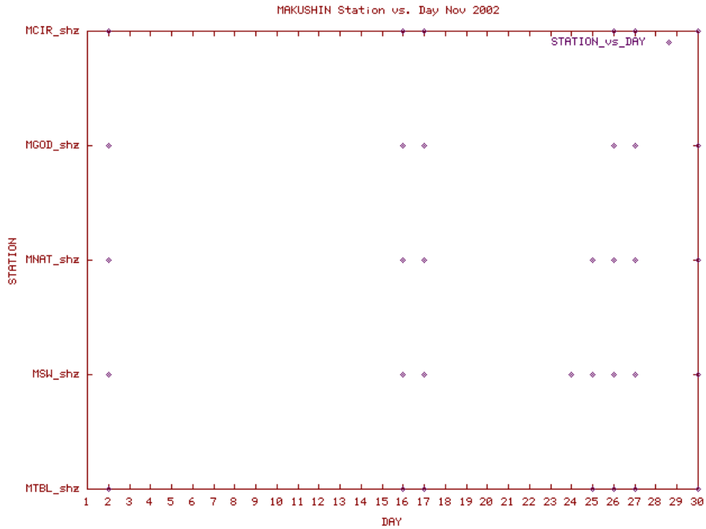
Station Use Plot for the Makushin subnetwork for November 2002
