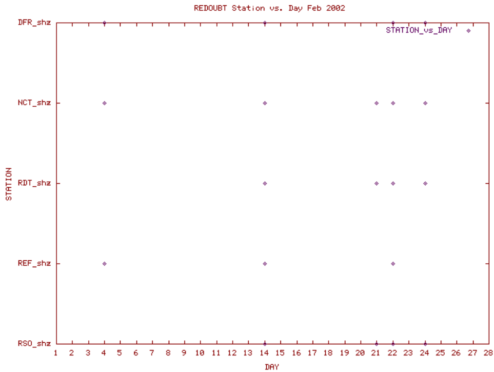
Station Use Plot for the Redoubt subnetwork for February 2002
