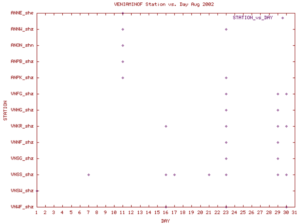
Station Use Plot for the Veniaminof subnetwork for August 2002
