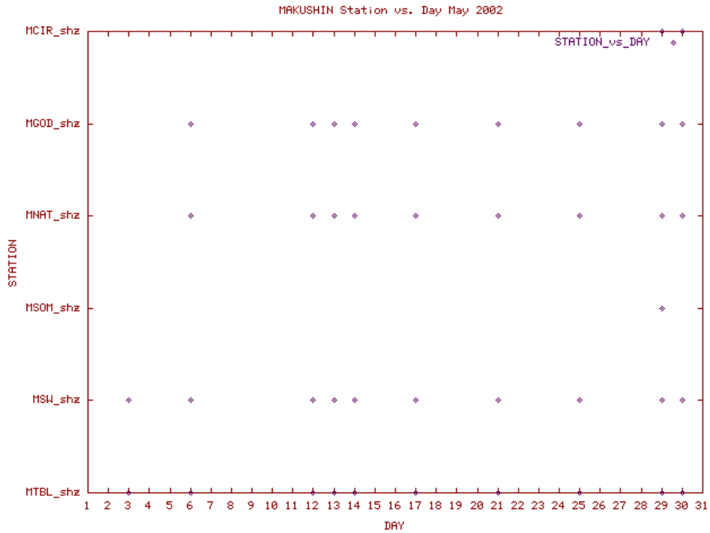
Station Use Plot for the Makushin subnetwork for May 2002
