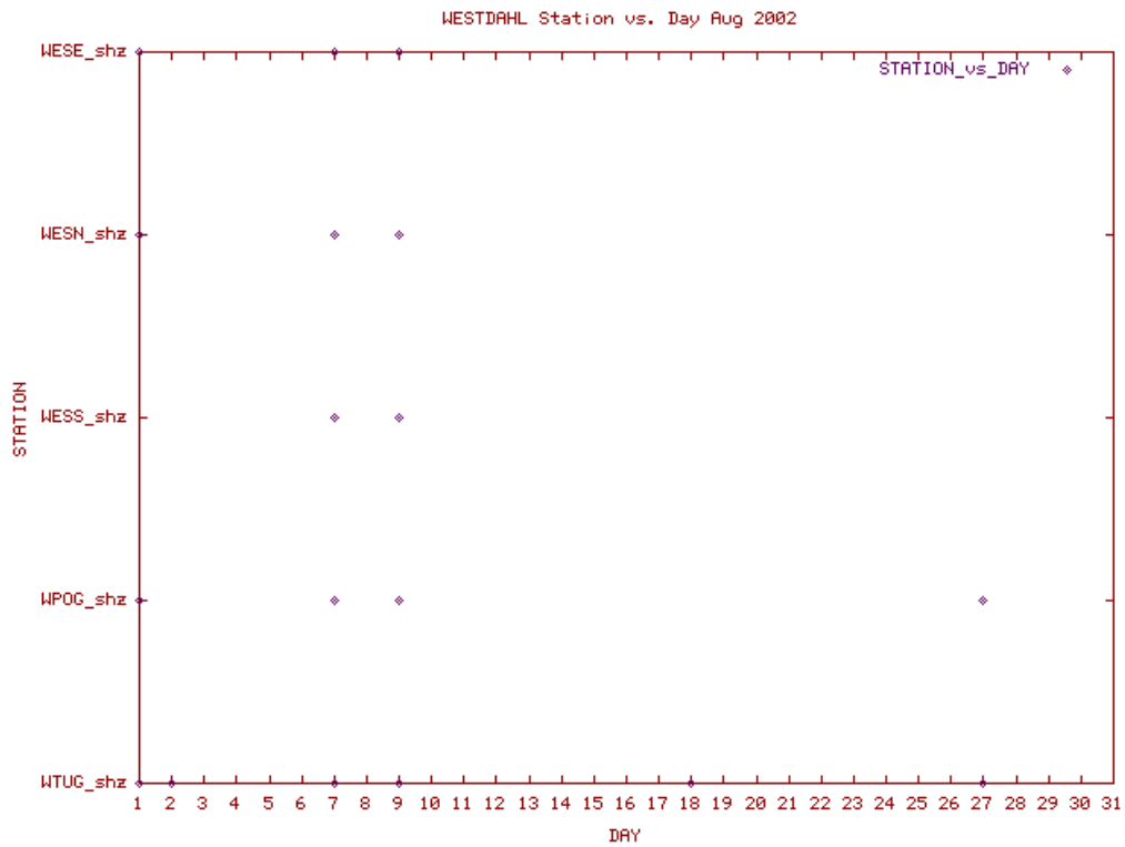
Station Use Plot for the Westdahl subnetwork for August 2002
