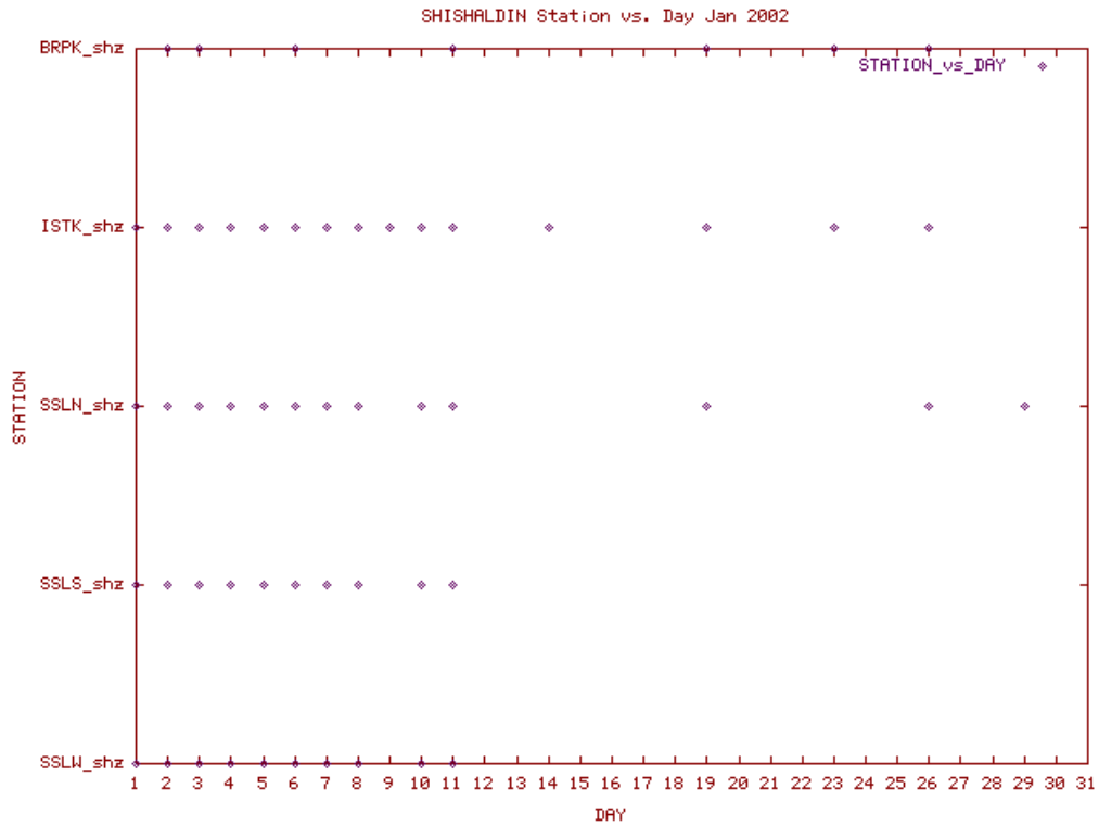
Station Use Plot for the Shishaldin subnetwork for January 2002
