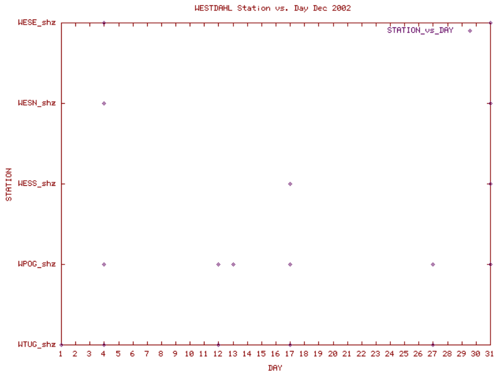
Station Use Plot for the Westdahl subnetwork for December 2002
