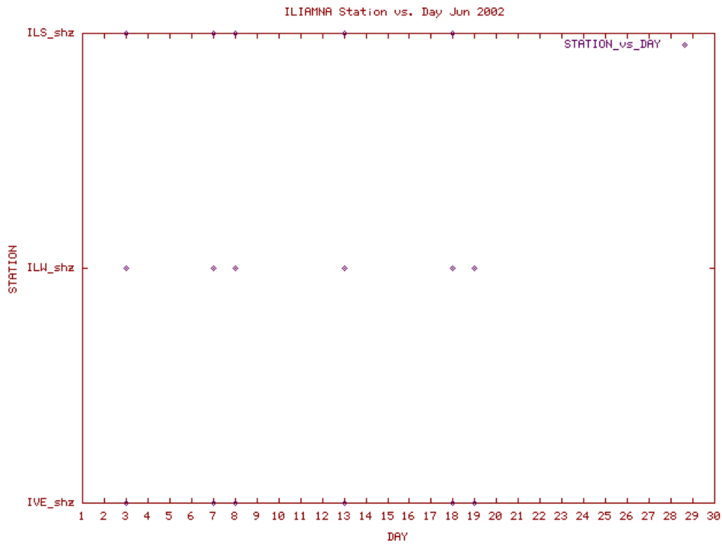
Station Use Plot for the Iliamna subnetwork for June 2002
