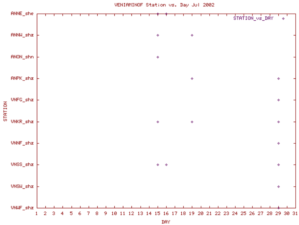
Station Use Plot for the Veniaminof subnetwork for July 2002
