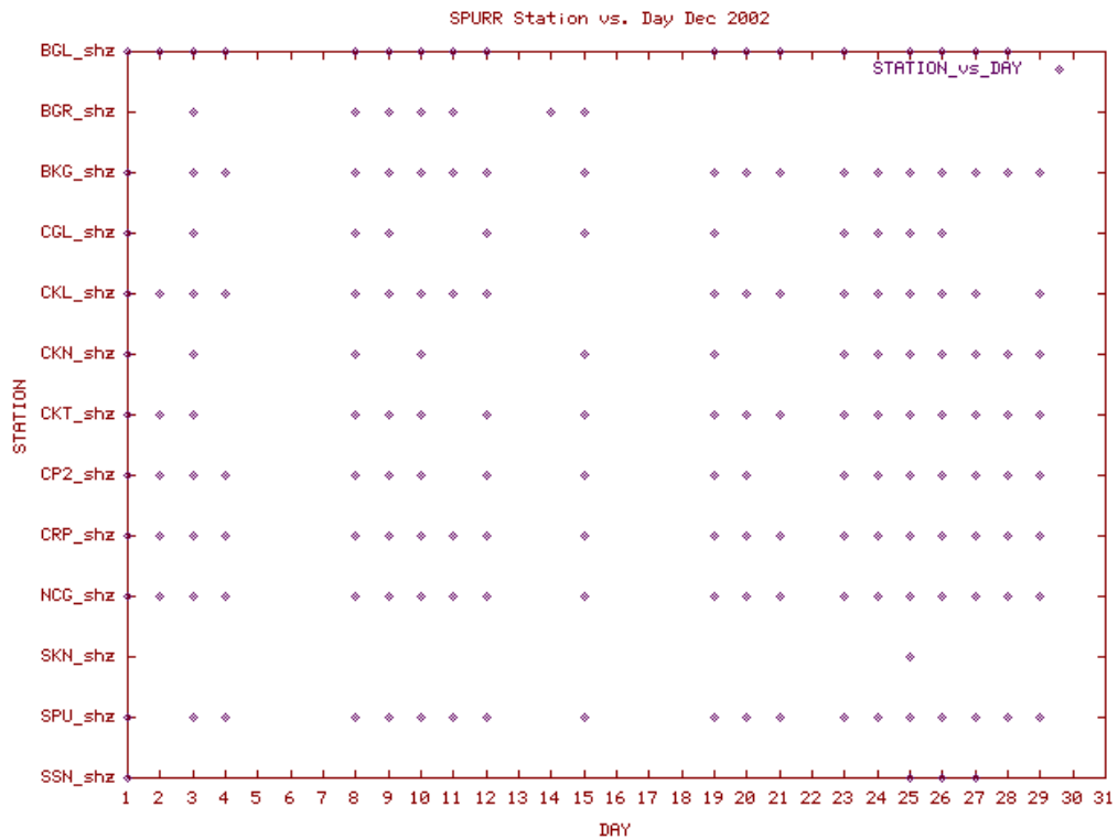
Station Use Plot for the Spurr subnetwork for December 2002
