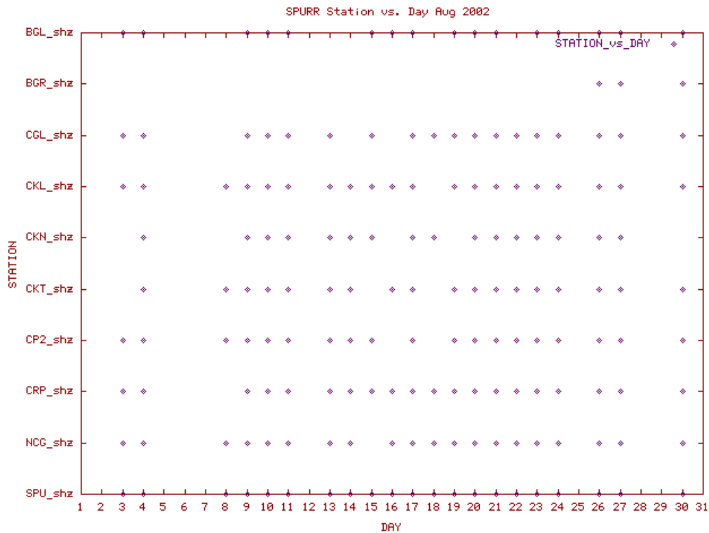
Station Use Plot for the Spurr subnetwork for August 2002
