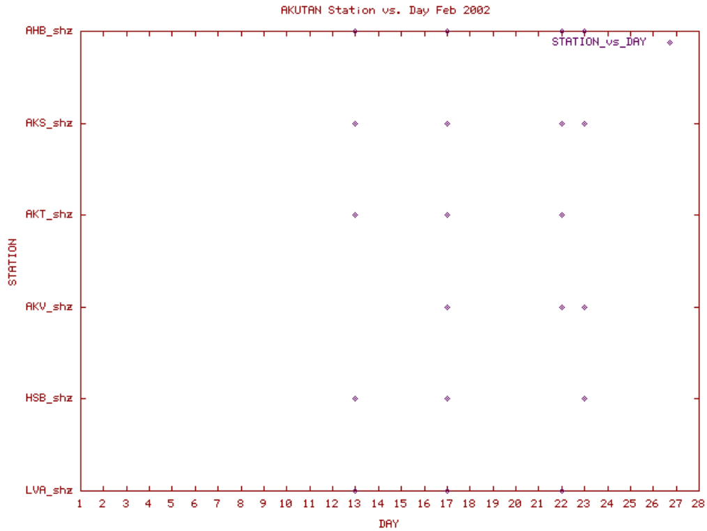
Station Use Plot for the Akutan subnetwork for February 2002
