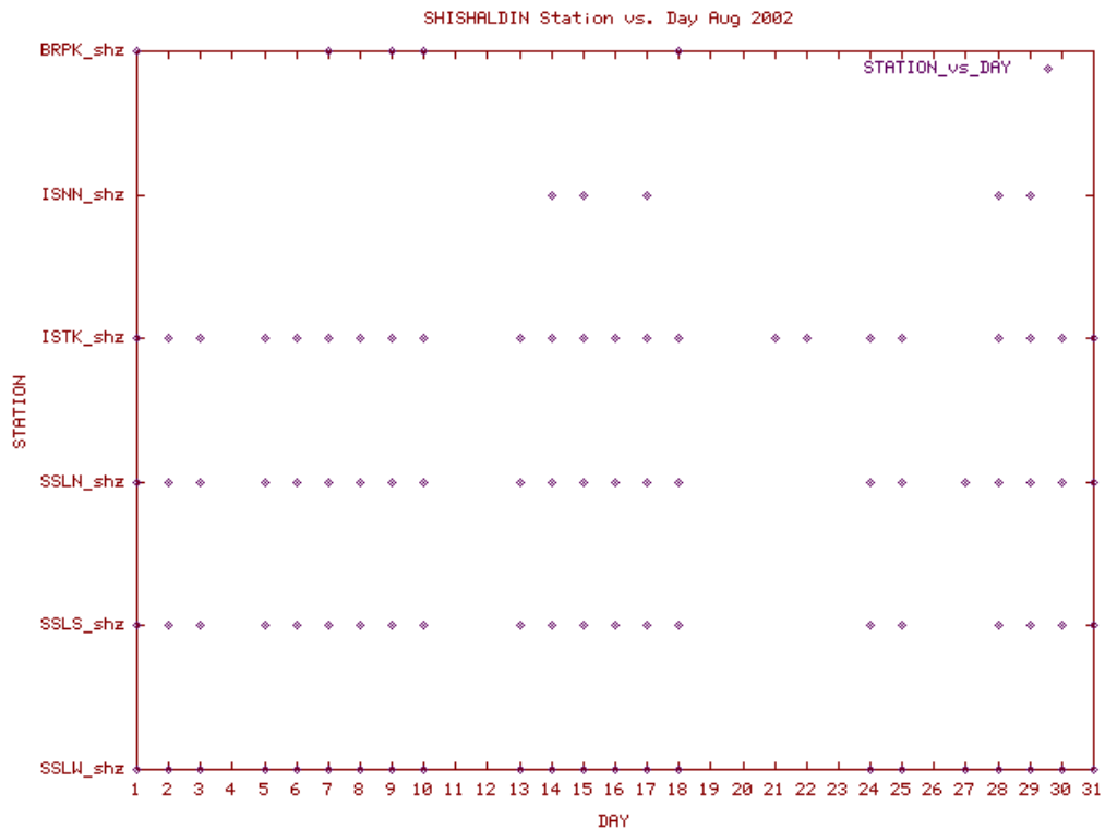
Station Use Plot for the Shishaldin subnetwork for August 2002
