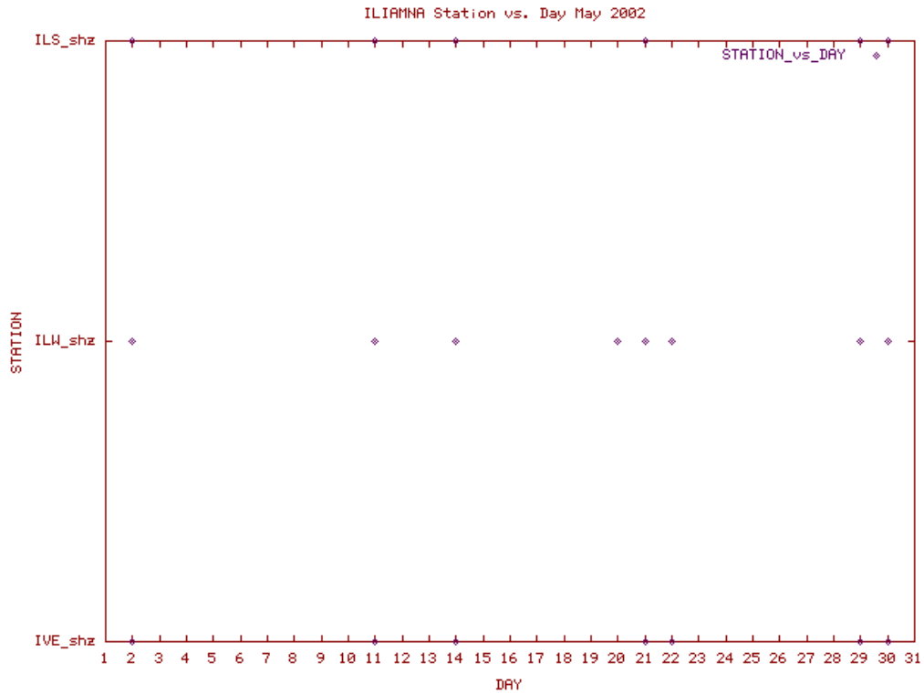
Station Use Plot for the Iliamna subnetwork for May 2002
