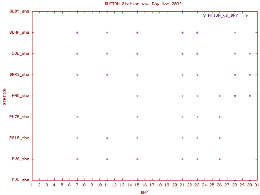
Station Use Plot for the Dutton and Pavlof subnetworks for March 2002
