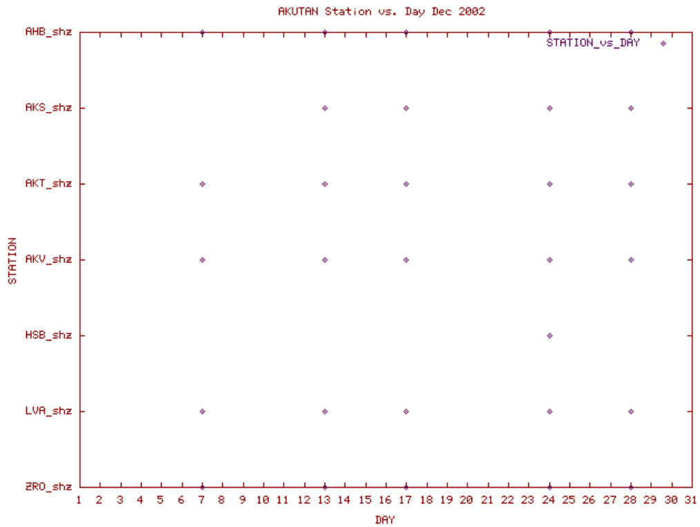
Station Use Plot for the Akutan subnetwork for December 2002
