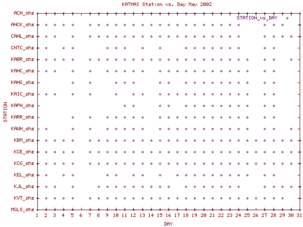
Station Use Plot for the Katmai volcanic group subnetwork for May 2002
