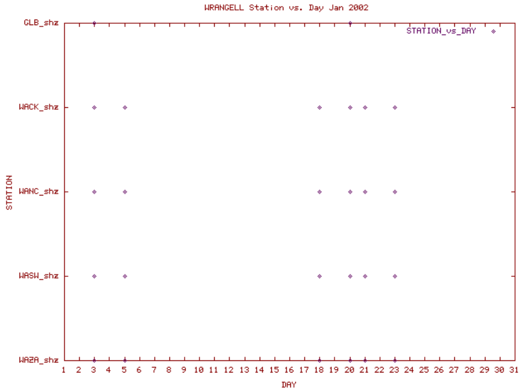
Station Use Plot for the Wrangell subnetwork for January 2002
