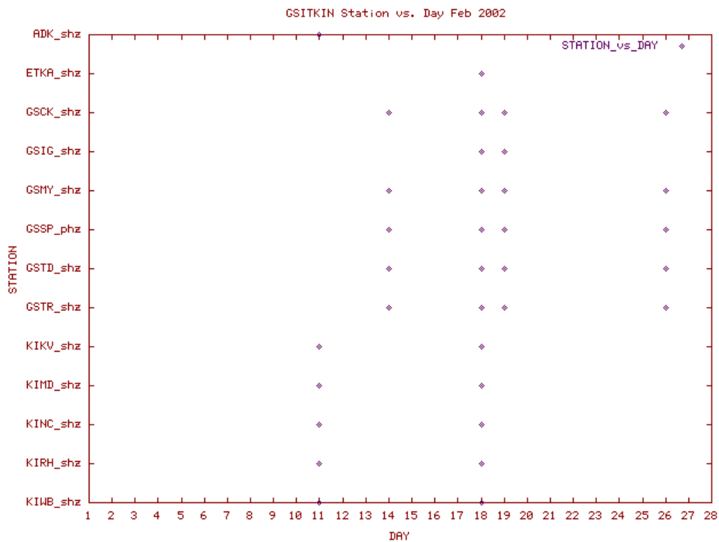
Station Use Plot for the Shishaldin subnetwork for February 2002
