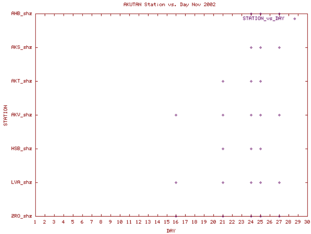
Station Use Plot for the Akutan subnetwork for November 2002
