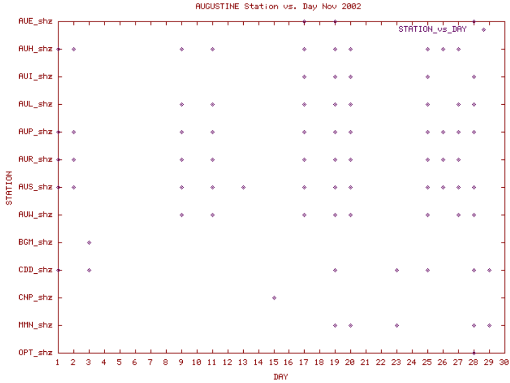
Station Use Plot for the Augustine subnetwork for November 2002
