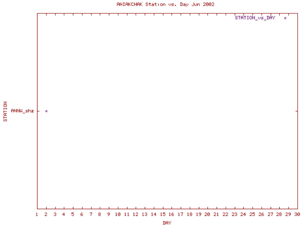
Station Use Plot for the Aniakchak subnetwork for June 2002
