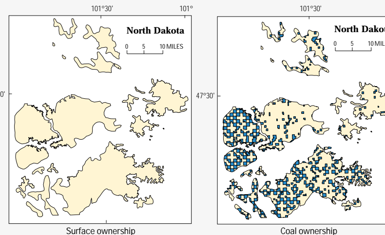
Figure 4. Index map showing the priority coal assessment unit study areas within Tertiary coal basins and maps showing Federal coal and surface ownership.
