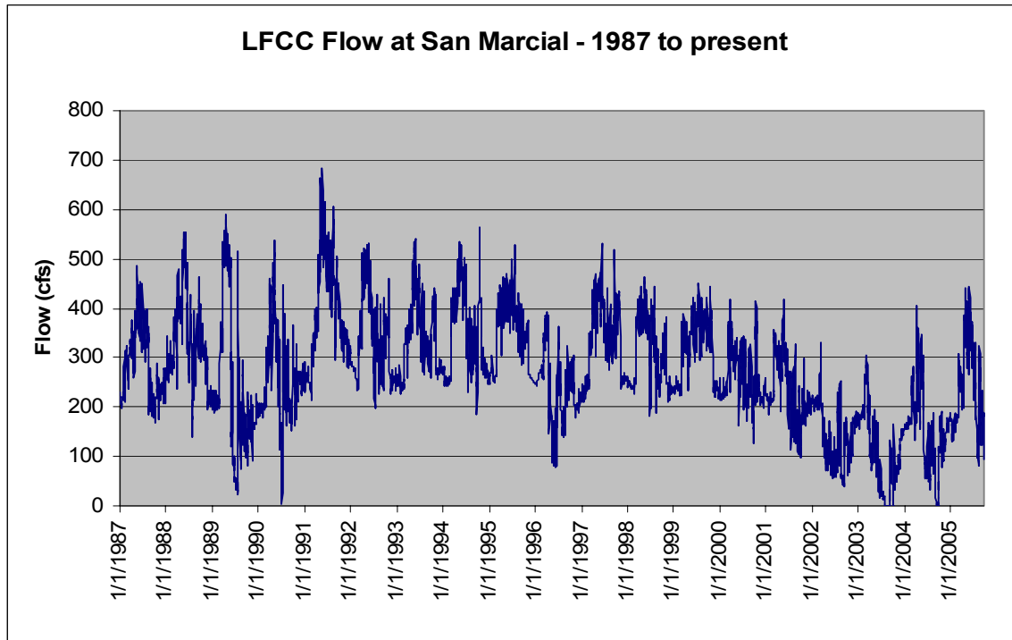
Figure 7. Average daily flow within the Low Flow Conveyance Channel, 1987 to present.
