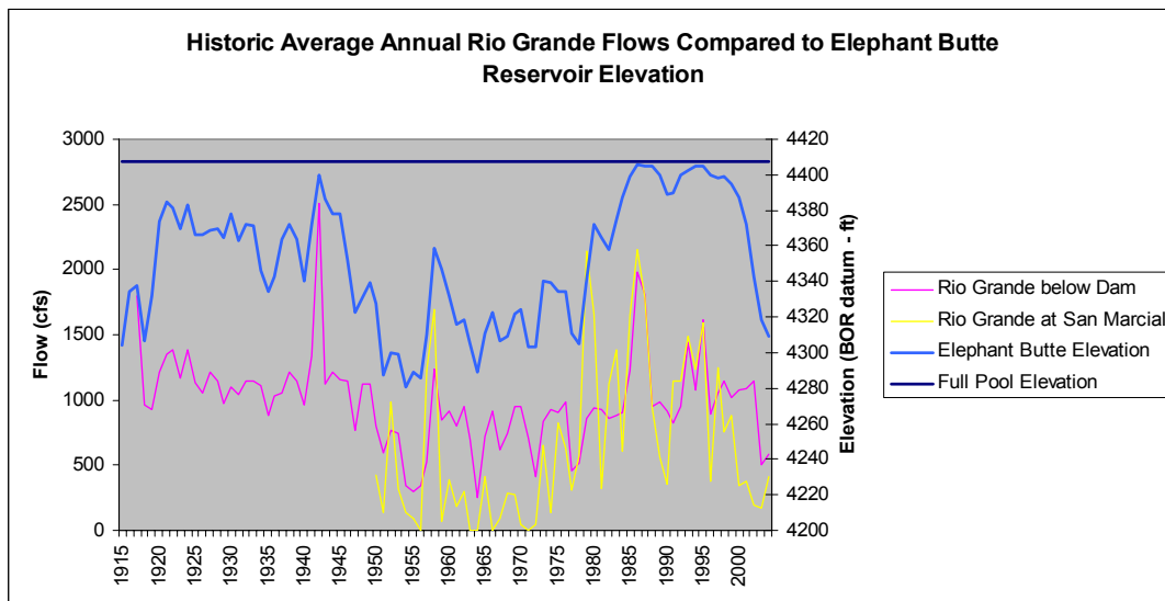
Figure 1. Average annual flow in the Rio Grande compared to Elephant Butte Reservoir elevations from 1915 to 2004. The San Marcial station was not installed until 1950.
