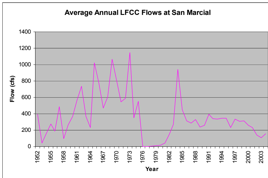
Figure 2. Average annual flow in the Low Flow Conveyance Channel at San Marcial from construction to present.
