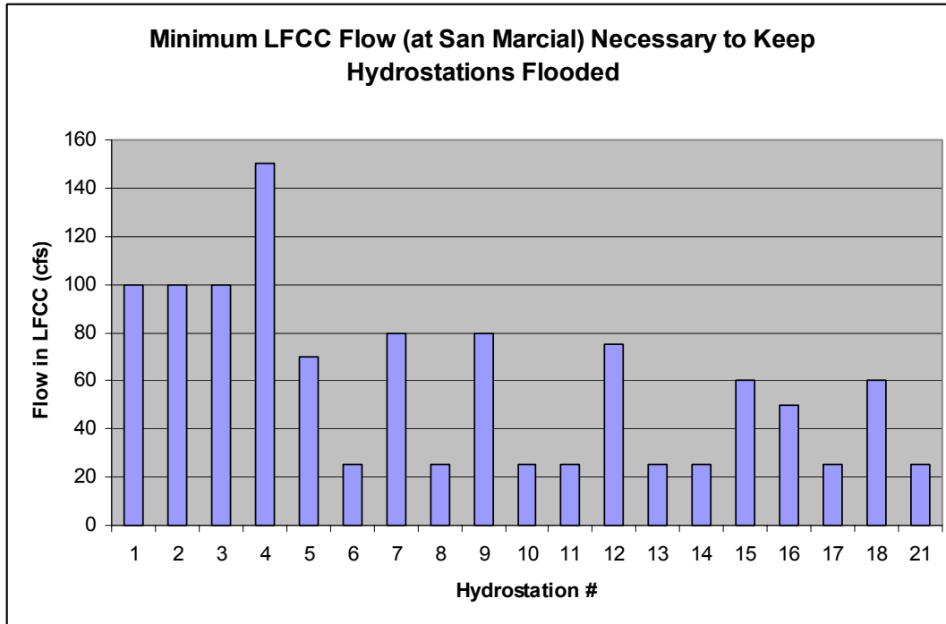
Figure 10. Minimum LFCC flows needed to keep hydrostations flooded during the 2004 and 2005 SWFL breeding seasons. Many hydrostations never dried out during the 2004 and 2005 seasons and the minimum flow during those years was 45 cfs, therefore stations were assigned a minimum flow of 25 cfs.
