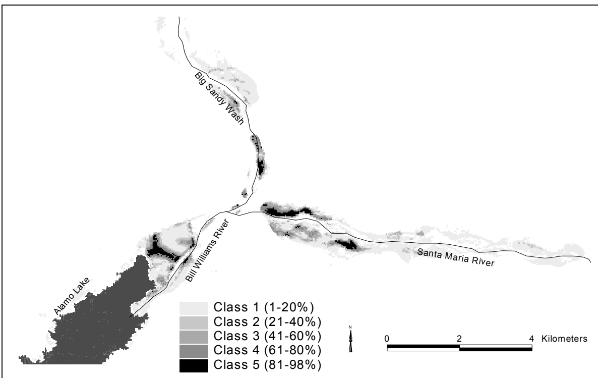
Figure 1.6. A southwestern willow flycatcher breeding-site suitability map of the Alamo Lake, Arizona test area that was produced from a GIS-based model developed 200 km to the southeast. The GIS-based model used logistic regression, digital elevation models, and TM imagery to map the probability of breeding-site occurrence. Probabilities ranged from 1 to 98%, which we reclassified into 1 of 5 probability classes.
