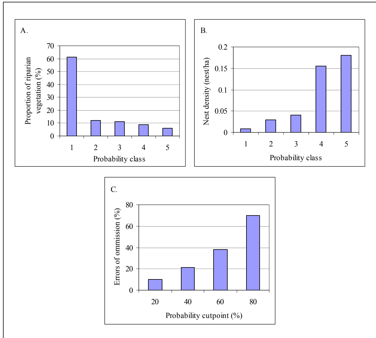
Figure 1.4. The proportion of predicted breeding habitat (A) and nest density (B) within 5 probability classes, produced from a GIS-based model within our project area (Arizona, USA) in 1999, and omission error at different probability cutpoints (C). Nest density was calculated from control sites (nests) not used in model development. The 5 classes divide the probability of breeding activity, as determined from the model, into 20% increments, while errors of omission refer to the number of nests found outside the suitability envelope. Cells with probabilities less than or equal to the probability cutpoint were considered unsuitable, while cells with values greater than the probability cutpoint were considered suitable.
