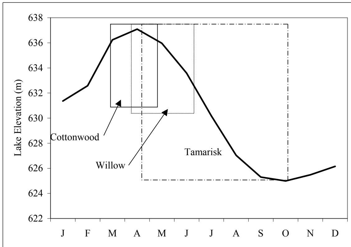
Figure 3.5. Seed-dispersal months (boxes) for 3 riparian tree species overlaid on Roosevelt Lake water elevations in 2001 (solid bold line). Note the greater chance for tamarisk establishment as water levels decline late in the growing season. Seed-dispersal data from Shafroth and others (1998) study on the Bill Williams River, west-central Arizona.
