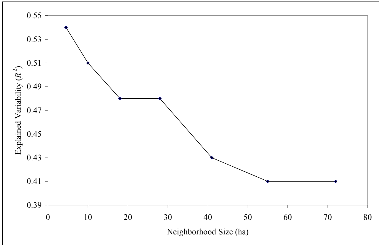
Figure 1.2. Amount of explained variability ( R^2 ) in southwestern willow flycatcher breeding-site occurrence, as determined with multiple logistic regression, within 7 different-sized neighborhoods (4.5-72 ha) around breeding and nonuse sites. In this analysis, NDVI (relative density of green vegetation at site) and FLOODPL12 (amount of floodplain or flat area within a 41-ha neighborhood) were constants, while a different-sized neighborhood was examined for the 2 vegetation variables (NDVISTD [standard deviation of NDVI] and NDVIBEST [amount of densest vegetation]) in each of the 7 model runs.
