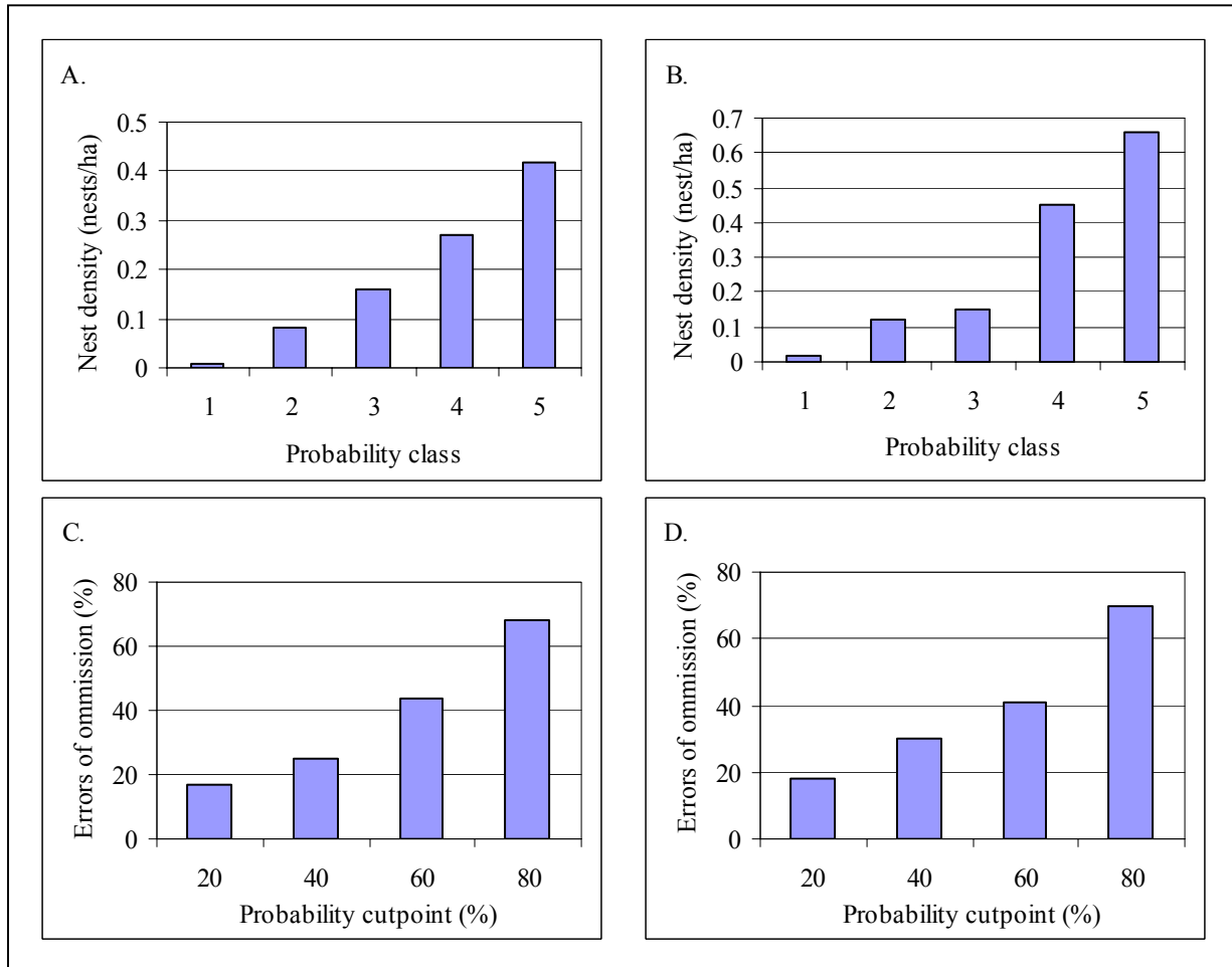
Figure. 1.5. We assessed the temporal accuracy of the 1999 model by overlaying 398 southwestern willow flycatcher breeding sites identified between 1995 and 1998, and 601 between 2000 and 2001, within the project area. Model fit was examined with nest density 1995-1998 (A) and 2000-2001 (B) within 5 probability classes. Model accuracy was determined by omission errors between 1995-1998 (C) and 2000-2001 (D) at 20% probability cutpoints. Cells with probabilities less than or equal to the probability cutpoint were considered unsuitable, while cells with values greater than the probability cutpoint were considered suitable.
