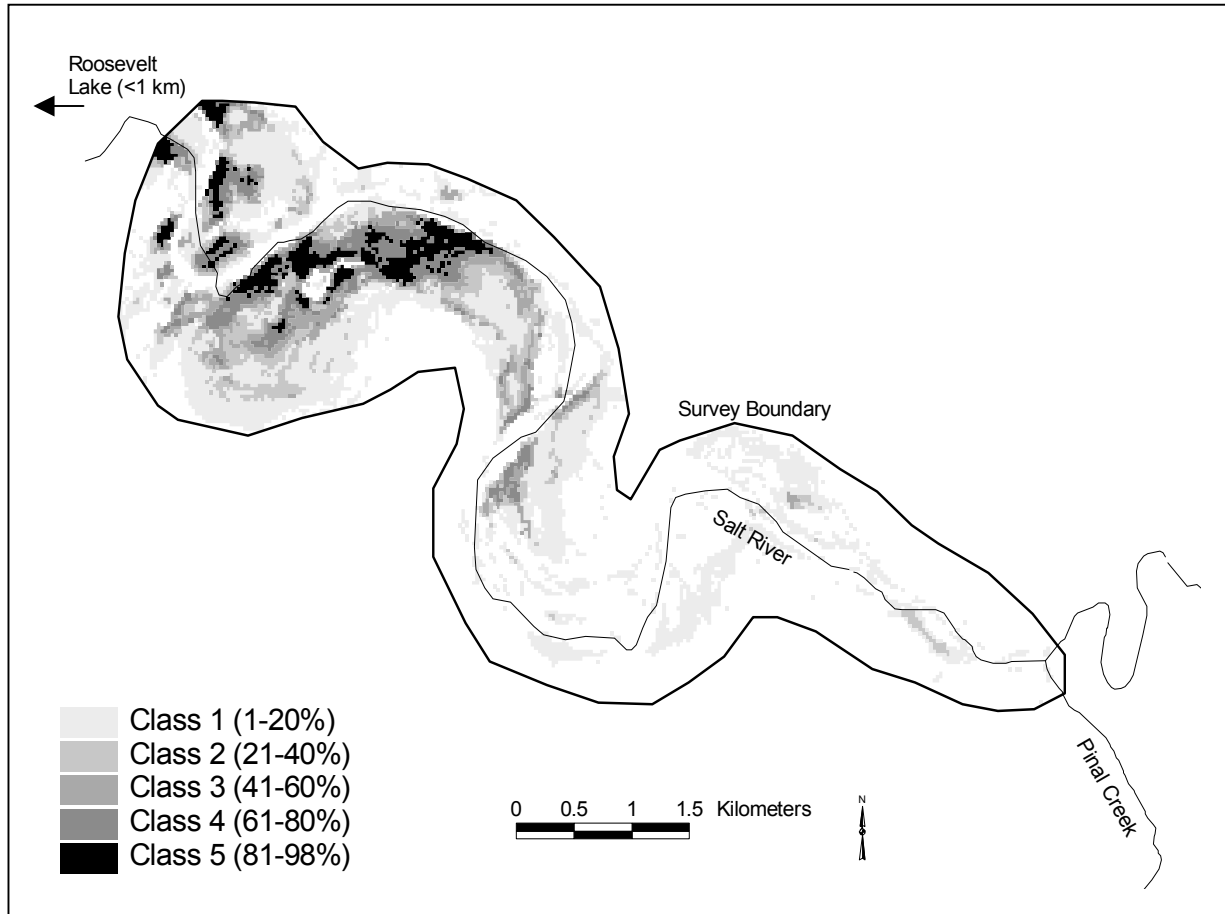
Figure 1.3. A southwestern willow flycatcher breeding-site suitability map of Salt River, Arizona, survey area in 1999 produced from a GIS-based model, logistic regression, digital elevation models, and Thematic Mapper imagery. Probability of breeding-site occurrence ranged from 1 to 98%, which we reclassified into 1 of 5 probability classes.
