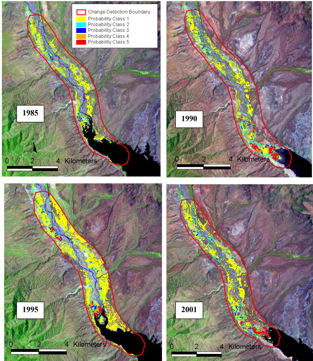
Tonto Creek inflow: predicted suitable SWFL breeding habitat in 1985, 1990, 1995, and 2001. Probability divided into 5 suitability classes: 1 (lowest potential) to 5 (highest potential).
