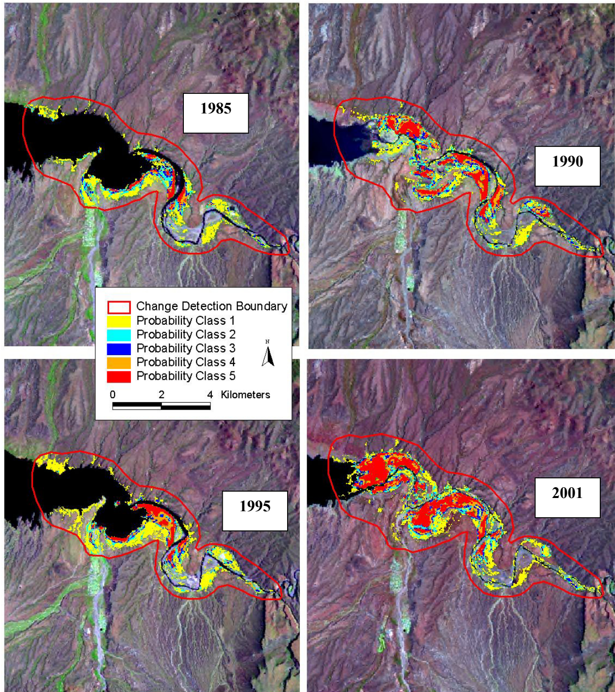
Salt River inflow: predicted suitable SWFL breeding habitat in 1985, 1990, 1995, and 2001. Probability divided into 5 suitability classes: 1 (lowest potential) to 5 (highest potential).
