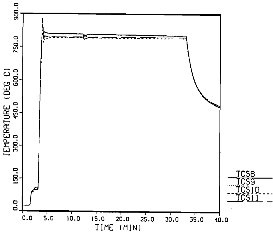
Figure 6.1-2 Radiant Heat Shroud Temperature Profile, Center Axial Plane
