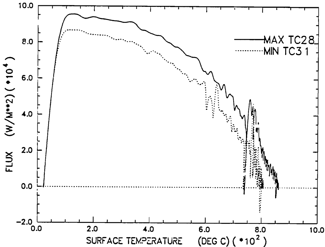
Figure 6.4-11 Maximum and Minimum Surface Heat Flux as a Function of Surface Temperature Obtained from the 870°C, 100-Minute Radiant Heat Test
