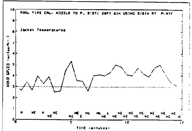
Fig. B-3: Pool fire calibration test TF-31-01-86-CAL-E, wind speed and direction.
