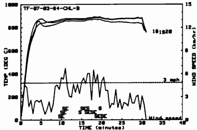
Figure 5: Jacket Temperatures and Wind Speed for the First Torch Fire Test of Kaowool (A-1)
