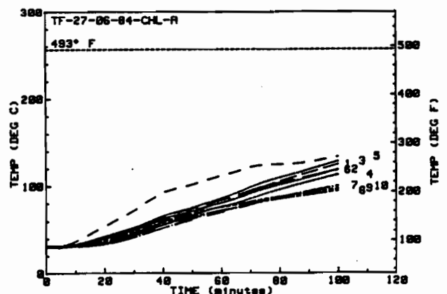
Figure 49: Back Plate and Rear Enclosure Air Temperatures for the Second Pool Test of Cerawool (C-5)
