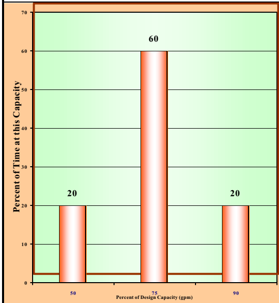
Sample Duty Cycle - HIGH PUMP LOADING
