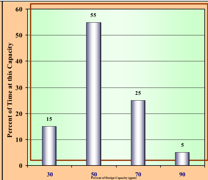
Sample Duty Cycle - LOW PUMP LOADING
