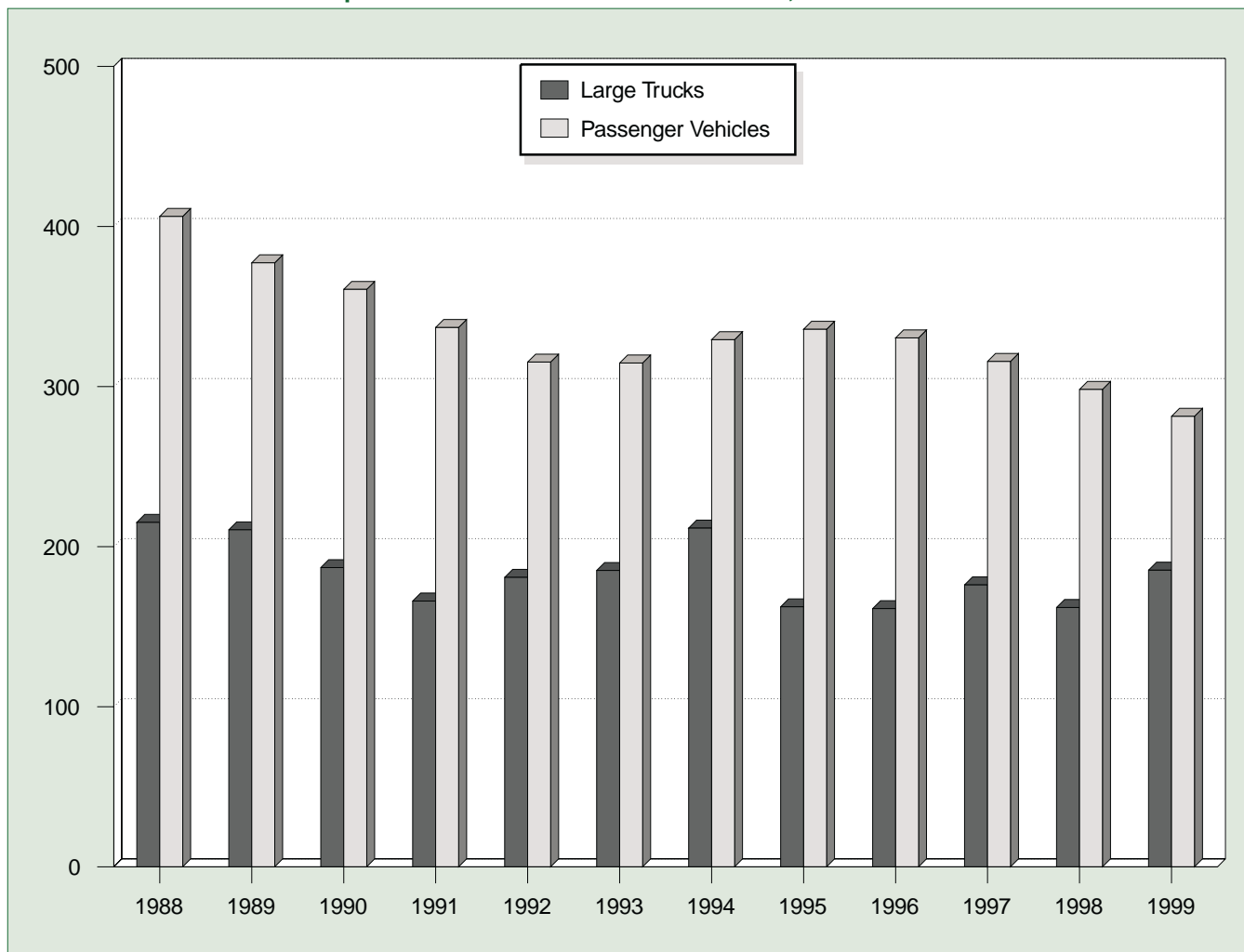
Figure 6. Large Trucks and Passenger Vehicles Involved in Property Damage Only Crashes per 100 Million Vehicle Miles Traveled, 1988-1999
