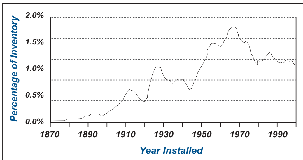
Figure 2–10: Age Distribution of Current Inventory of Pipe for 20 Cities
