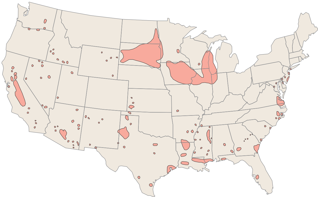
Figure 9. Areas of water-table decline or artesian water-level decline in excess of 40 feet in at least one aquifer since predevelopment (modified from U.S. Geological Survey, 1984).
