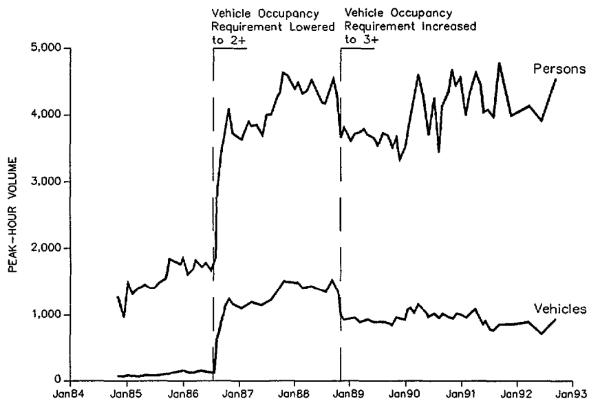
Figure 9. Katy Freeway HOV Lane, A.M. Peak-Hour Utilization
