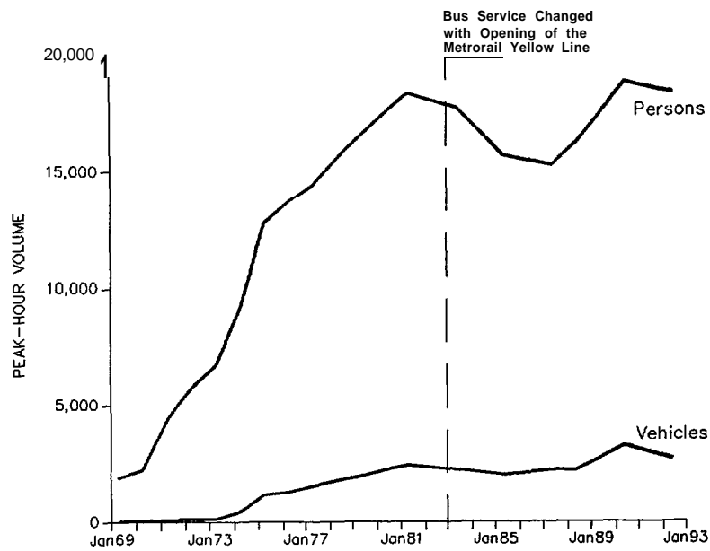
Figure 19. Shirley Highway HOV Lanes, A.M. Peak-Hour Utilization
