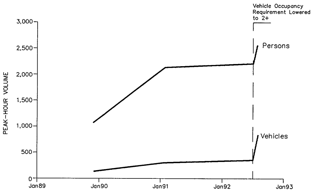
Figure 15. I-279 HOV Lanes, A.M. Peak-Hour Utilization
