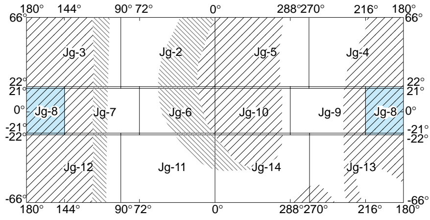
Approximate resolution of available Voyager images expressed as kilometers per picture element (pxl)
