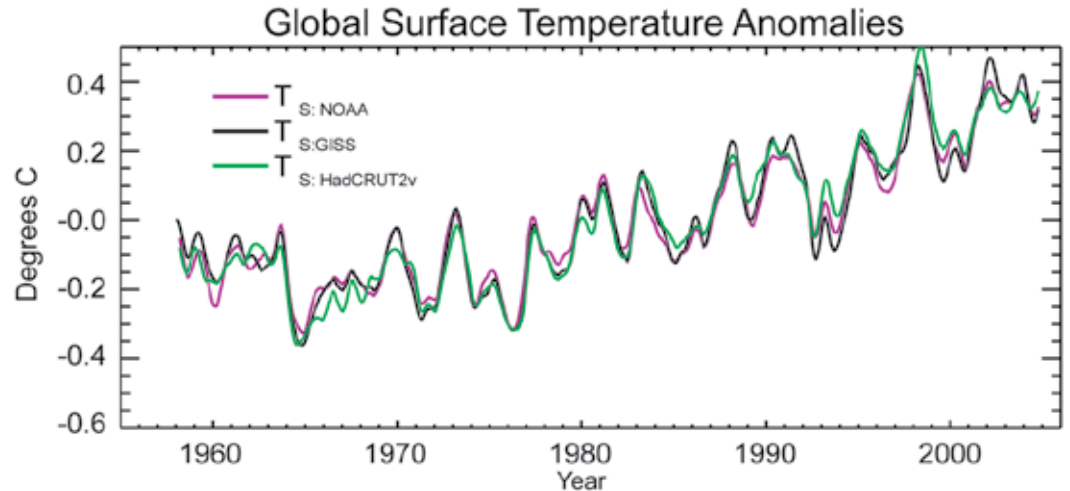
Figure 3.1 - Time series of globally averaged surface temperature ( T_s ) for NOAA (violet), NASA (black), and HadCRUT2v (green) datasets. All time series are 7-month running averages (used as a smoother) of original monthly data, which were expressed as a departure ( ^{\circ}\text{C} ) from the 1979-97 average.
