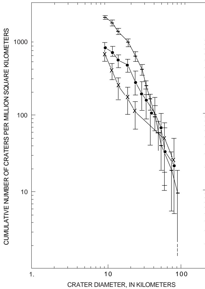
Figure 1. Density distribution of craters on dark materials dark materials (—), on transitional materials formed of slivers and wedges of dark material located in the light terrains (●), and on light materials (X) in the Memphis Facula quadrangle of Ganymede. Error bars denote standard error (\pm N/A)^{1/2} .
