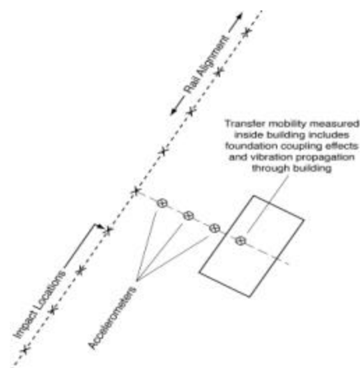
Figure 9.2b Approach 2 for Vibration Propagation Tests
