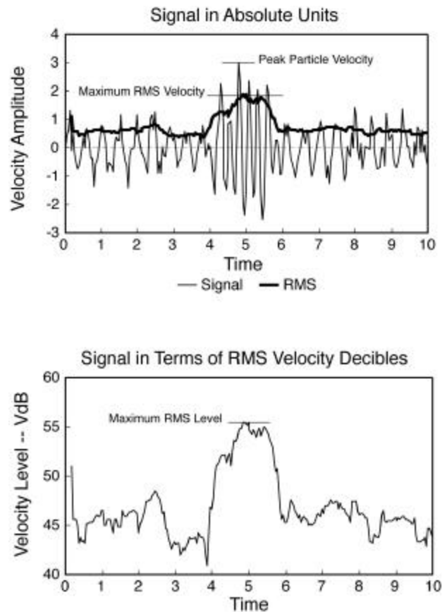
Figure 6-2 Different Methods of Describing a Vibration Signal
