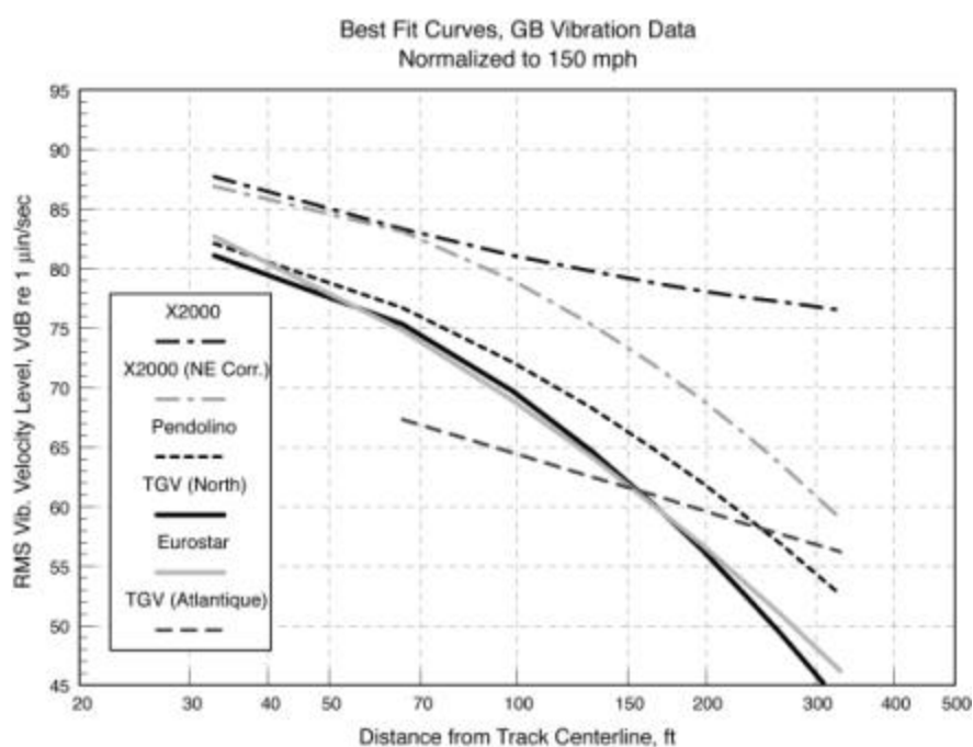
Figure D-2 Best-Fit Curves of Vibration Velocity Level vs. Distance
