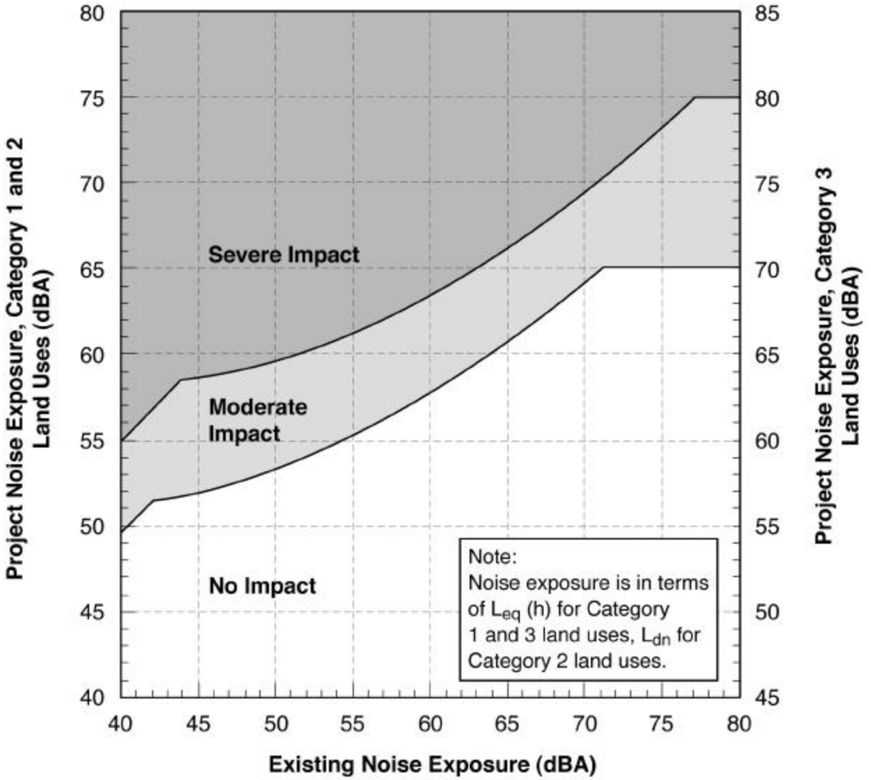
Figure 3-1 Noise Impact Criteria for High Speed Rail Projects
