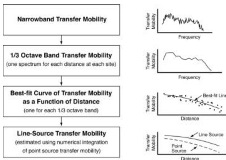
Figure 9-4 Analysis of Transfer Mobility
