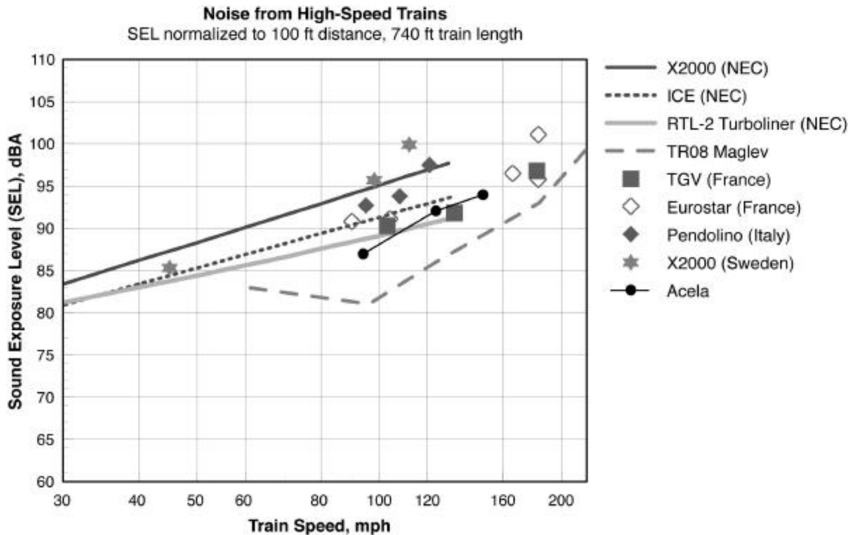
Figure 2-14 Measured Values of SEL vs Speed from High-Speed Trains
