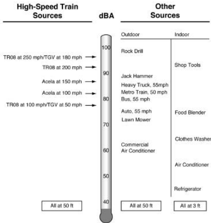
Figure 2-2 Typical A-Weighted Sound Levels
