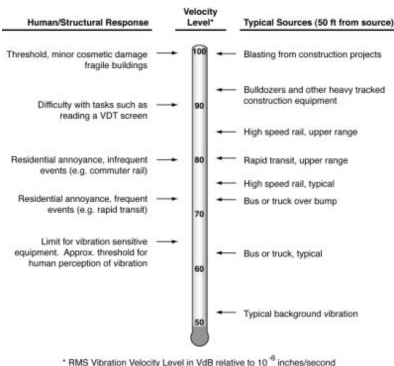
Figure 6-3 Typical Levels of Ground-Borne Vibration
