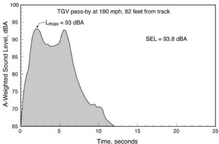
Figure 2-3 Typical High-Speed Train Passby
