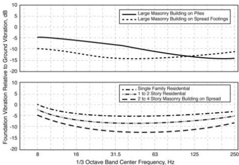
Figure 9-7 Approximate Foundation Response for Various Types of Buildings (Ref. 50)
