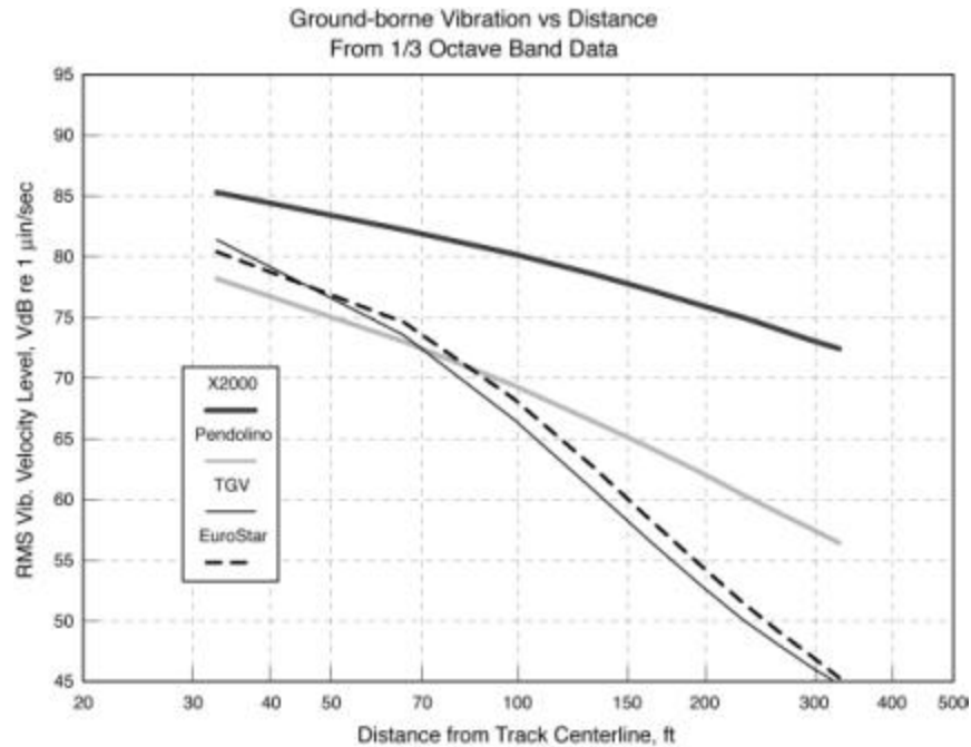
Figure D-3 Vibration Velocity vs. Distance Calculated from Smoothed 1/3 Octave Bands
