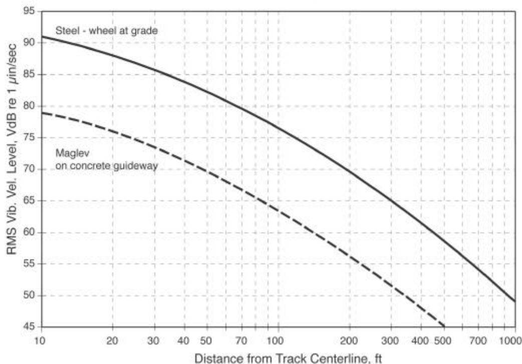
Figure 8-1 Generalized Ground-Borne Vibration Curve
