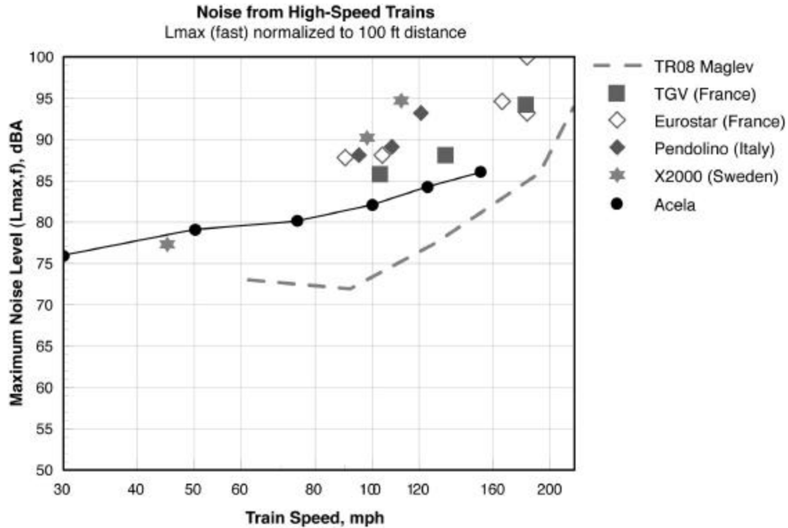
Figure 2-13 Measured Values of L max,s vs Speed from High-Speed Trains
