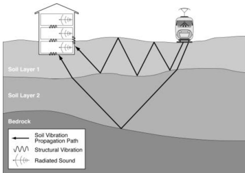
Figure 6-1 Propagation of Ground-Borne Vibrations into Buildings
