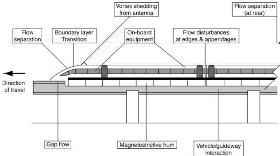
Figure 2-9 Noise Sources on a Maglev System
