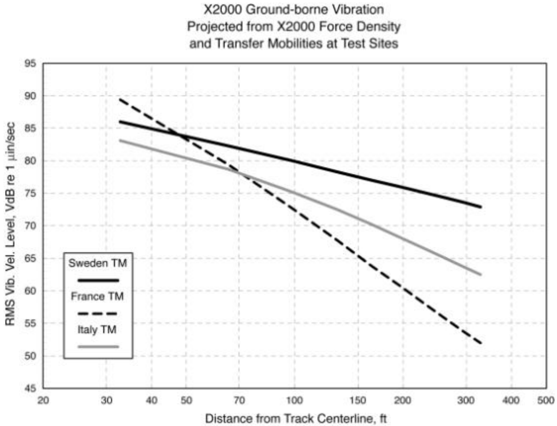
Figure D-9 Projected Vibration Velocity, X2000 Force Density
