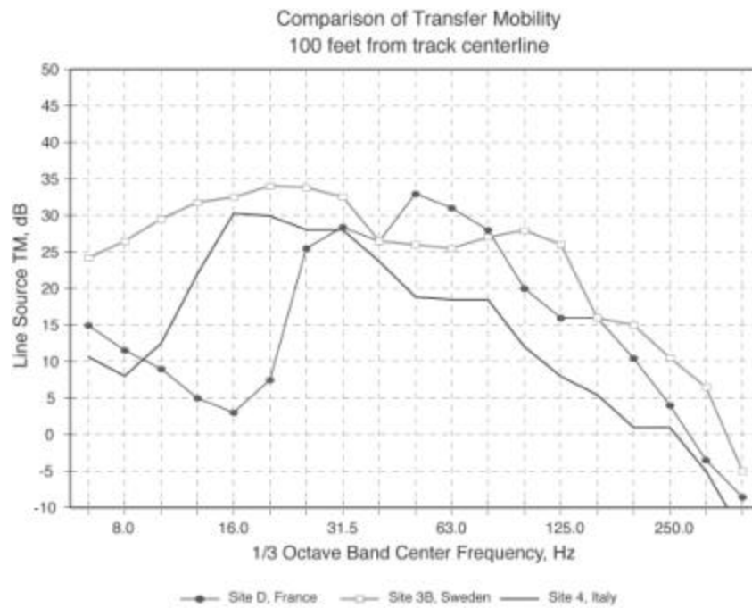
Figure D-5 Line-Source Transfer Mobility at the Test Sites
