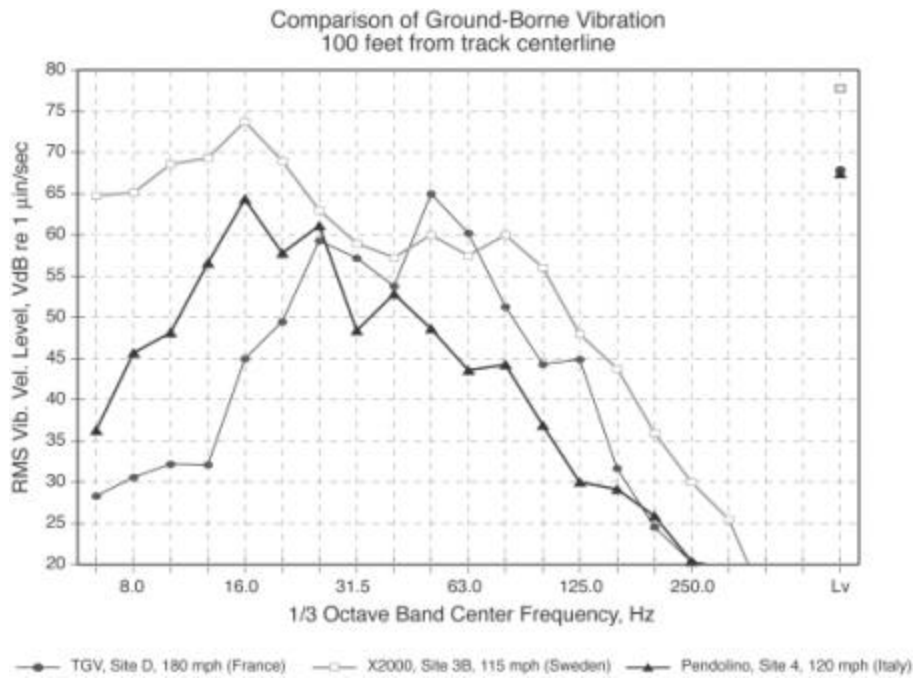
Figure D-4 Comparison of 1/3 Octave Band Spectra
