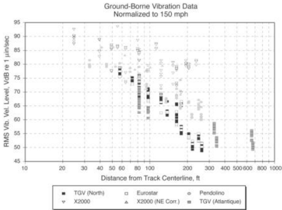
Figure D-1 Overall Vibration Velocity Level for Different High Speed Trains
