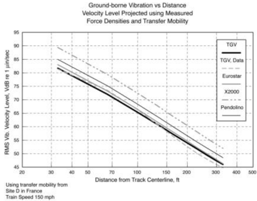
Figure D-7 Projected Vibration Velocity, Transfer Mobility from Site in France
