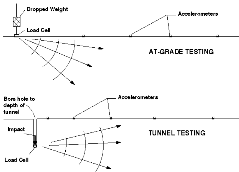
Figure 9-1 Impact Method for Measuring Transfer Mobility
