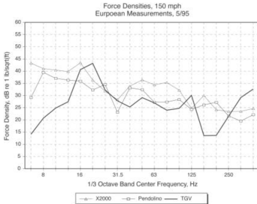
Figure D-6 Force Density Functions Derived from Measurements
