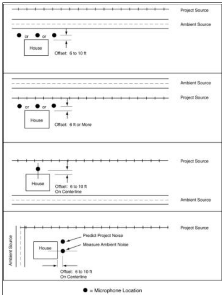
Figure 5-2 Recommended Microphone Locations for Existing Noise Measurements
