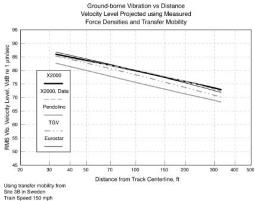
Figure D-8 Projected Vibration Velocity, Transfer Mobility from Site in Sweden
