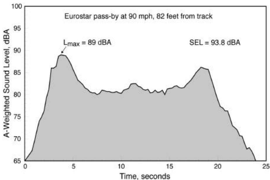
Figure 2-4 Typical Longer-Duration High-Speed Train Event
