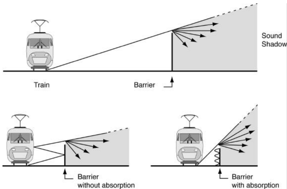
Figure 2-12 Noise Barrier Geometry
