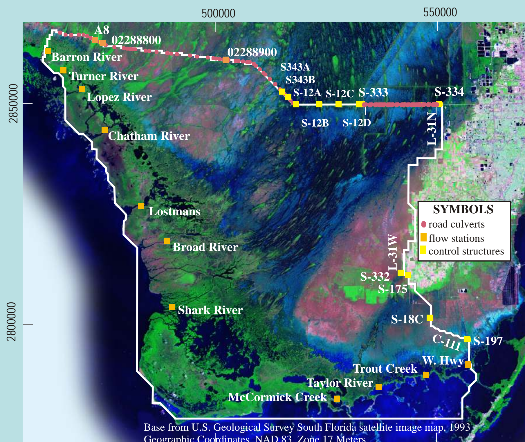
Figure 7. Locations of road culverts, flow stations, and hydraulic control structures in the TIME model domain.
