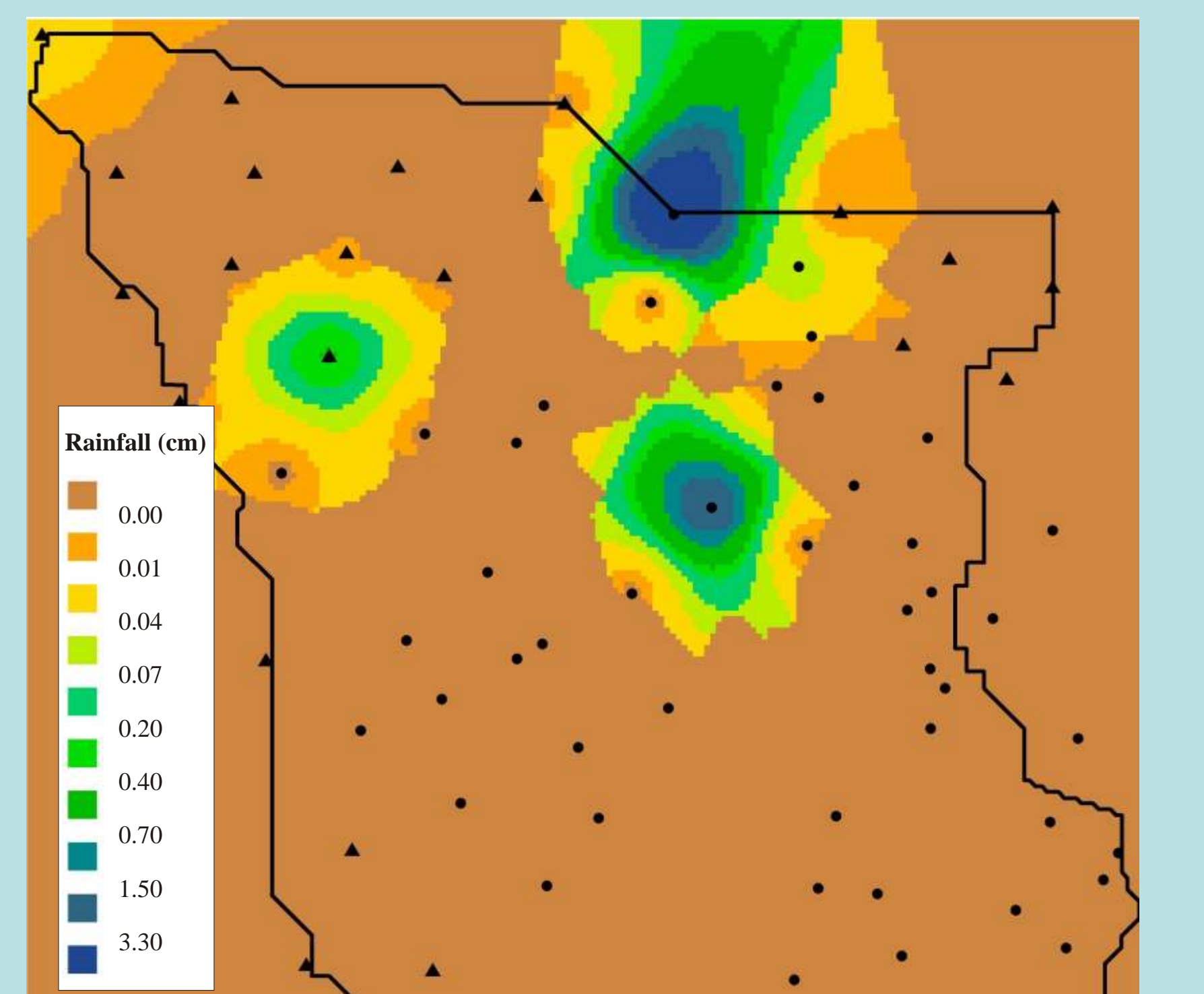
Figure 10. Rainfall on June 16, 1999, between 1500 and 1600 hours in 500-m-square TIME grid resolution.
