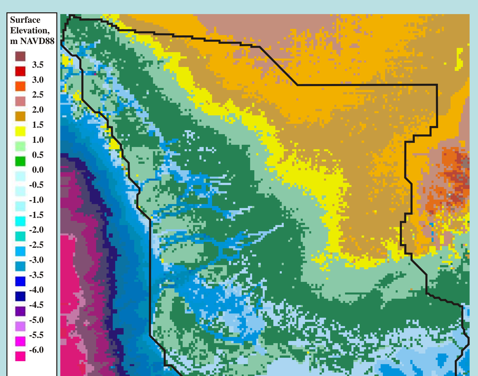
Figure 3. Land-surface elevations.
