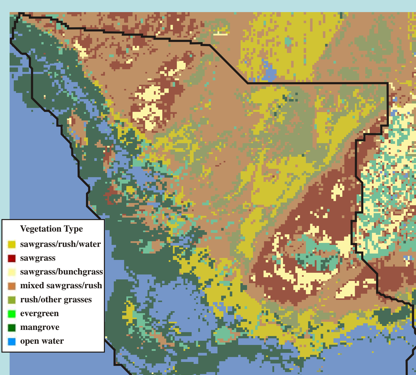
Figure 4. Vegetation types.
