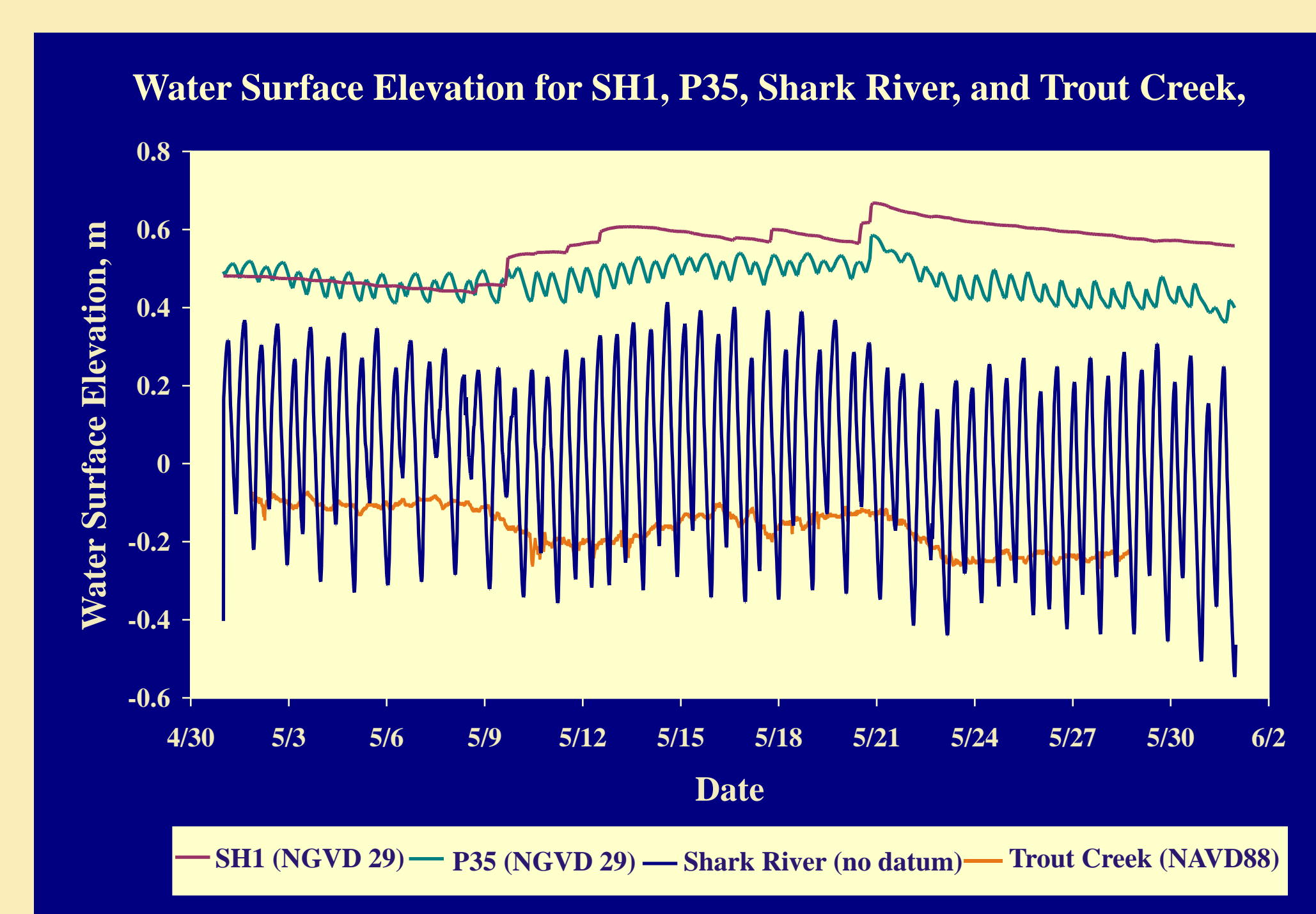
Figure 2. Water-level data recorded in Shark River (SR), Shark River Slough (P35 and SH1), and Trout Creek, a tributary to Florida Bay.
