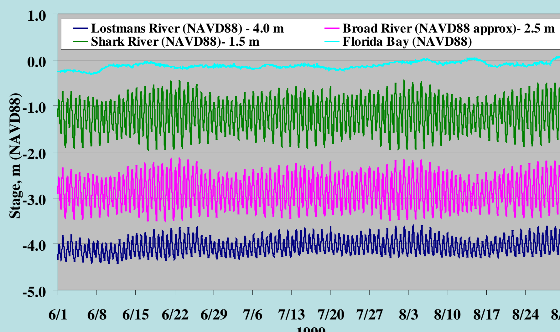
Figure 9. Water-surface elevations specified as open boundary conditions.
