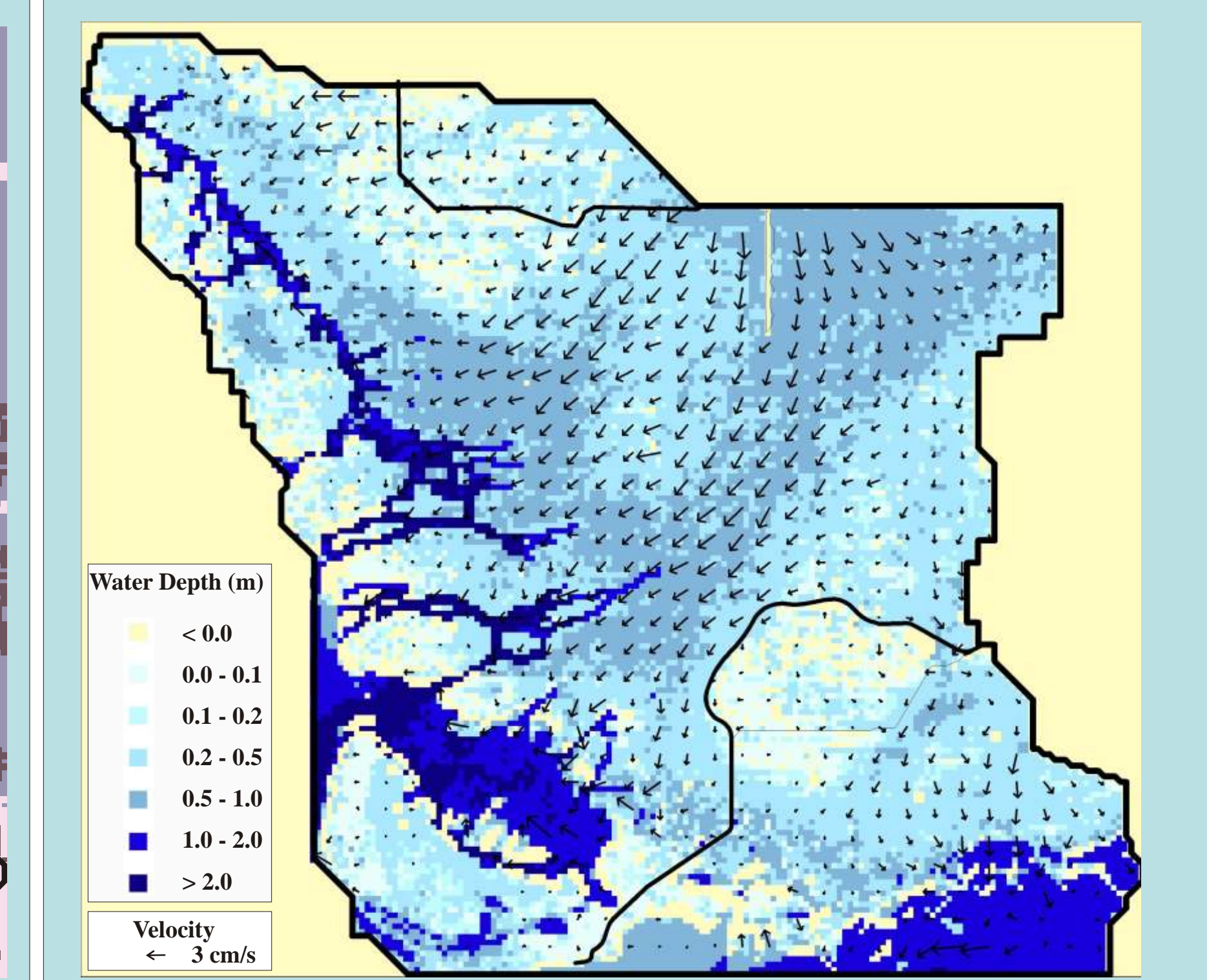
Figure 13. Preliminary simulated flow depths and velocities at midnight on August 31, 1999.
