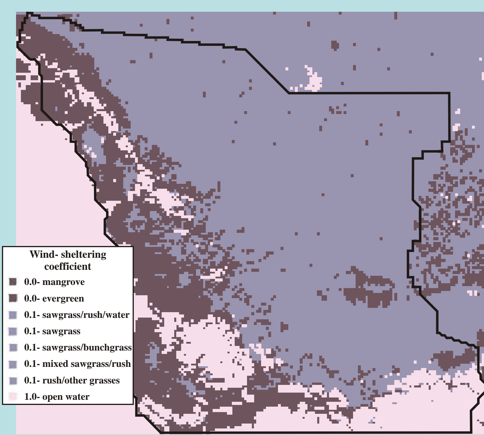
Figure 6. Wind-sheltering coefficients.
