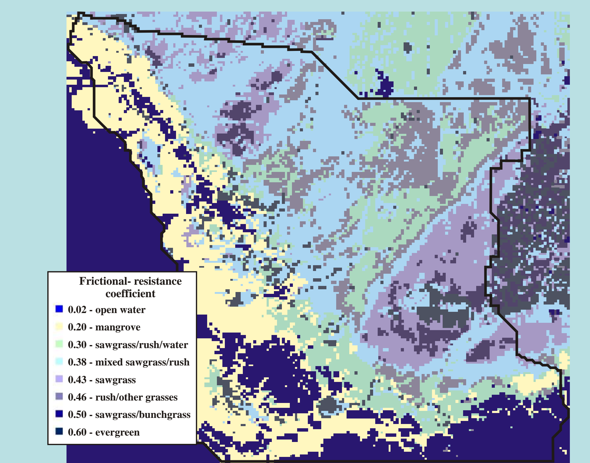
Figure 5. Frictional-resistance coefficients.
