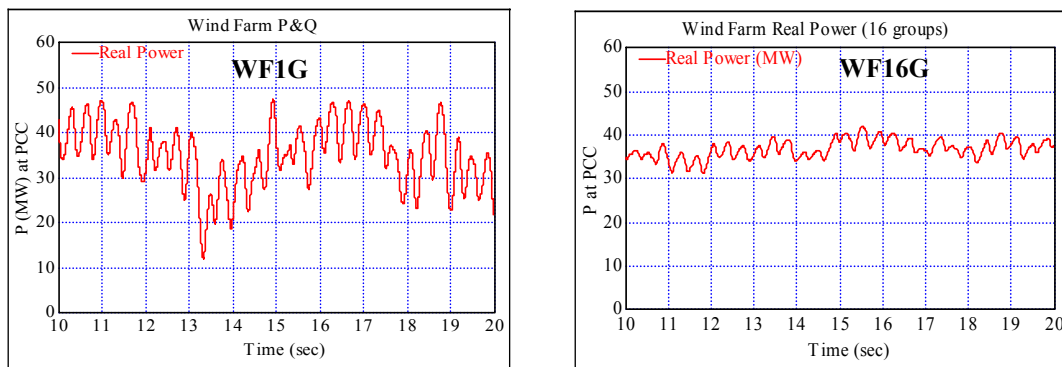
Fig. 3. Real power output of a wind farm in a WF1G and in a WF16G.
