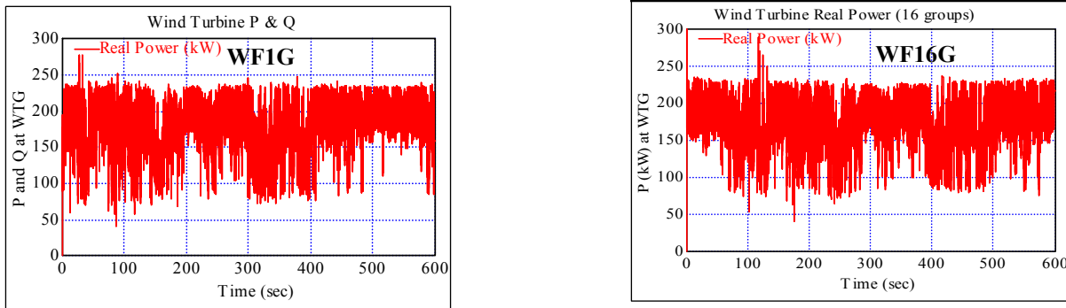
Fig. 2. Real power output of a turbine in a WF1G and in a WF16G.
