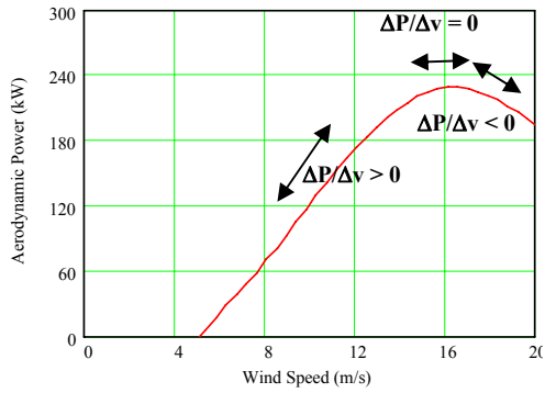
Fig.6. A typical power curve of a wind turbine generator
